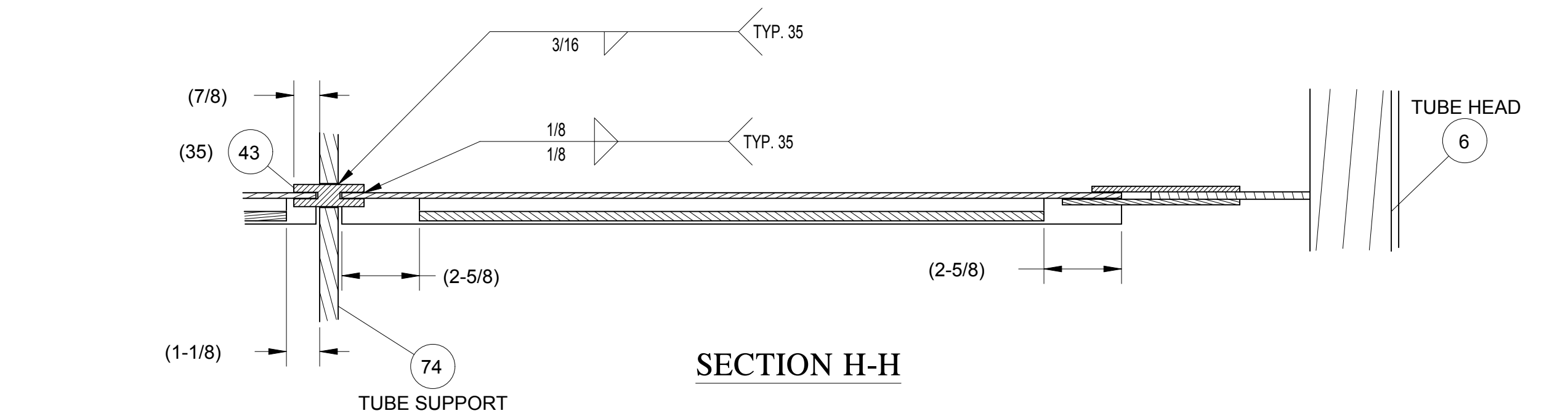
TUBE SUPPORT
