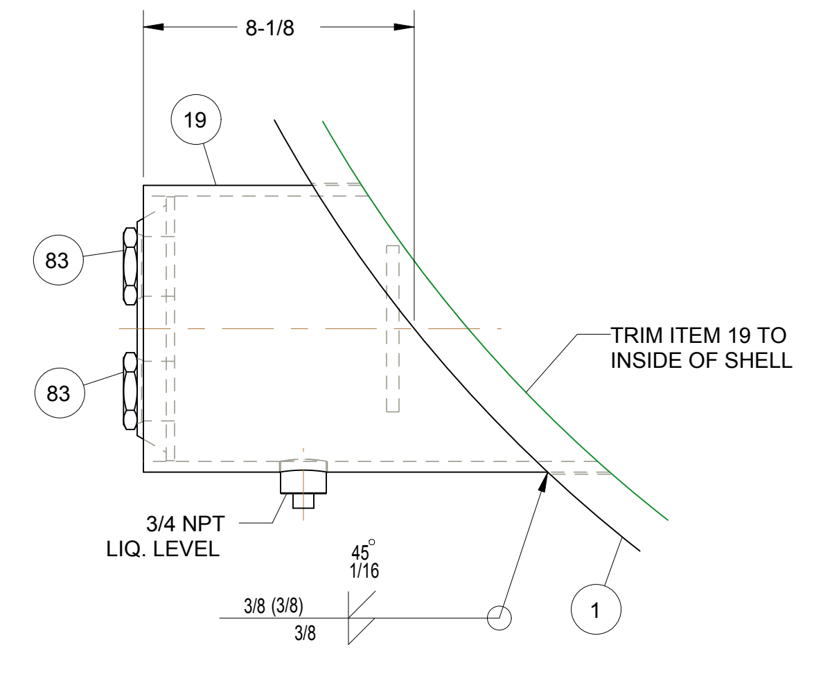
DETAIL M
