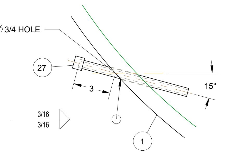
DETAIL N
