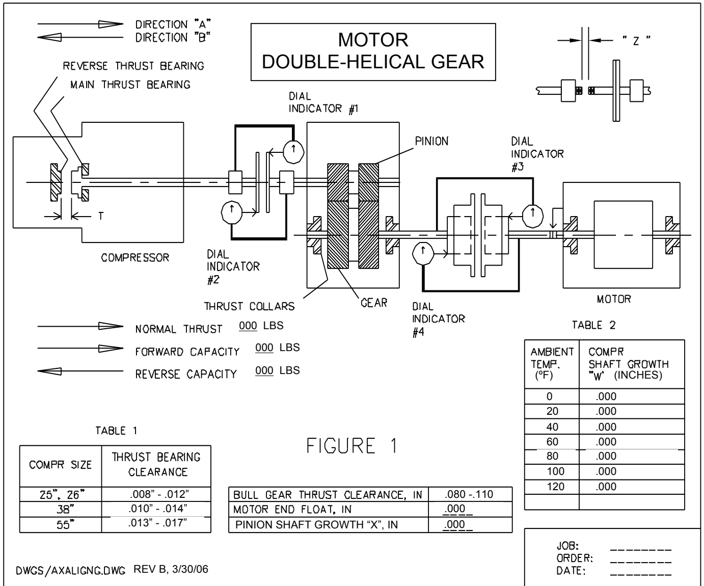
Axial Alignment Drawing
