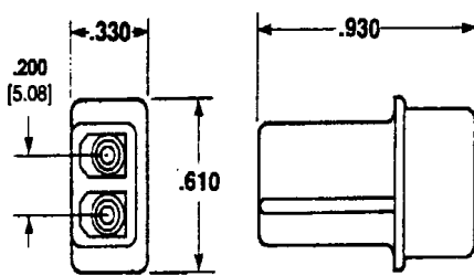
2 Circuit In-Line Pin Housing
