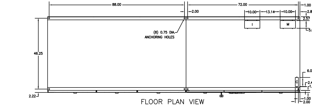
FLOOR PLAN VIEW
