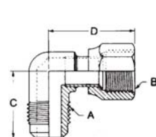
Ext FI to Int FI Swivel
