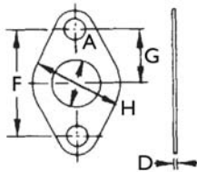
2 Bolt Gasket, Asbestos-Free
