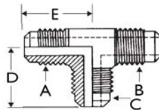
Three-Way
