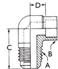
Half Union - Flare to Solder
