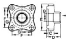
4 Bolt, Flat, Tongue, Groove Diameters 2 3/4" x 2 3/16"
