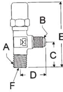
NPTF Inlet to Flare
