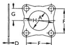
4 Bolt Gasket, Asbestos-Free
