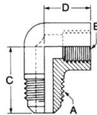
External Flare to NPTFI
