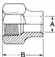
Long Forged Nuts
