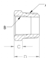
Bushing NPT to NPTFI
