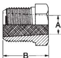
Fusible Pipe Plugs - NPTFE
