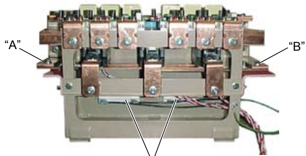
1RES and 2RES Bus Capacitors Bank Equalizing / Bleeder Resistors
