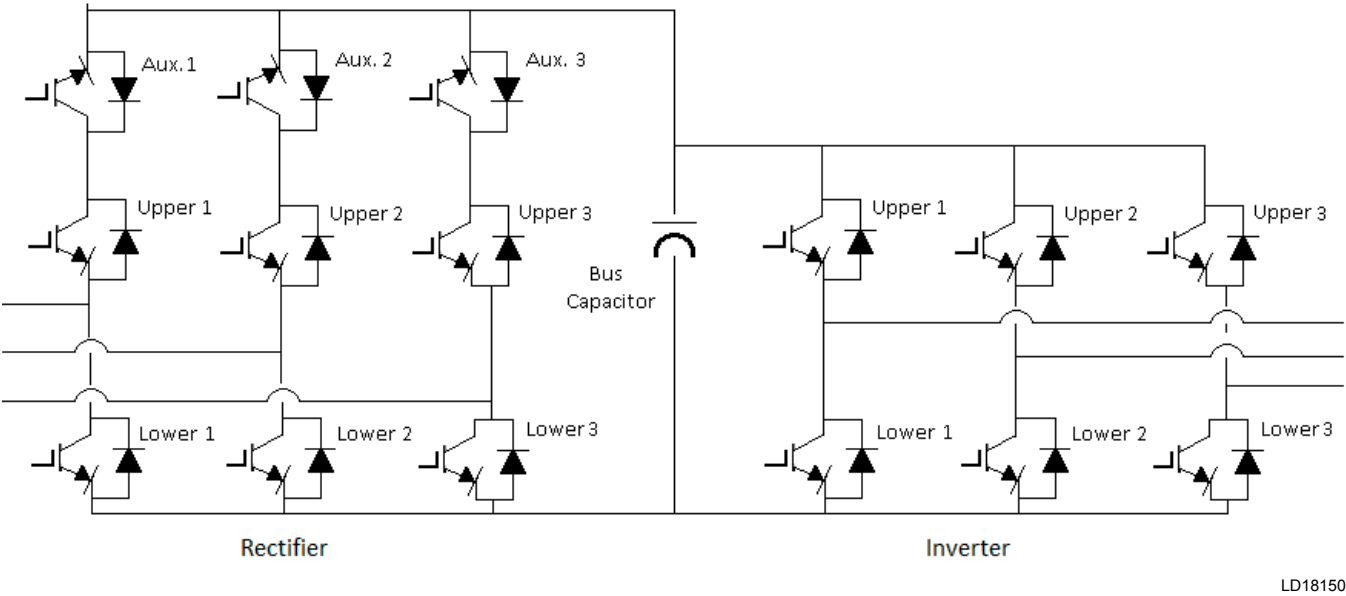
FIGURE 13 - HYP MODEL POWER CIRCUIT
