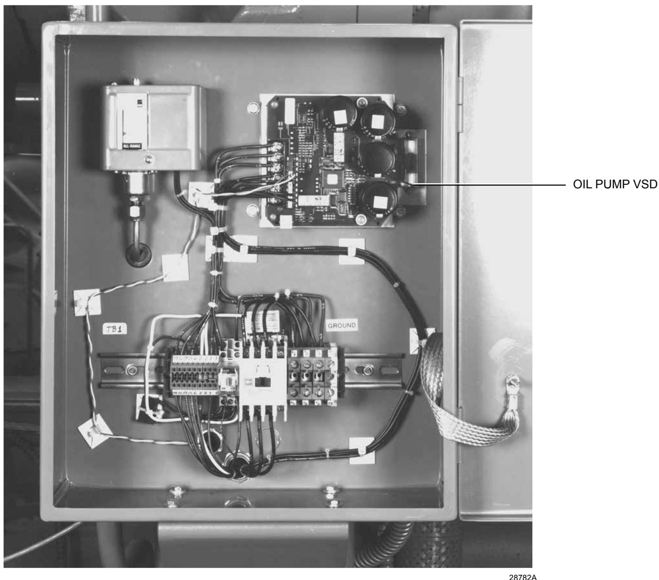
FIGURE 74 - OIL PUMP VARIABLE SPEED DRIVE (VSD)
