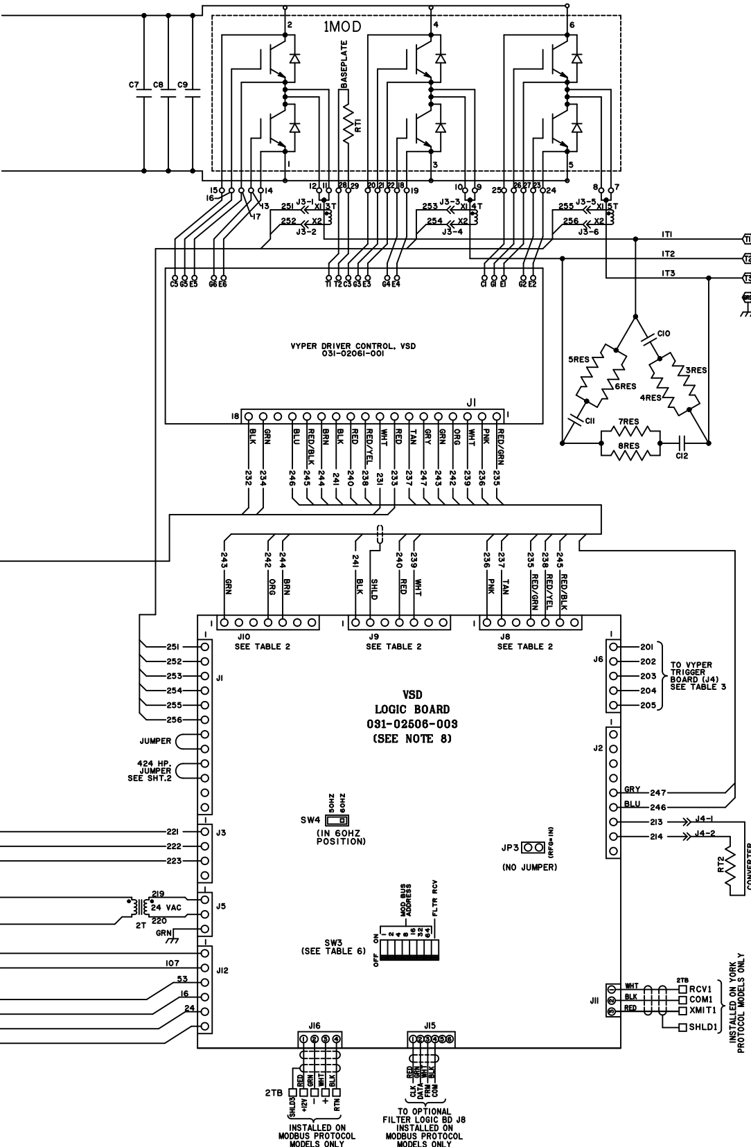
FIGURE 3 - ELEMENTARY WIRING DIAGRAM 424 HP ON UNITS MANUFACTURED AFTER DECEMBER 2006 (CONT'D)
