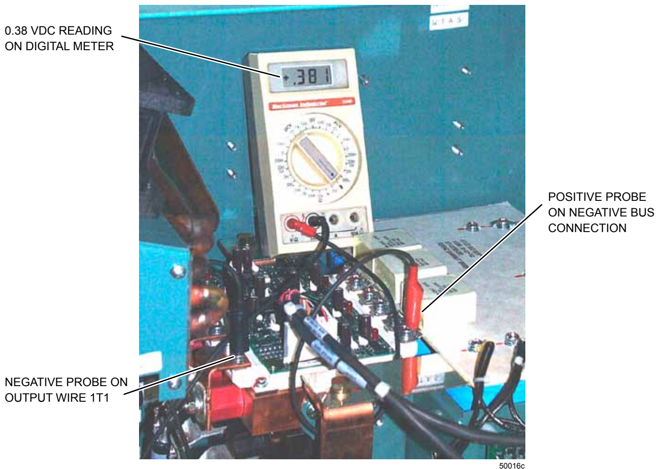
FIGURE 23 - 270/292/351/424 HP DRIVE IGBT MODULE VERIFICATION #1
