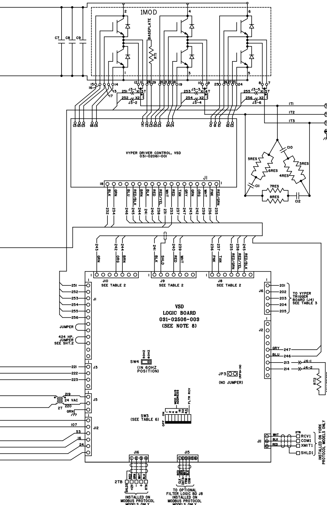
FIGURE 4 - ELEMENTARY WIRING DIAGRAM 424 HP ON UNITS MANUFACTURED BEFORE DECEMBER 2006 (CONT'D)
