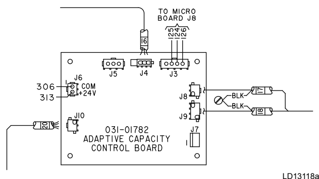
FIGURE 21 - ADAPTIVE CAPACITY CONTROL BOARD FOR OPTIVIEW CONTROL CENTER
