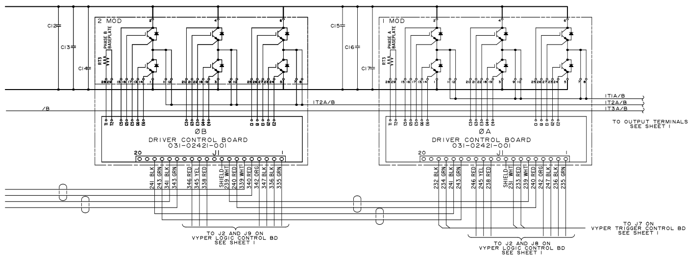
FIG. 5 (CONT'D)– POWER ASSEMBLY ELEMENTARY WIRING DIAGRAM 419/503 HP
