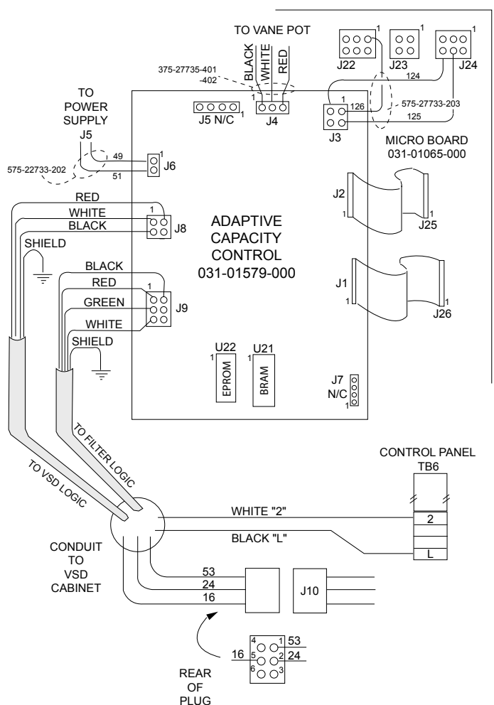
FIG. 13 – ADAPTIVE CAPACITY CONTROL BOARD
