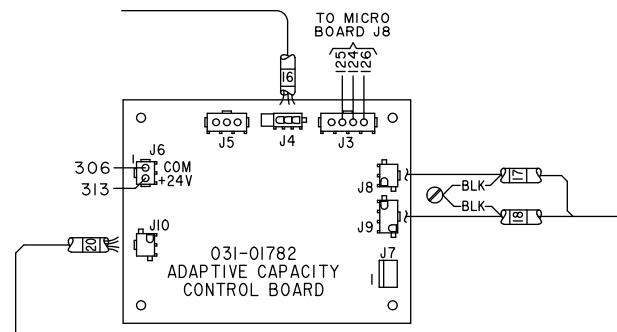
FIG. 12 – ADAPTIVE CAPACITY CONTROL BOARD FOR OPTIVIEW CONTROL CENTER
