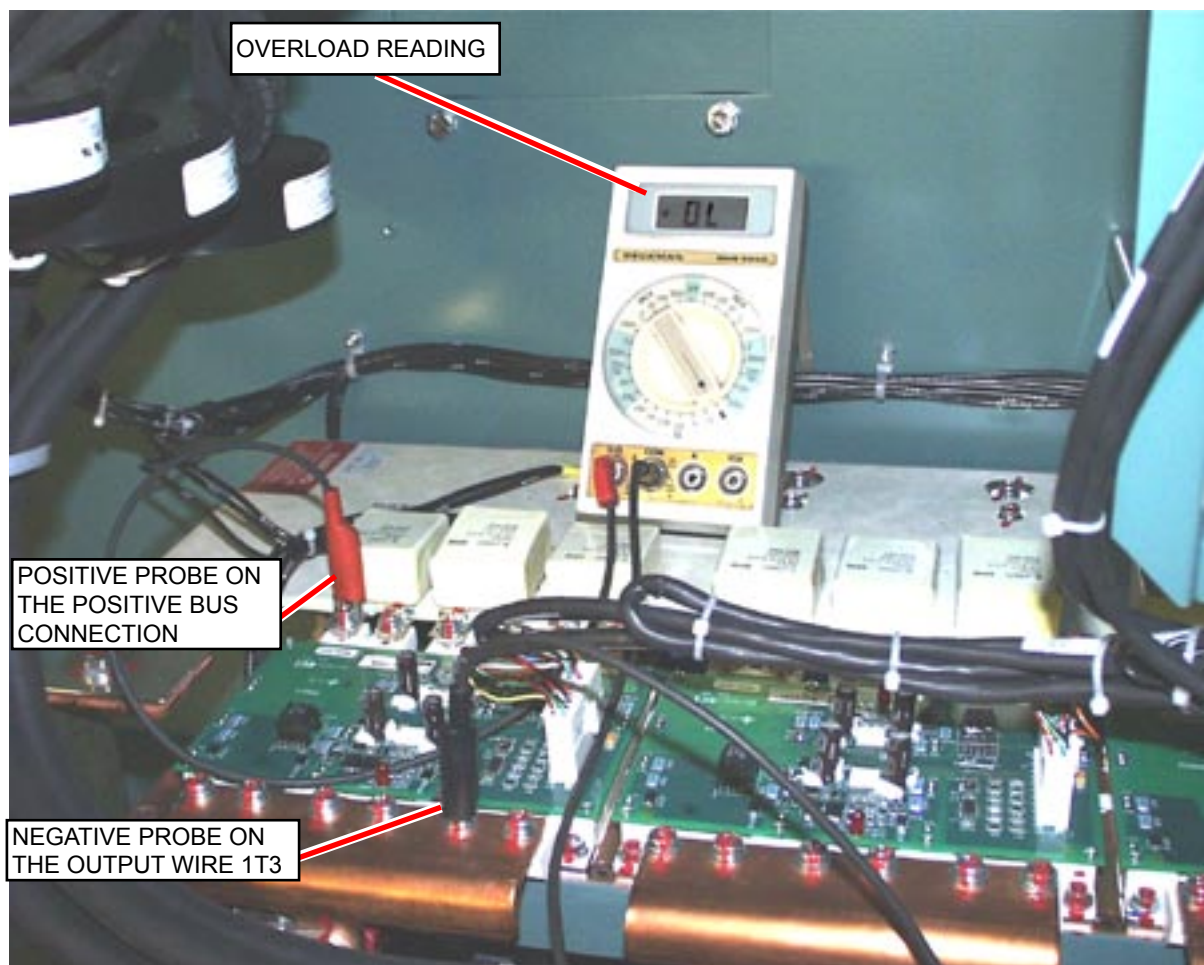
FIG 17 - 419/503/608 HP DRIVE IGBT MODULE VERIFICATION #1
