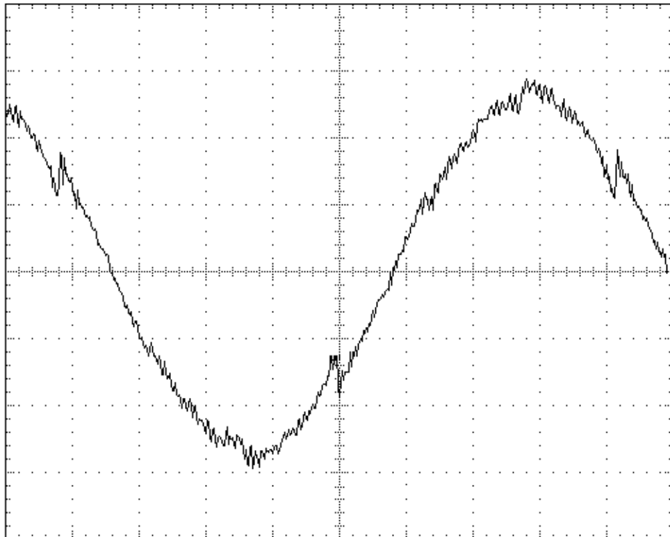
FIG. 7B – VSD INPUT CURRENT WITH FILTER
