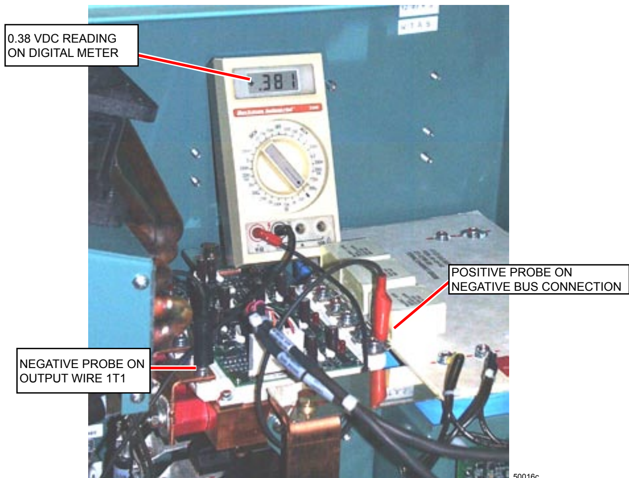
FIG. 14 - 292/351/424 HP DRIVE IGBT MODULE VERIFICATION #1
