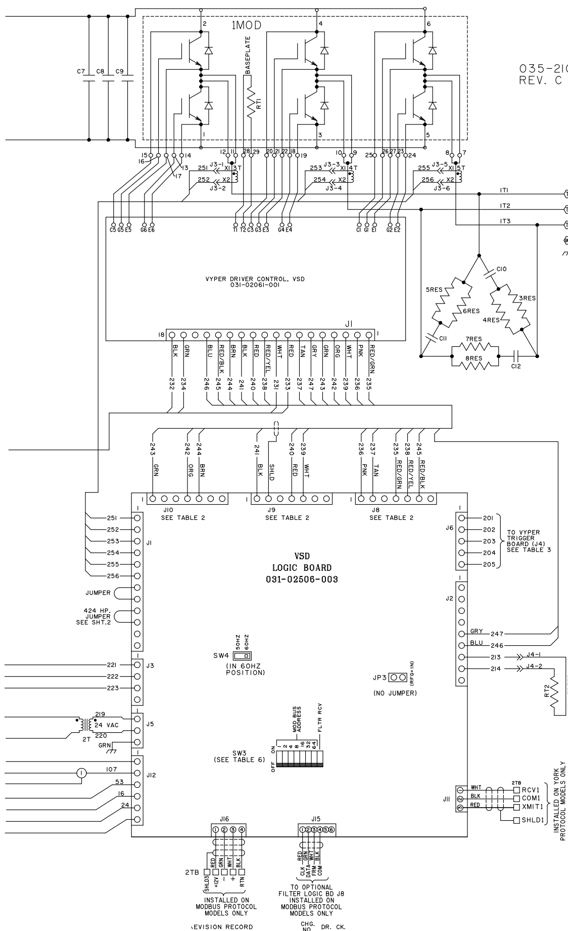
FIG. 2 (CONT'D) - ELEMENTARY WIRING DIAGRAM 424 HP
