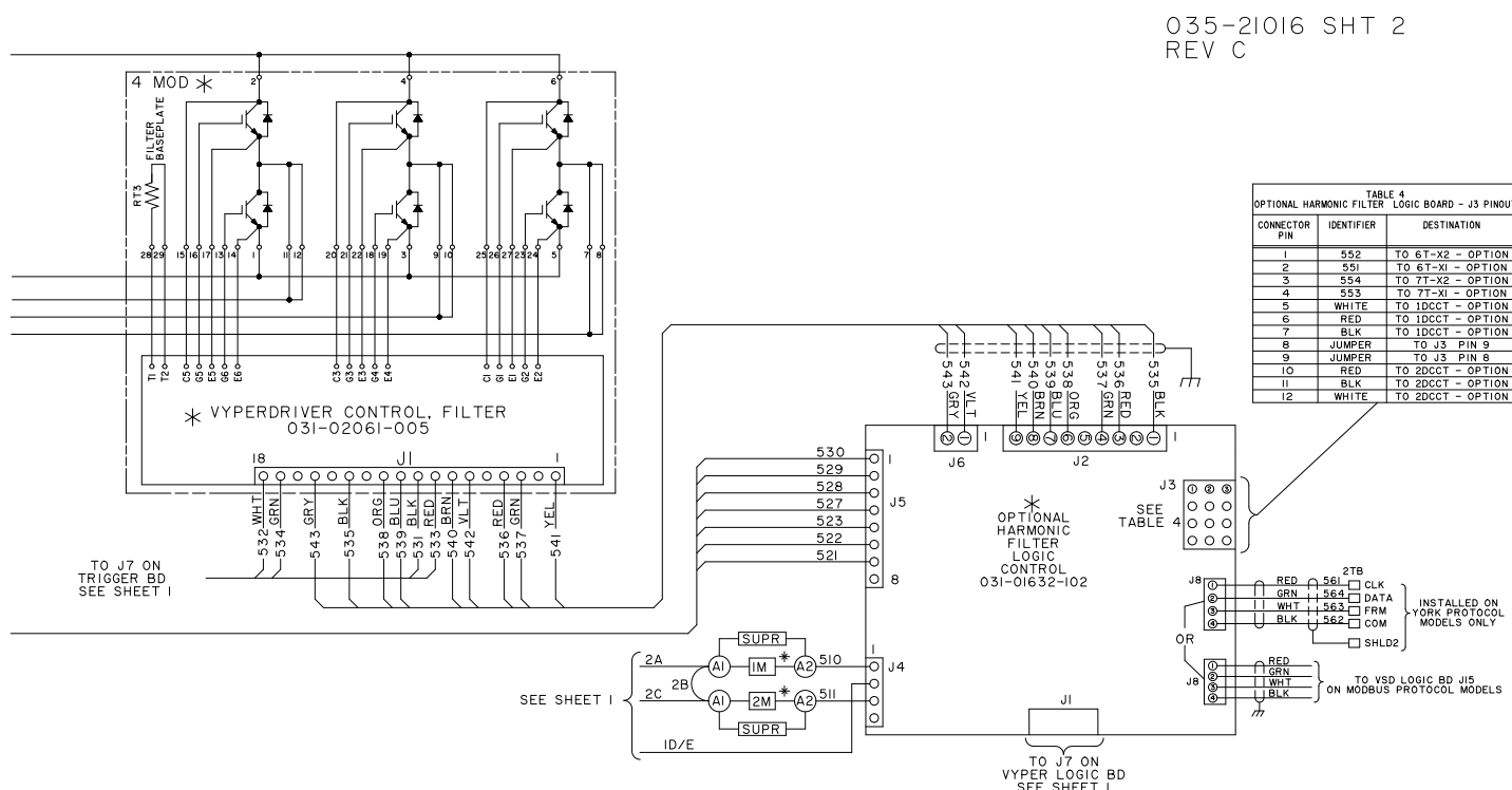
FIG. 11 (CONT'D)– HARMONIC FILTER WIRING DIAGRAM 608 HP
