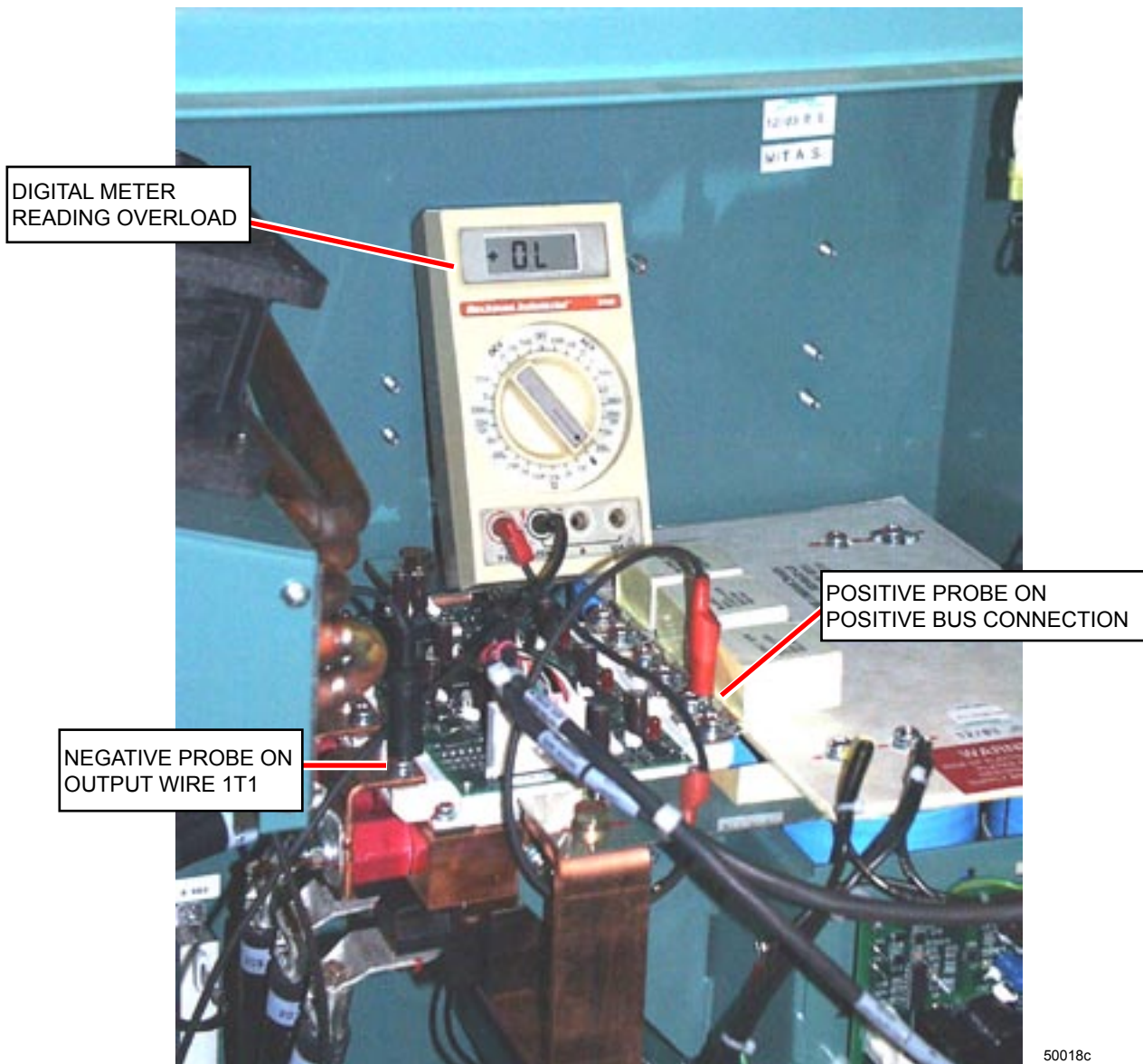
FIG. 16 - 292/352/424 HP DRIVE IGBT MODULE VERIFICATION #3.
