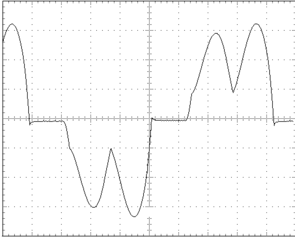
FIG. 7A – VSD INPUT CURRENT WITHOUT FILTER
