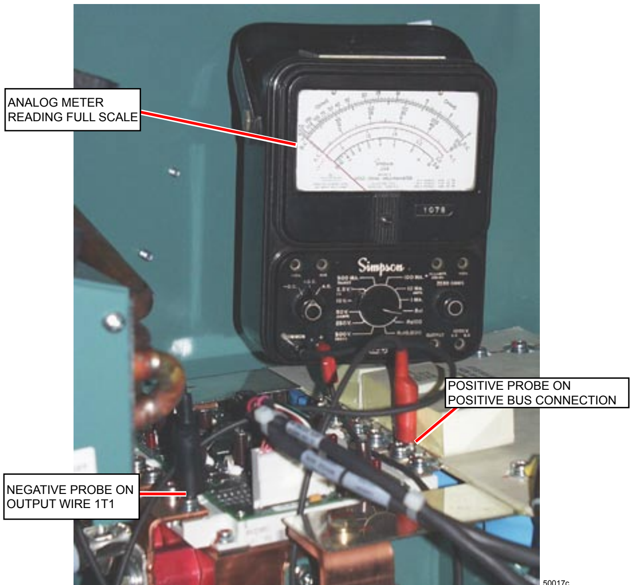
FIG. 15 - 292/351/424 HP DRIVE IGBT MODULE VERIFICATION #2.
