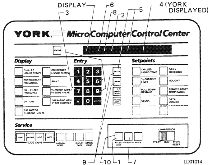
FIG. 3 – KEYPAD – PROGRAMMING SYSTEM SETPOINTS
