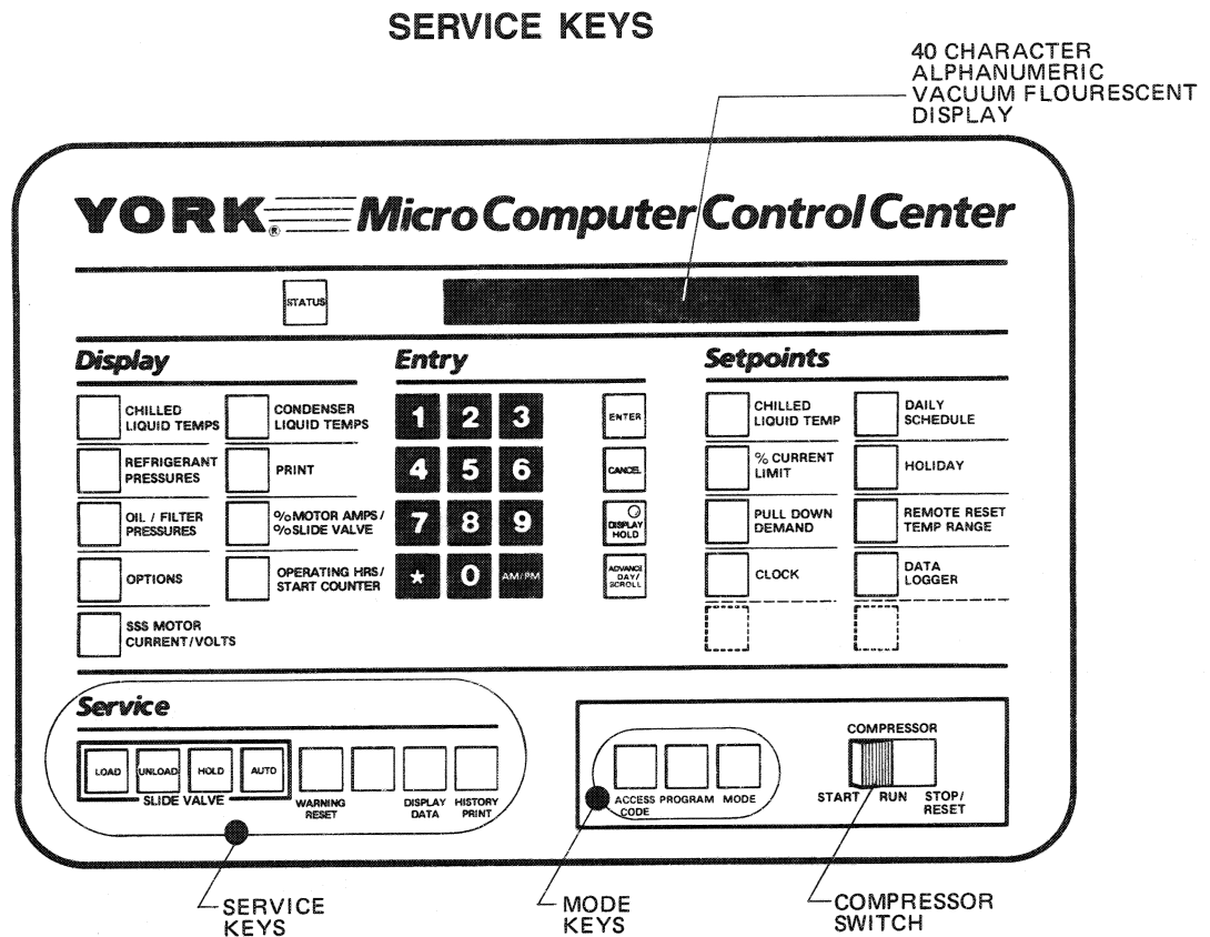
FIG. 12 – KEYPAD – SERVICE KEYS LOCATION
