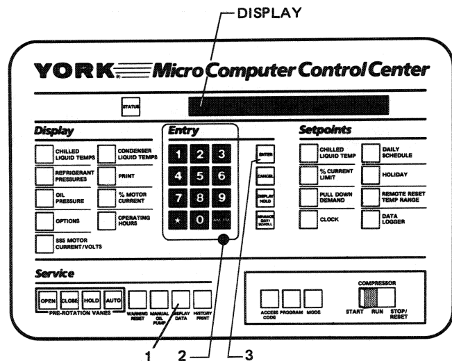
FIG. 11 – KEYPAD - PROGRAMMING "EXCESS PURGE THRESHOLD"
