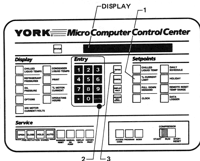
FIG. 5 – KEYPAD – PROGRAMMING “% CURRENT LIMIT” SETPOINT
