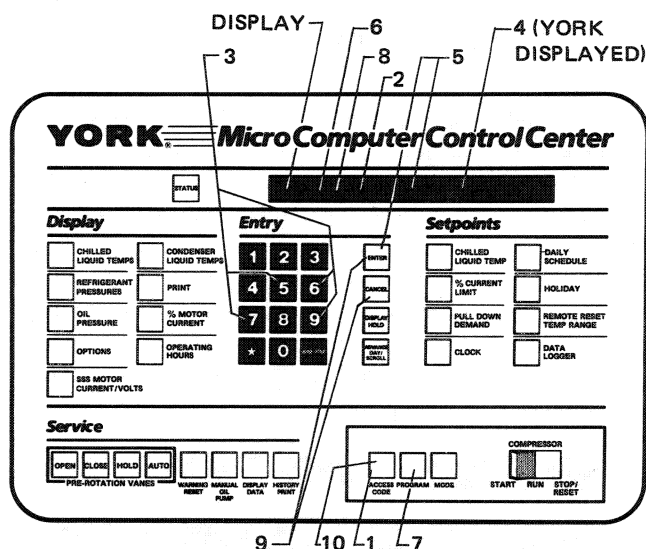
FIG. 3 - KEYPAD — PROGRAMMING SYSTEM SETPOINTS
