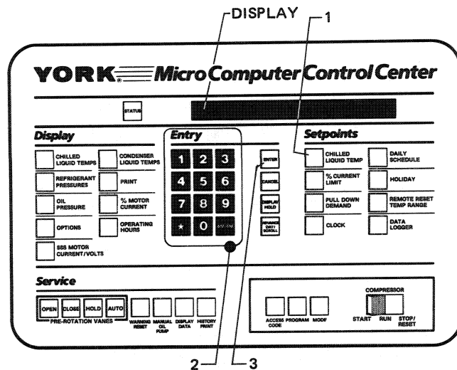
FIG. 4 – KEYPAD — PROGRAMMING “LEAVING CHILLED WATER TEMP.” SETPOINT
