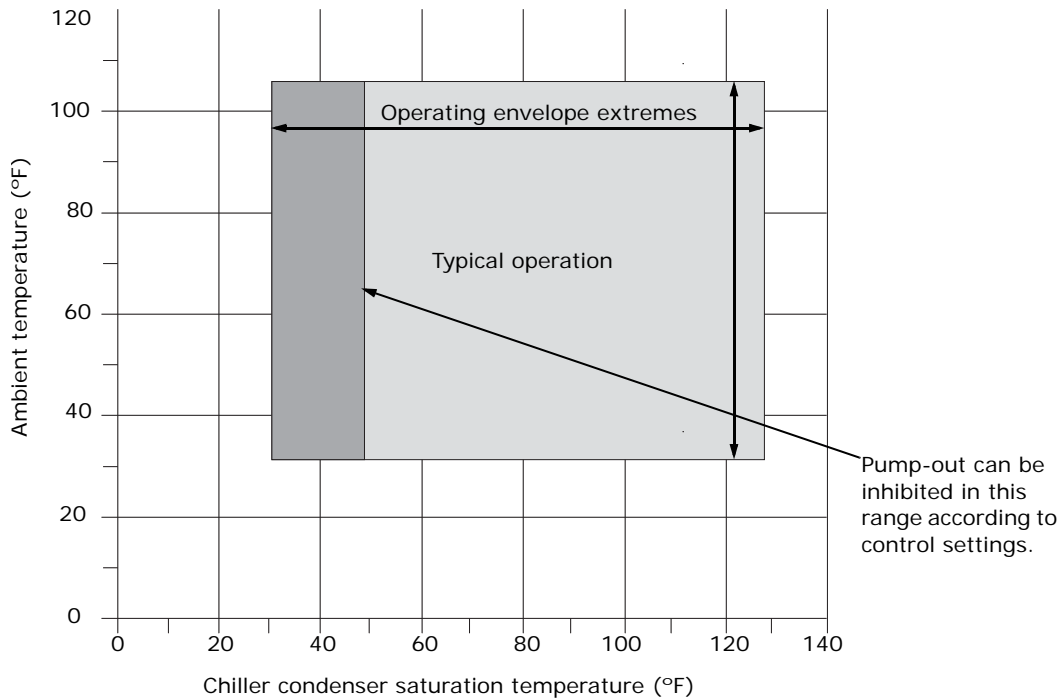
Figure 6. EarthWise purge operating limits
