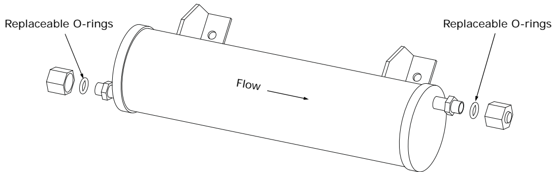
Figure 11. Filter-drier assembly
