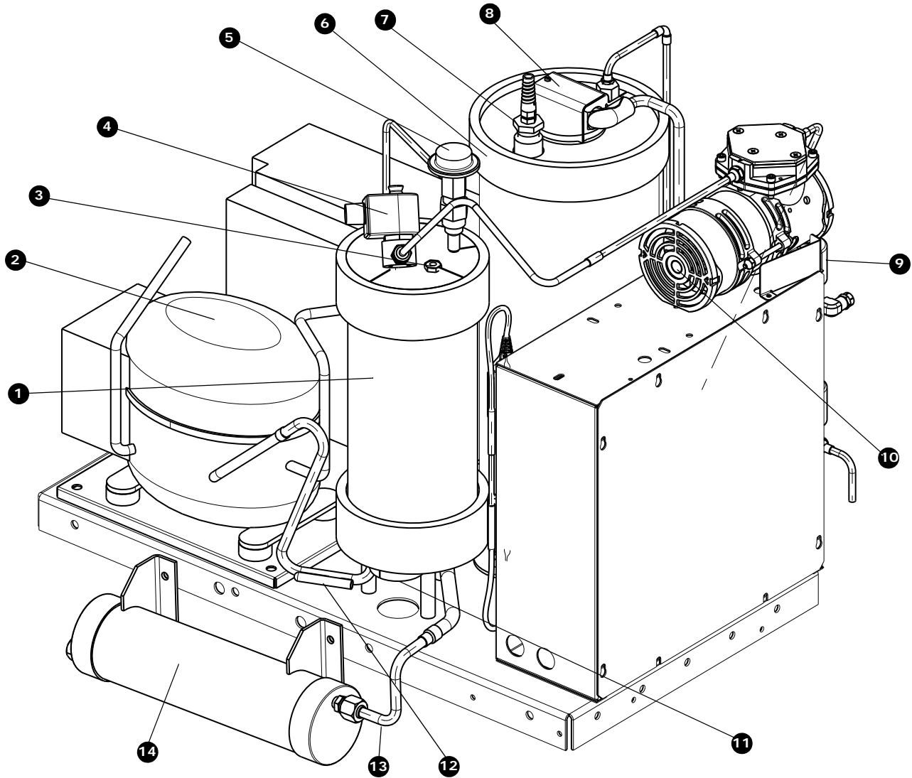
Figure 1. Components of a Trane EarthWise purge system (front view)
