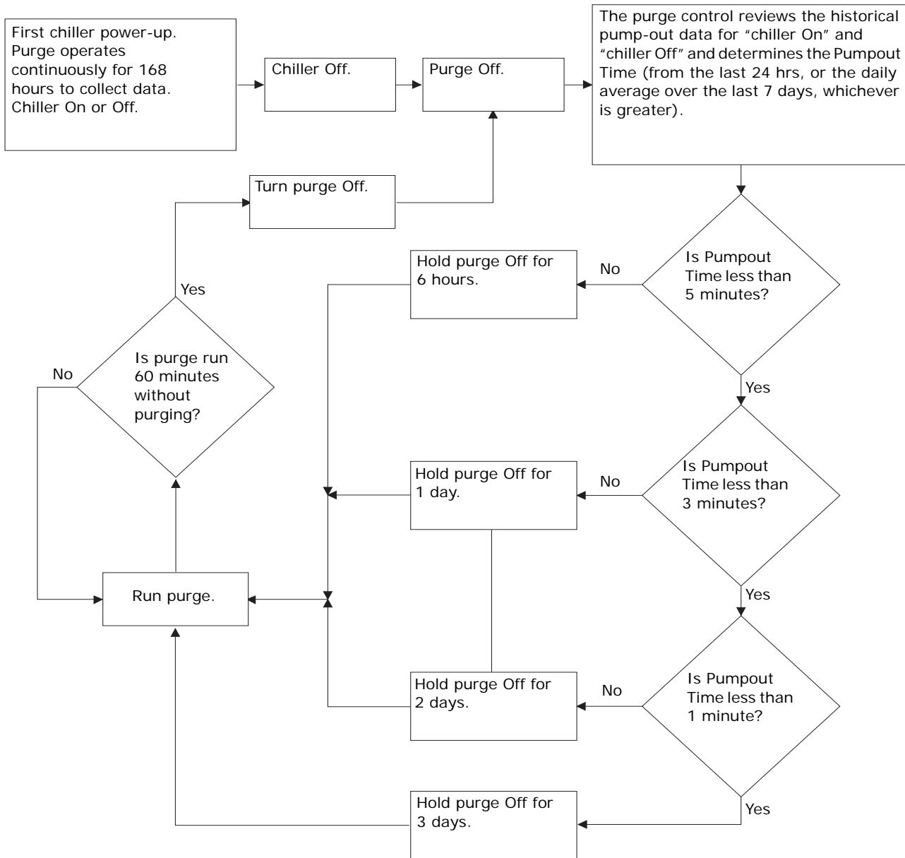
Figure 4. Adaptive chiller OFF flow chart
