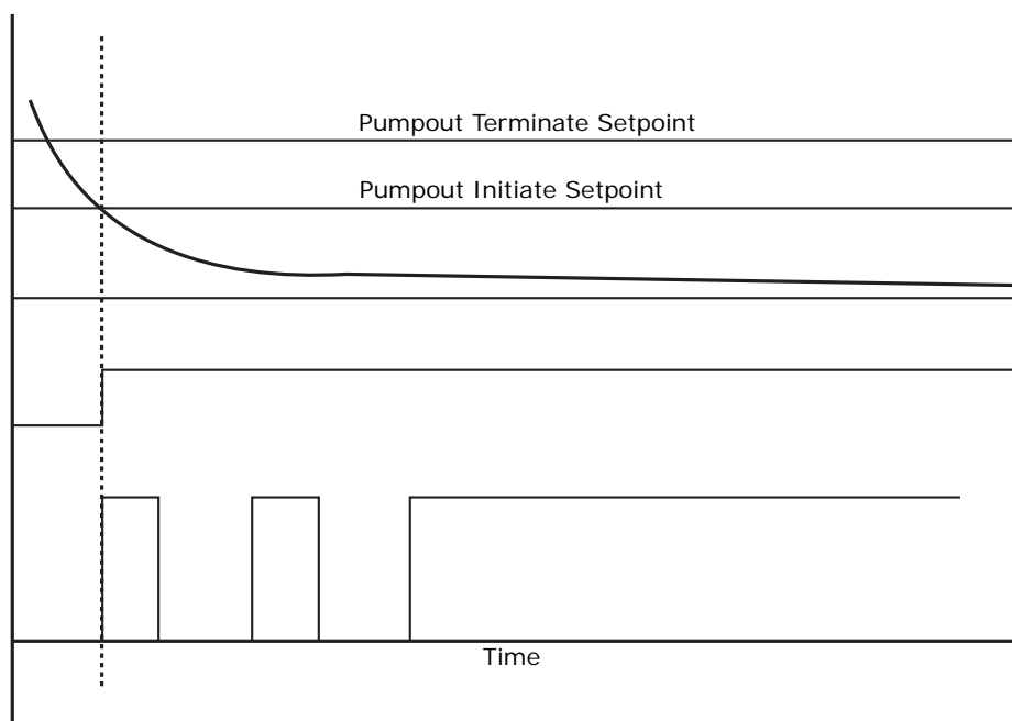
Figure 8. Non-condensable pump-out cycle, large quantity of air
