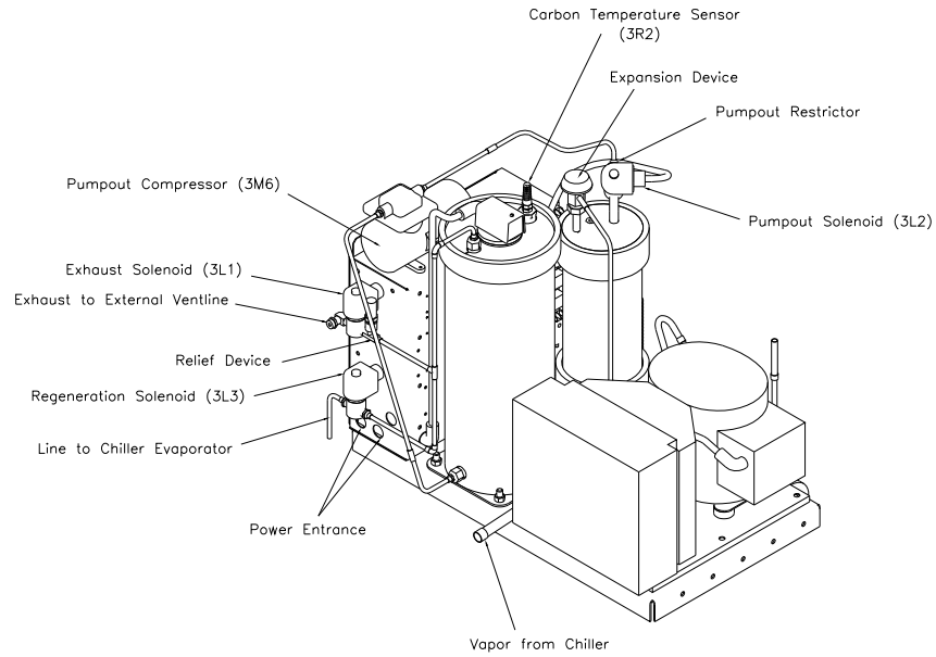
Figure 4. Typical EarthWise Purge component list
