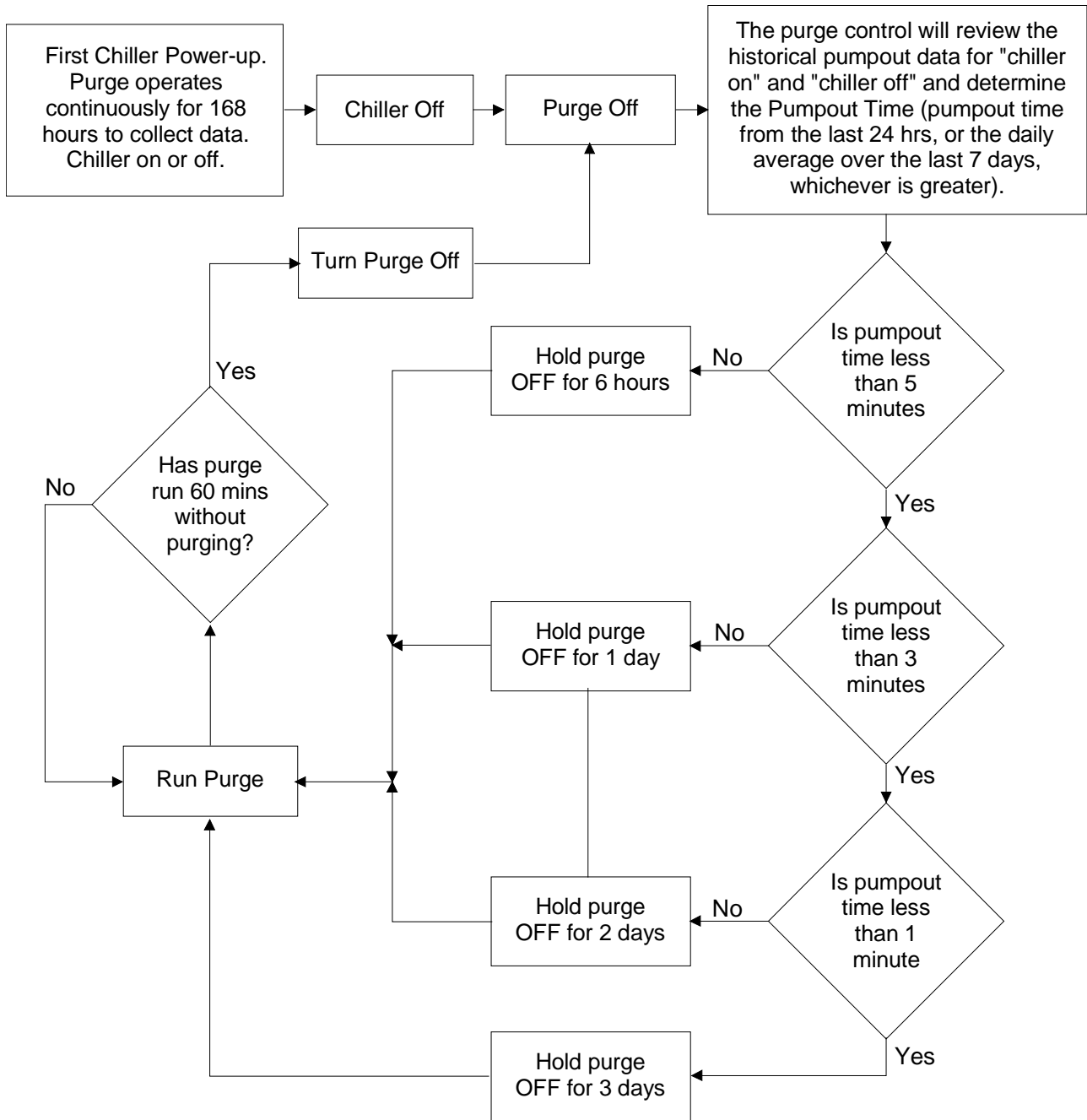
Figure 9. Adaptive chiller OFF flow chart
