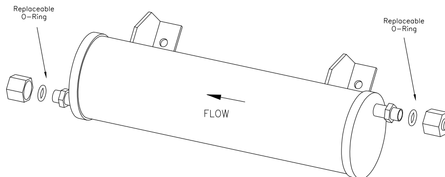
Figure 18. Filter-drier
