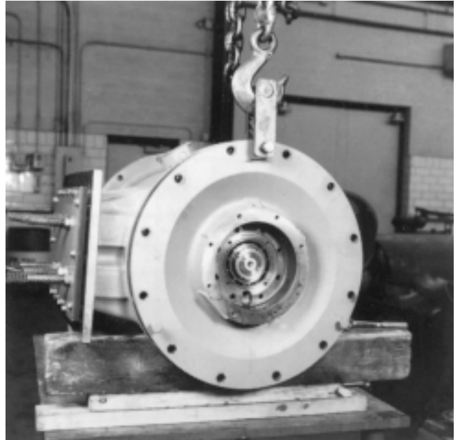
Figure 8. Removing bearing bracket (opposite drive end)
