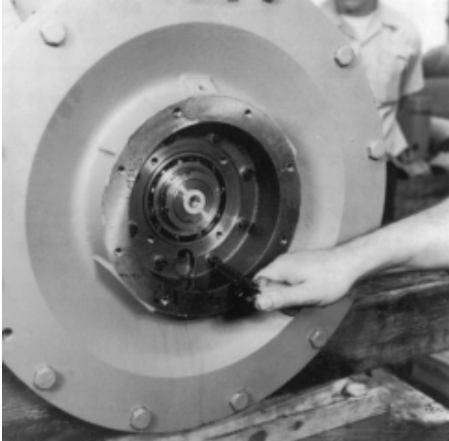
Figure 7. Removing bearing retaining screws
