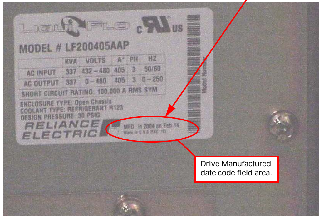
Figure 2. LF 2 Labeling as shown on inside Power module.
