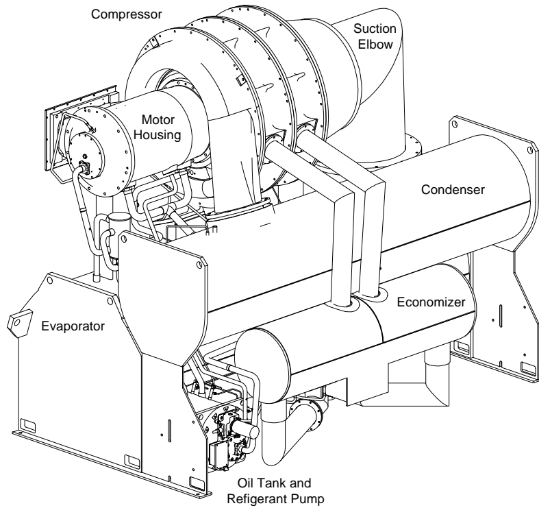
Figure 4 CVHE and CVHG with Refrigerant Pump
