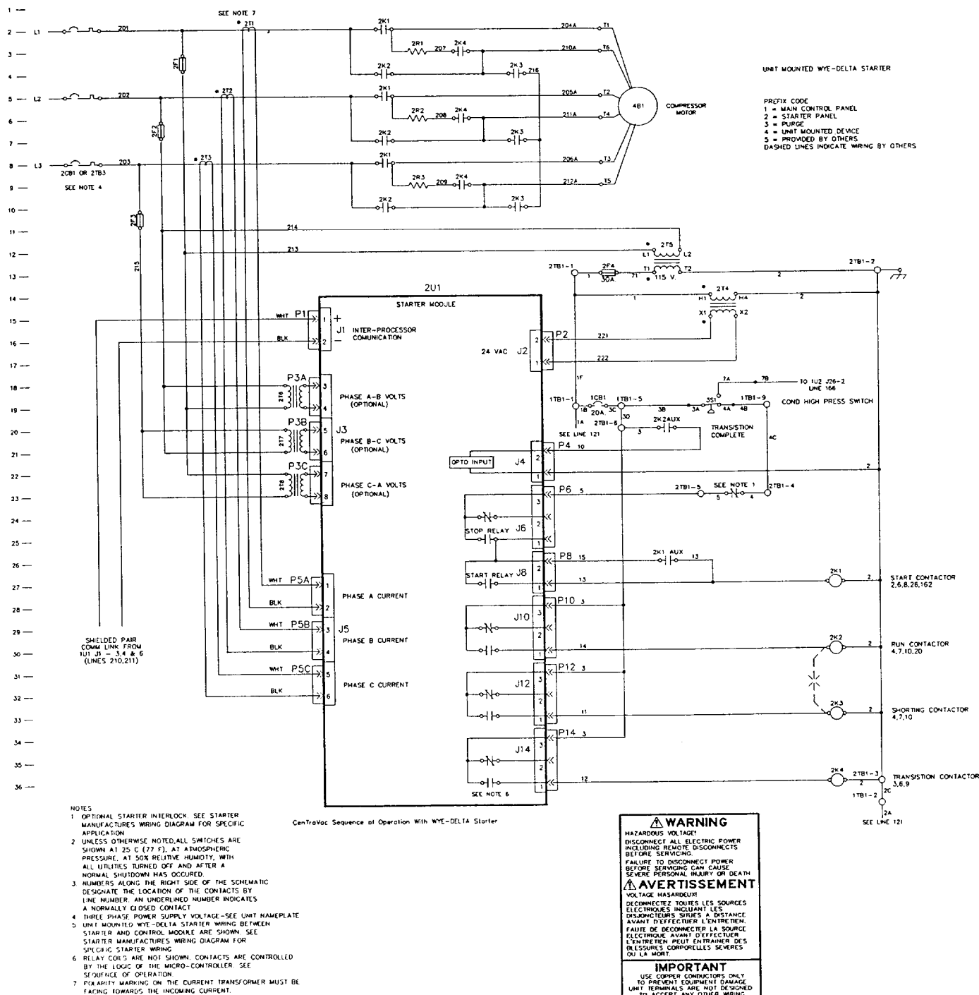
Figure 19 Starter Module - CVHE/CVHF with Factory Mounted Wye-Delta Starter
