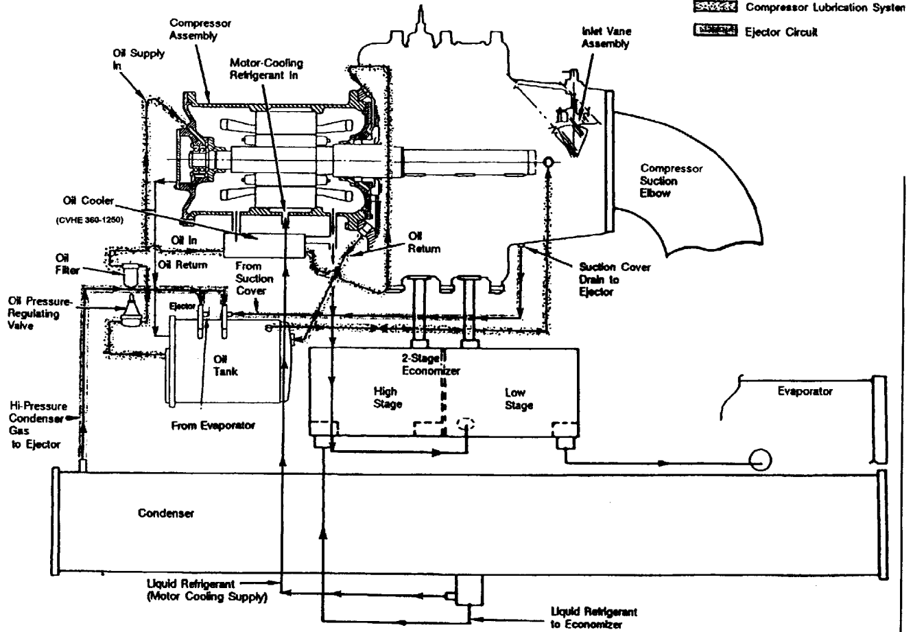
Figure 5 - CVHE Compressor Lubrication and Motor-Cooling Systems
