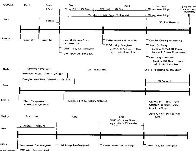
CentriVac Sequence of Operation With WYE-DELTA Starter
