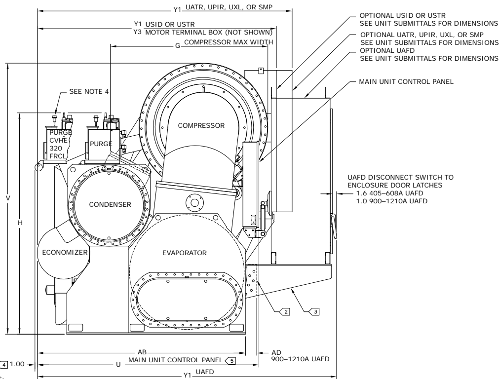
Figure 1. For Table 1, p. 6, Table 2, p. 6, and Table 3, p. 7: Assembly for CVHE, CVHF, and CVHG (CVHF-080 shown)
