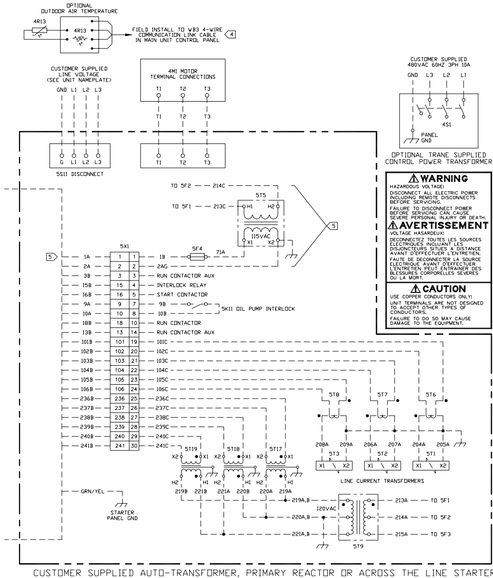
CUSTOMER SUPPLIED AUTO-TRANSFORMER, PRIMARY REACTOR OR ACROSS THE LINE STARTER
