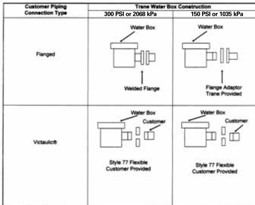
Figure 6. Customer piping alternatives for water connections
