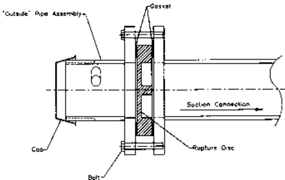
Cross Section of Rupture Disc
