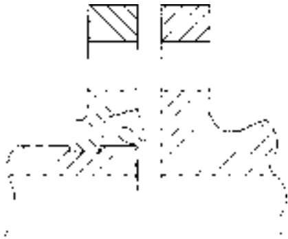
Figure 8. Typical victaulic flange gasket configuration
