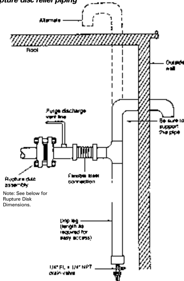
Figure 12. Arrangement for rupture disc relief piping
