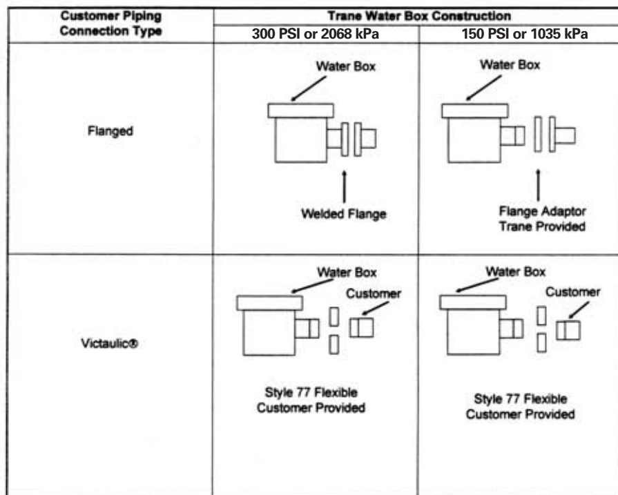
Figure 5 – Customer Piping Alternatives for Water Connections
