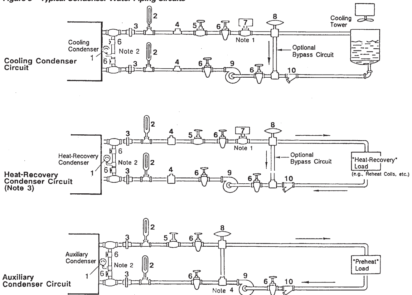
Figure 3 – Typical Condenser Water Piping Circuits
