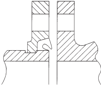
Figure 7 – Typical Victaulic Flange Gasket Configuration
