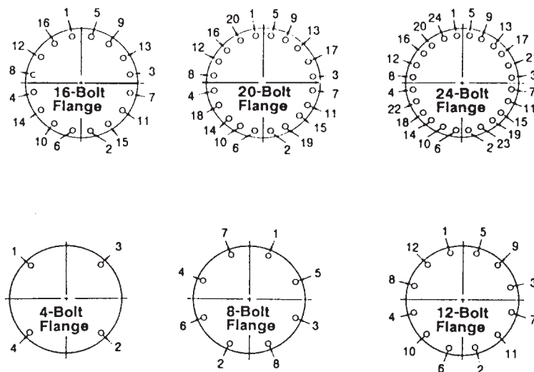
Figure 9 – Bolt Tightening Sequences for Water Piping Flanges and Water Boxes
