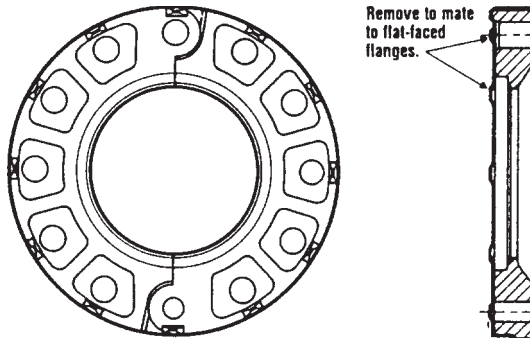
Figure 8 – Modifying 300 PSIG Flange Adaptors for Flat-Faced Flange Application
