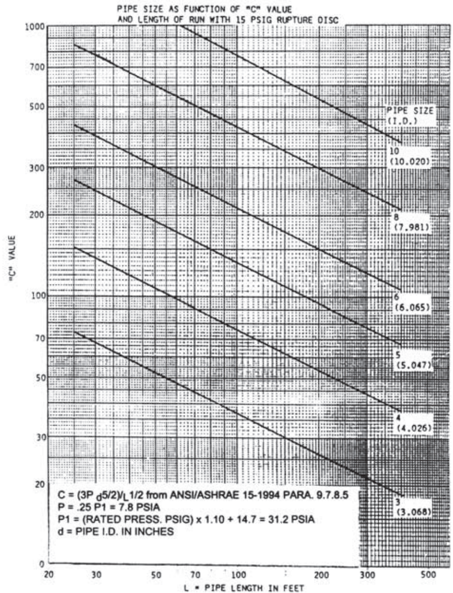
Figure 12 – Rupture Disc Vent Pipe Sizing
