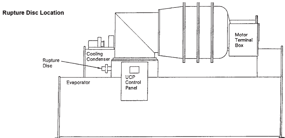
Figure 10 – Illustrates Rupture Disc Location, Cross Section of Rupture Disc and Recommended Rupture Disc Relief Piping
