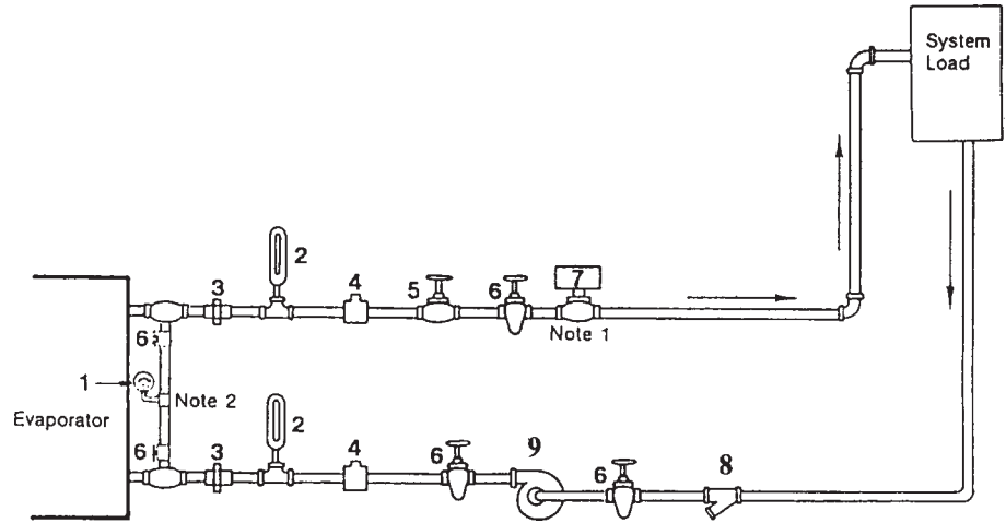
Figure 2 – Typical Evaporator Water Piping Circuit
