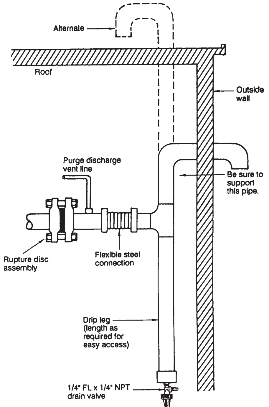
Figure 11 – Arrangement for Rupture Disc Relief Piping
