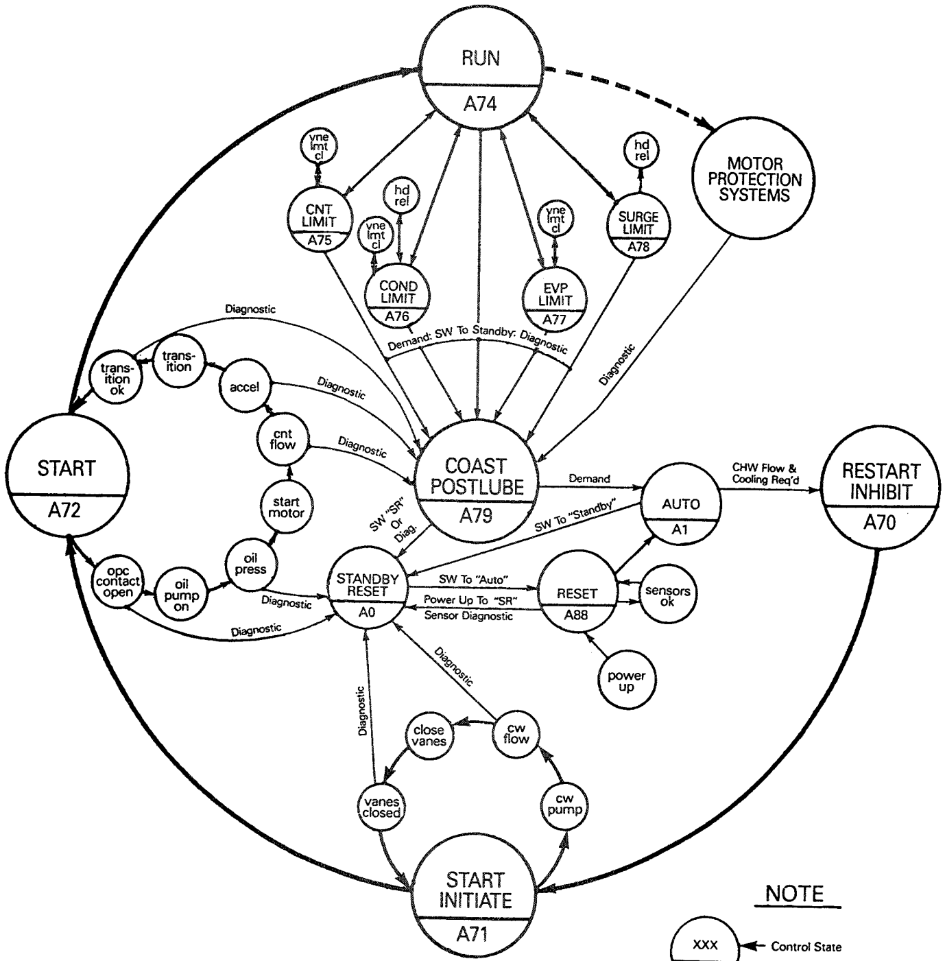
Figure 23 UCP Start-Run-Shutdown Sequence
