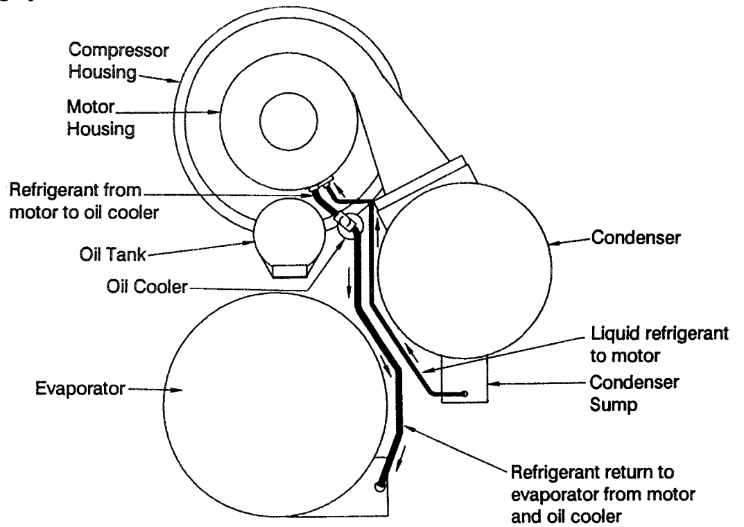
Figure 12 CVHF Motor Cooling System
