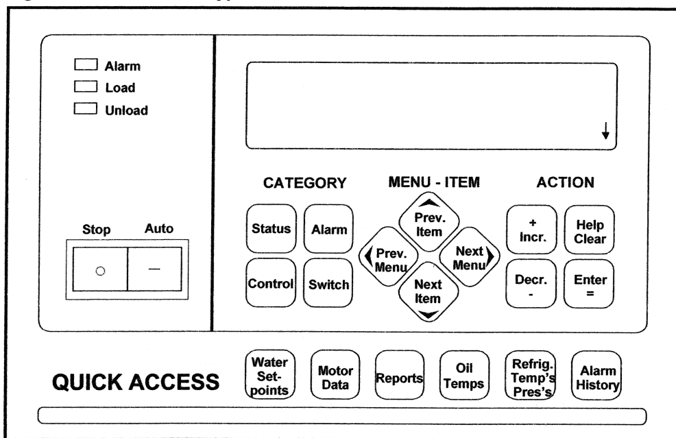
Figure 10, MicroTech Keypad
