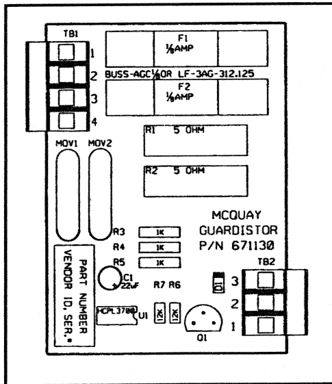
Figure 9, Guardistor Board
