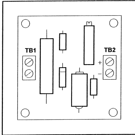
Figure 8, Signal Converter Board
