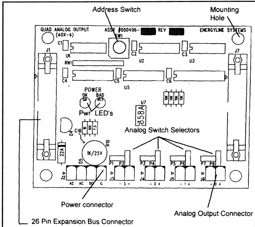
Figure 7, AOX Board
