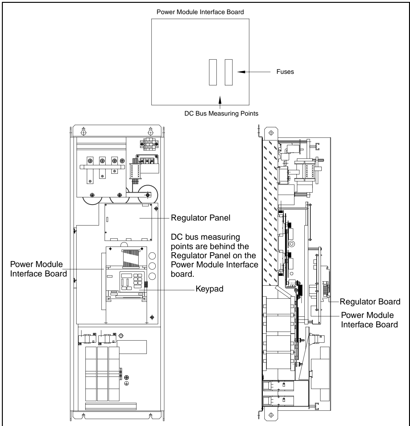
Figure 3.15 – Drive Components and Locations in 100 to 150HP @ 460VAC Drives
