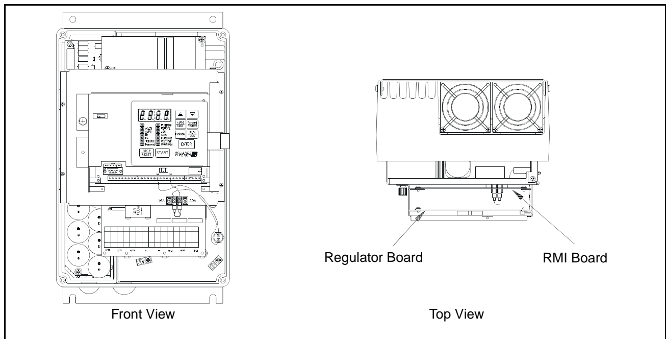
Figure 3.12 – RMI Board Location in 15 to 25 HP @ 460VAC Drives
