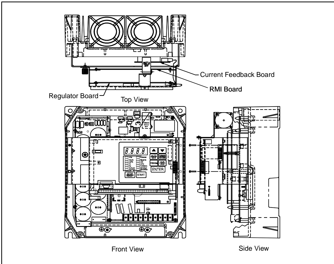
Figure 3.4 – RMI Board Location in 7.5 to 10HP Drives
