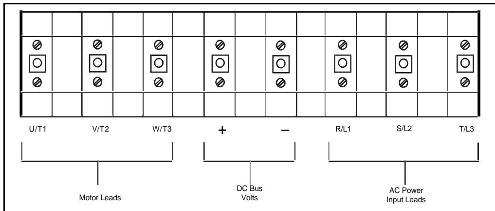
Figure 3.10 – DC Bus Voltage Terminals (15 to 25 HP @ 460VAC)
