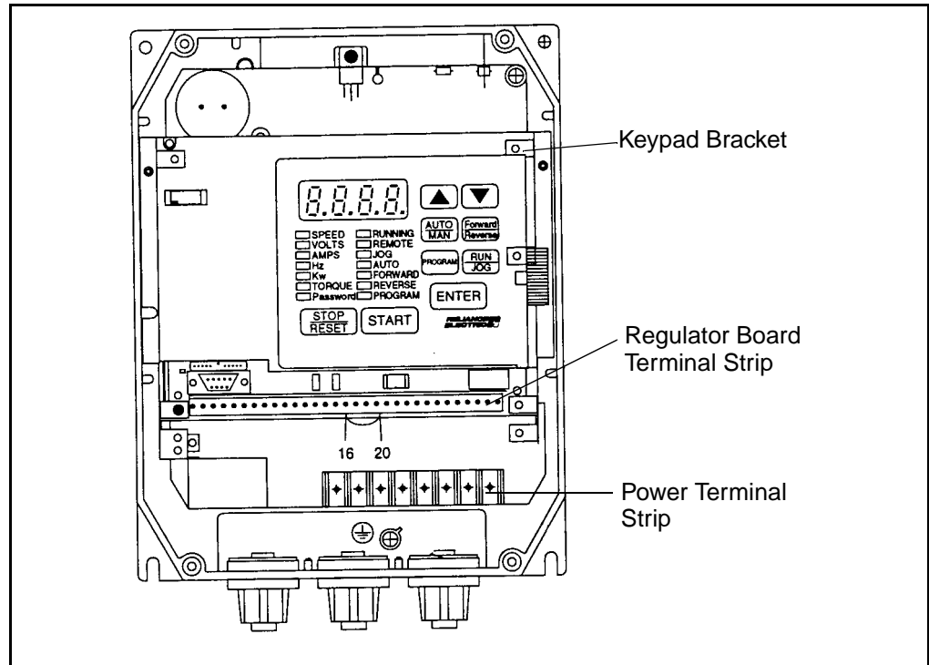
Figure 3.6 – 1 to 20HP @ 230 V GV3000/SE Drive
