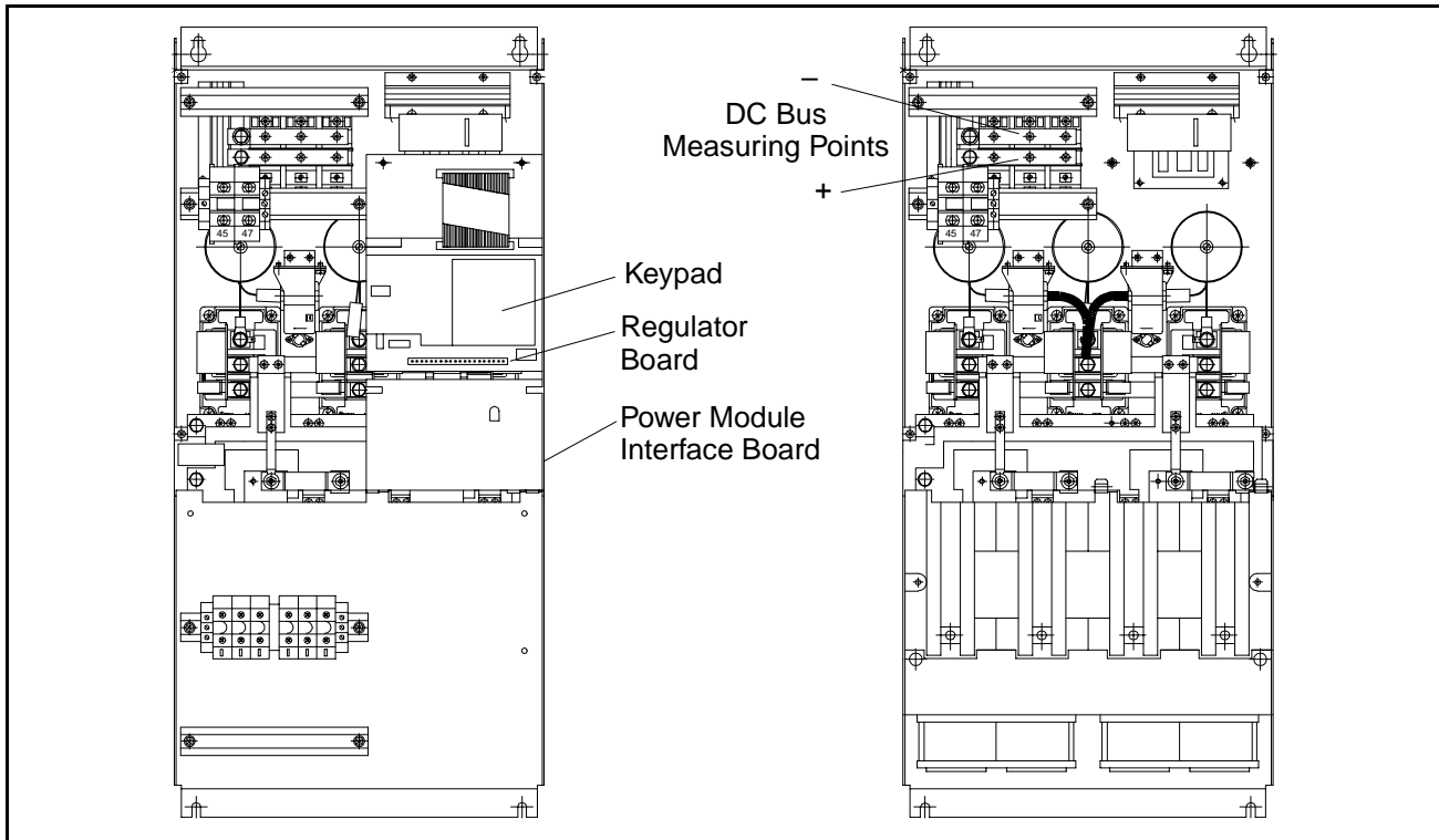
Figure 3.14 – Drive Components and Locations (50 to 100HP @ 460VAC)
