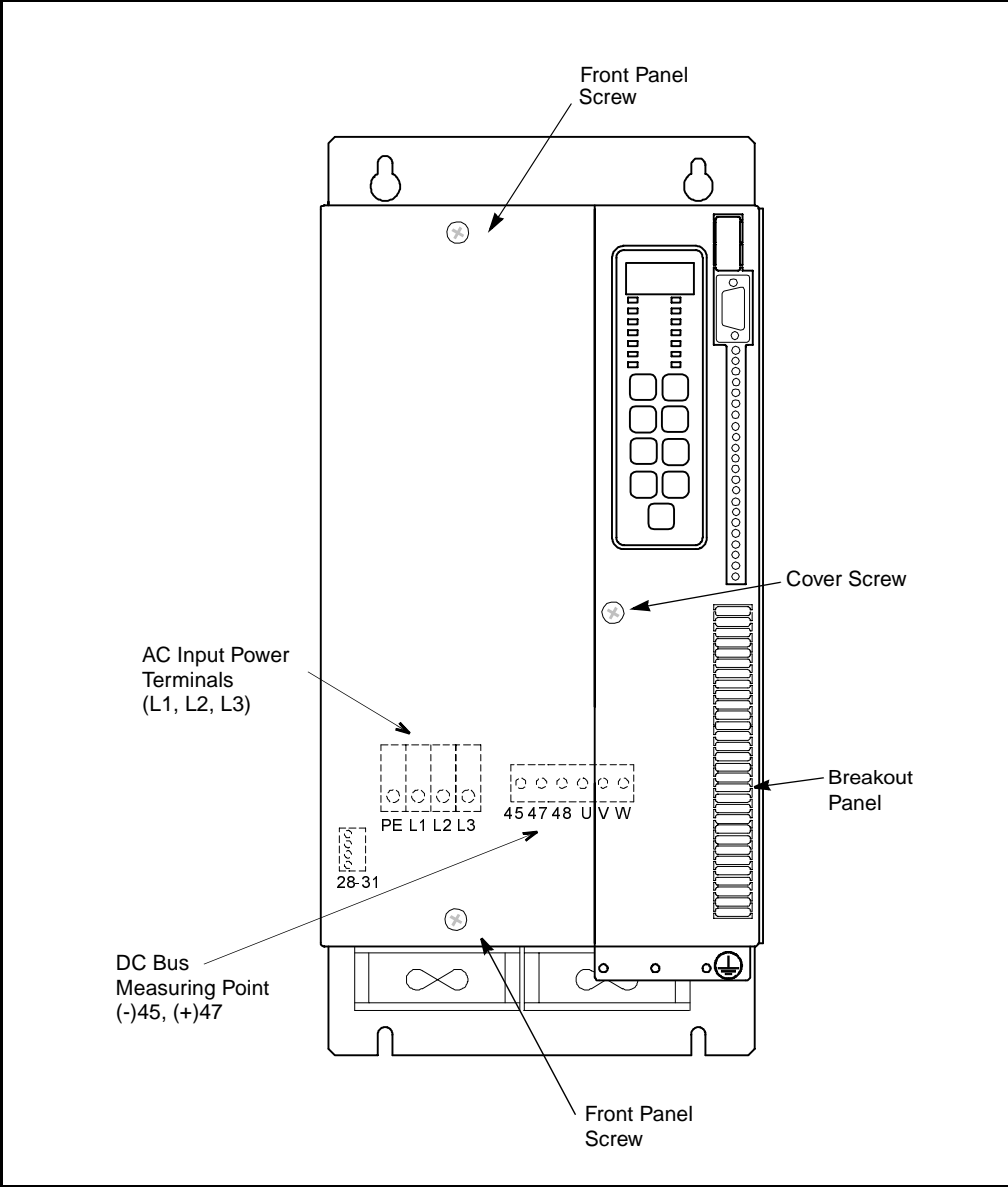
Figure 3.19 – 43 Amp GV3000/SE Bookshelf Drive
