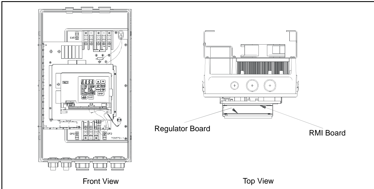
Figure 3.13 – RMI Board Location in 25 to 60 HP @ 460VAC Drives
