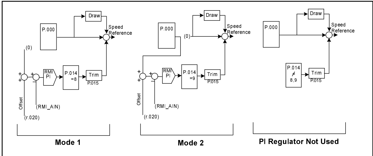
Figure 4.2 – PI Regulator Operating Modes
