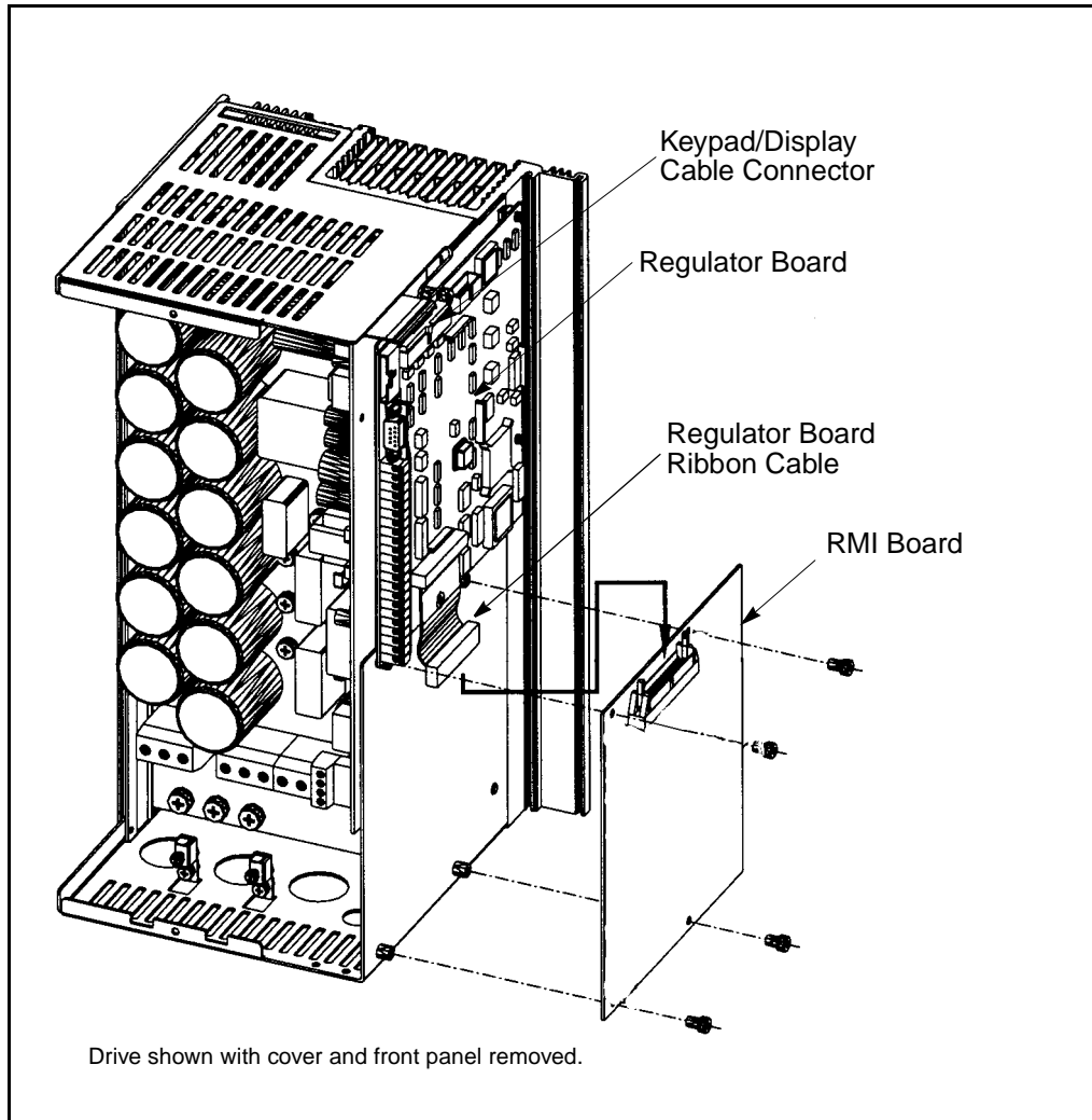
Figure 3.20 – Installing the RMI Board in a Bookshelf Drive
