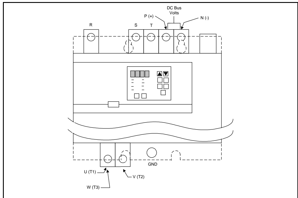
Figure 3.7 – DC Bus Voltage Terminals (30 to 100HP @ 230VAC and 75 to 200HP @ 460VAC)
