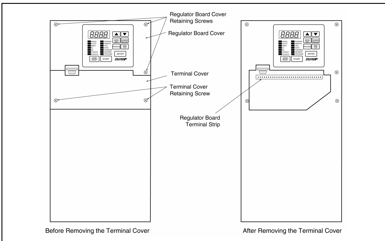
Figure 3.8 – Location of Terminal Cover and Regulator Board Cover in 30 to 100HP @ 230VAC and 75 to 200HP @ 460VAC Drives
