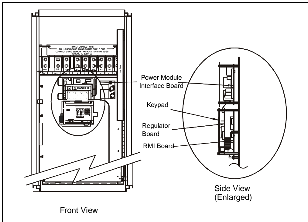
Figure 3.16 – RMI Board Location in 200 to 400HP @ 460VAC Drives
