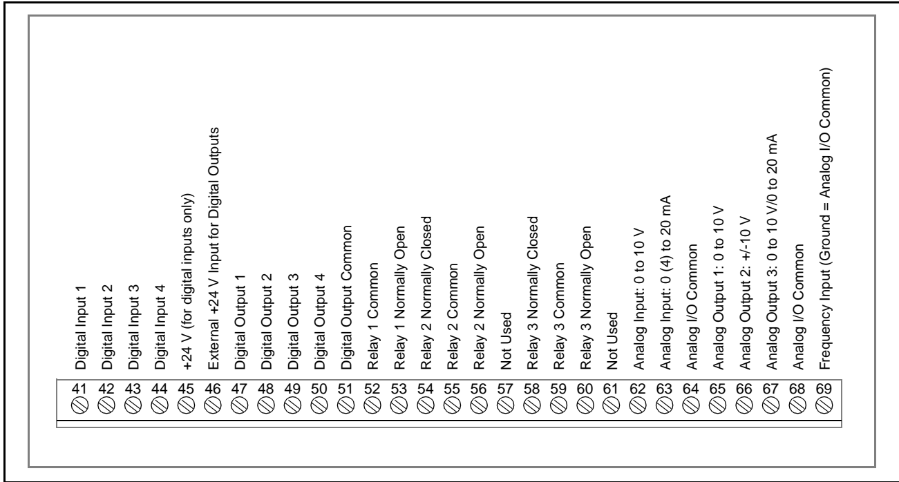
Figure 3.21 – Terminal Connections on the RMI Board
