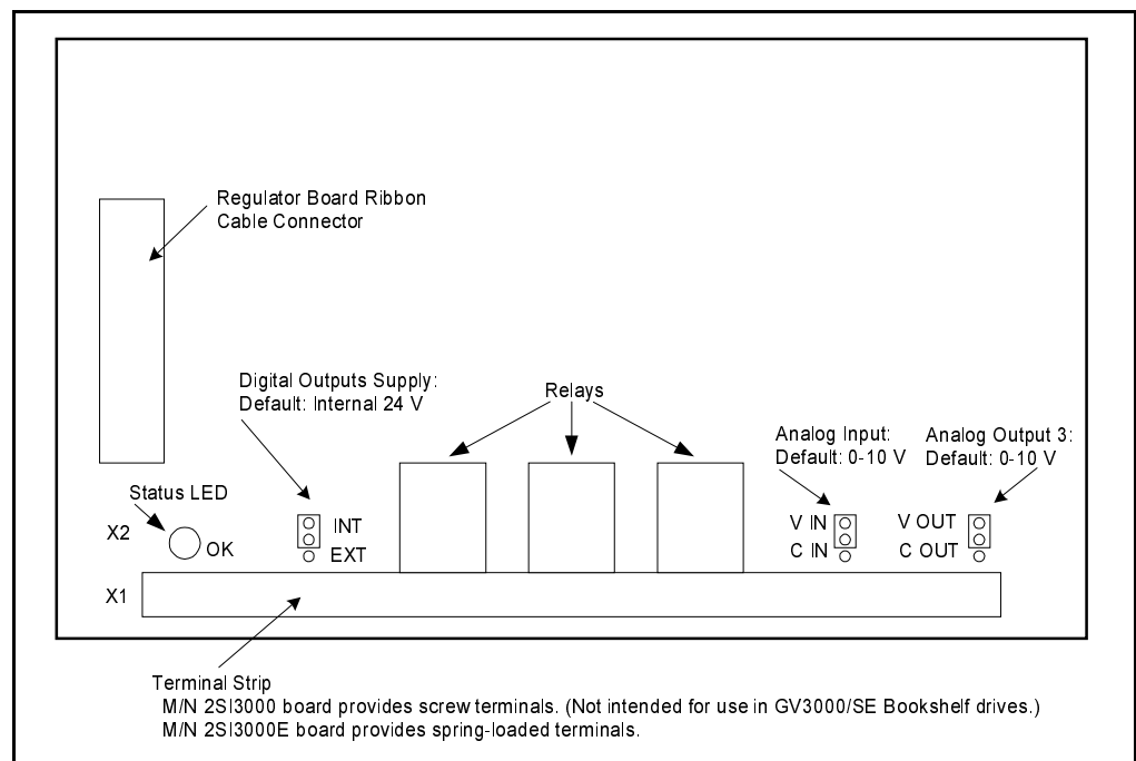
Figure 2.1 – RMI Board
