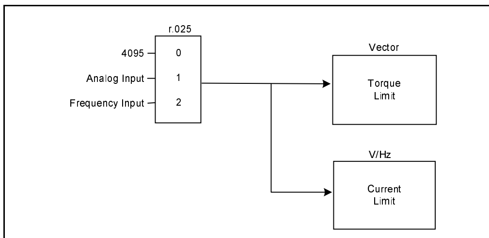
Figure 4.3 – Torque or Current Limit Selection
