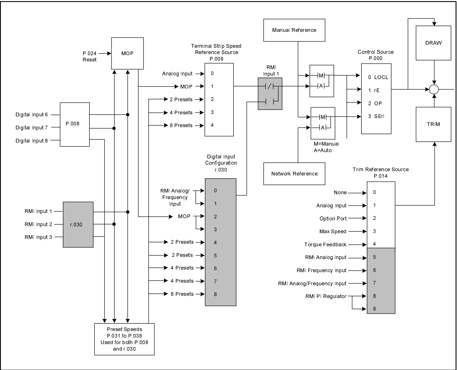
Figure 4.4 – Speed Reference Options
