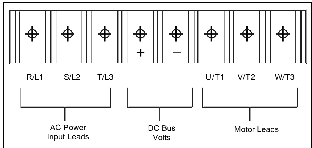
Figure 3.5 – DC Bus Voltage Terminals (1 to 20HP @ 230VAC)
