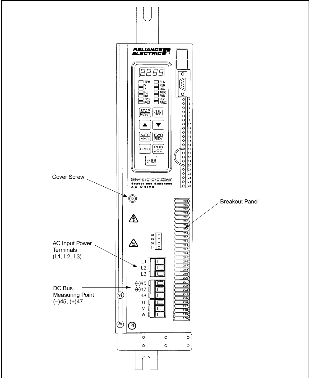
Figure 3.17 – 2 to 15 Amp GV3000/SE Bookshelf Drive
