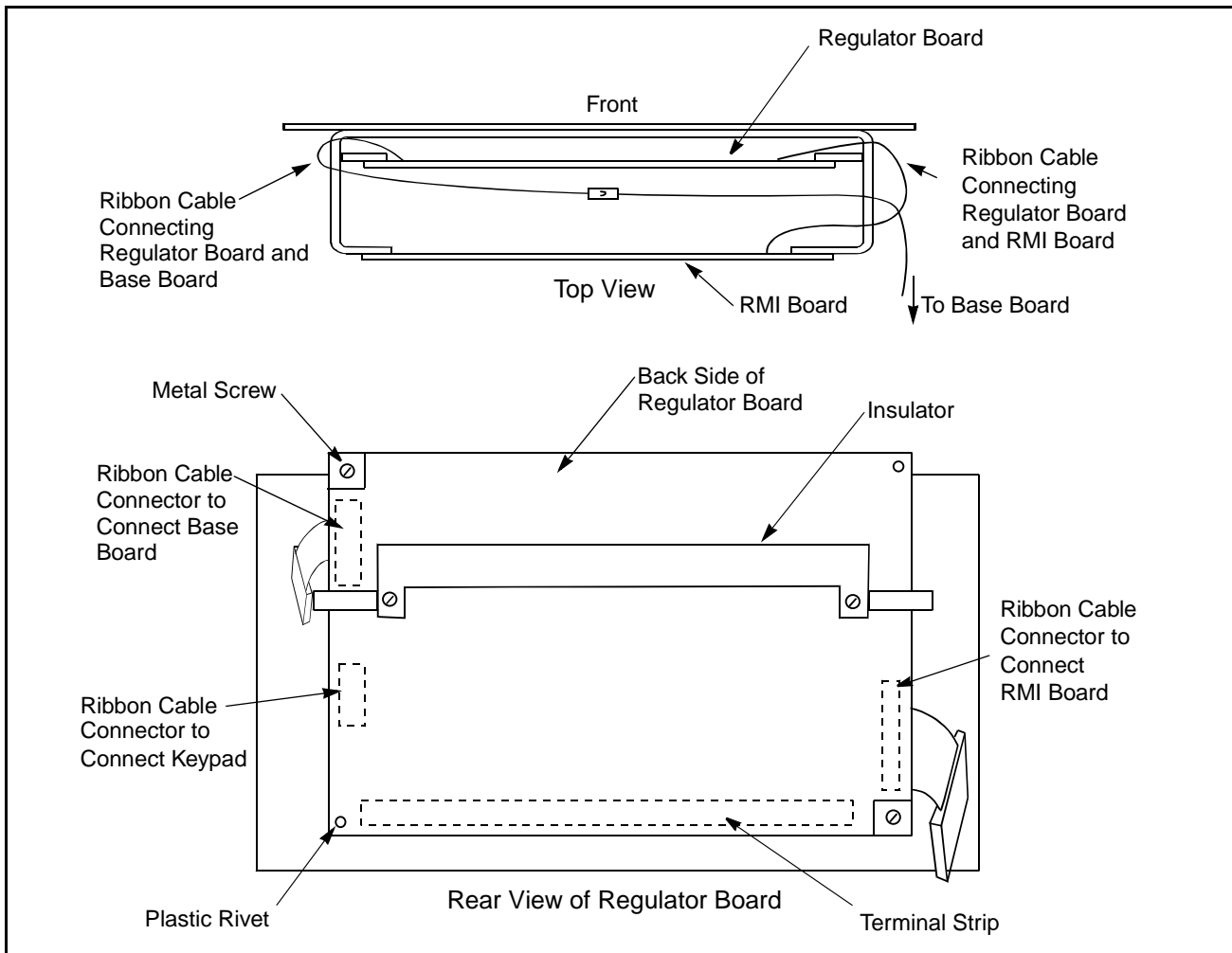
Figure 3.9 – Regulator Board's Connection to RMI Board, Keypad, and Base Board
