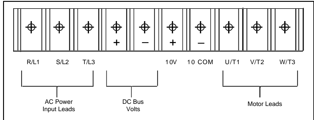
Figure 3.3 – DC Bus Voltage Terminals (7.5 to 10HP @ 460VAC)
