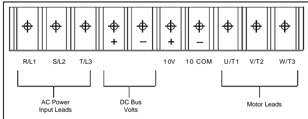
Figure 3.1 – DC Bus Voltage Terminals (1 to 5HP @ 460VAC)
