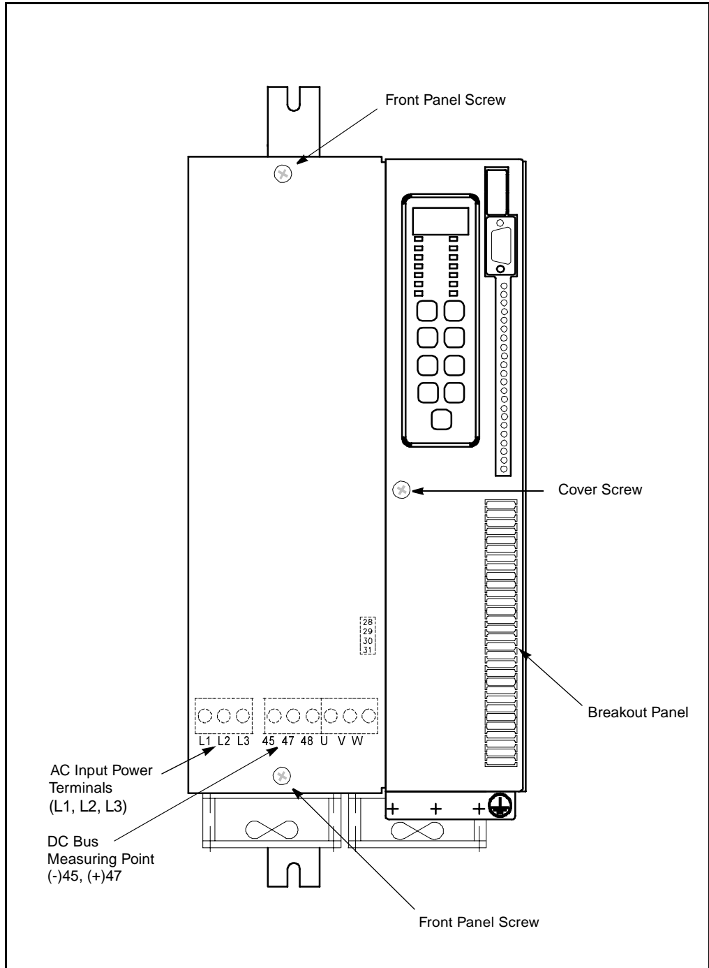
Figure 3.18 – 24 to 30 Amp GV3000/SE Bookshelf Drive
