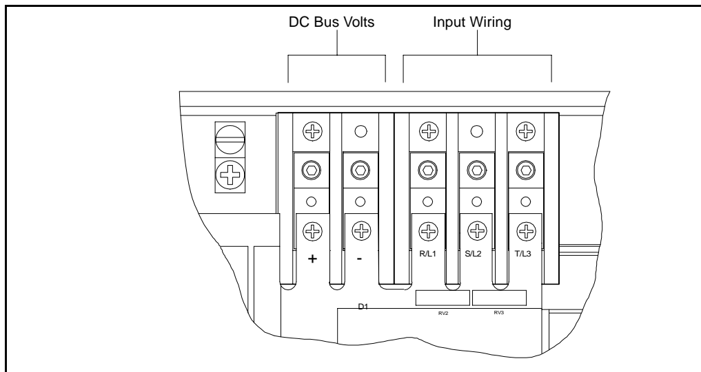
Figure 3.11 – DC Bus Voltage Terminals (25 to 60 HP @ 460VAC)
