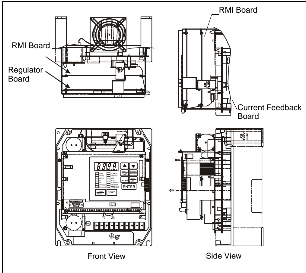
Figure 3.2 – RMI Board Location in 1 to 5HP @ 460VAC Drives
