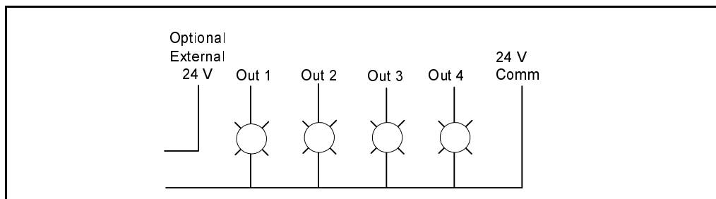
Figure 2.3 – Digital Output Circuit
