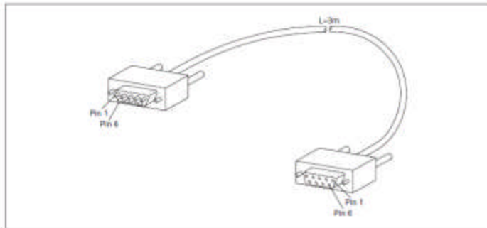
Figure C-3: RS-232 Cable
