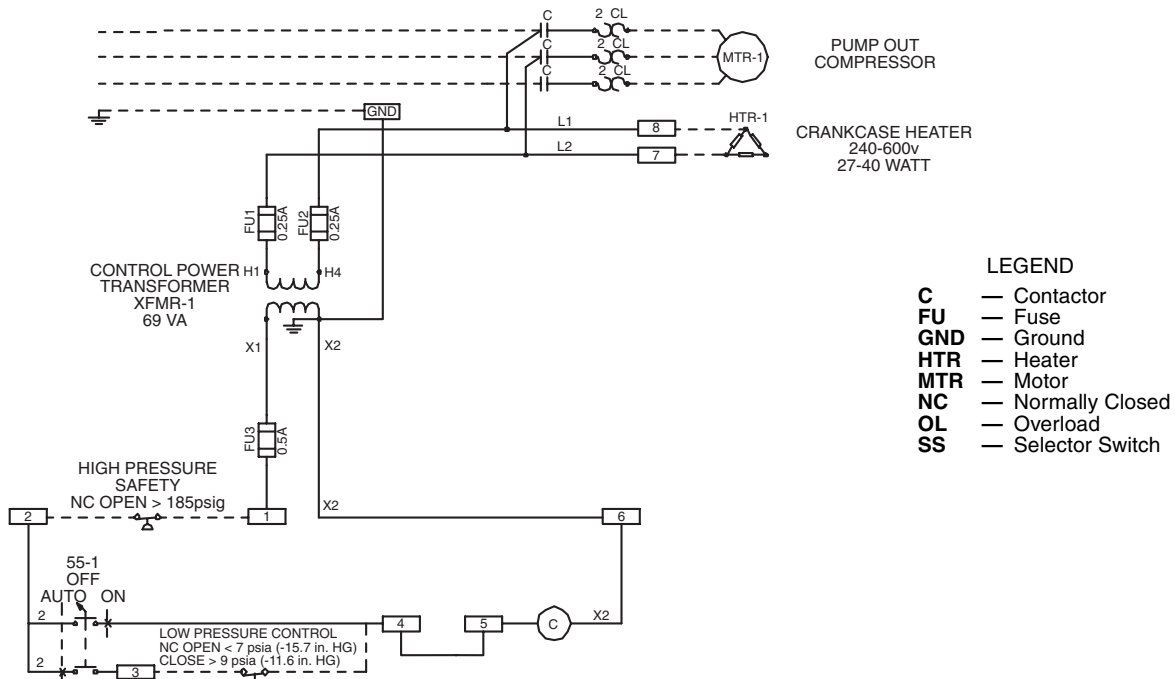
Fig. 8 — Pumpout Unit Wiring Schematic
