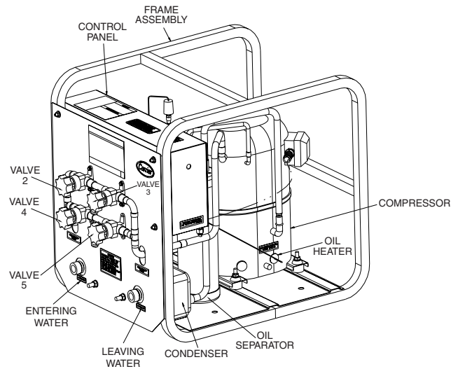
Fig. 9 — Pumpout Unit
