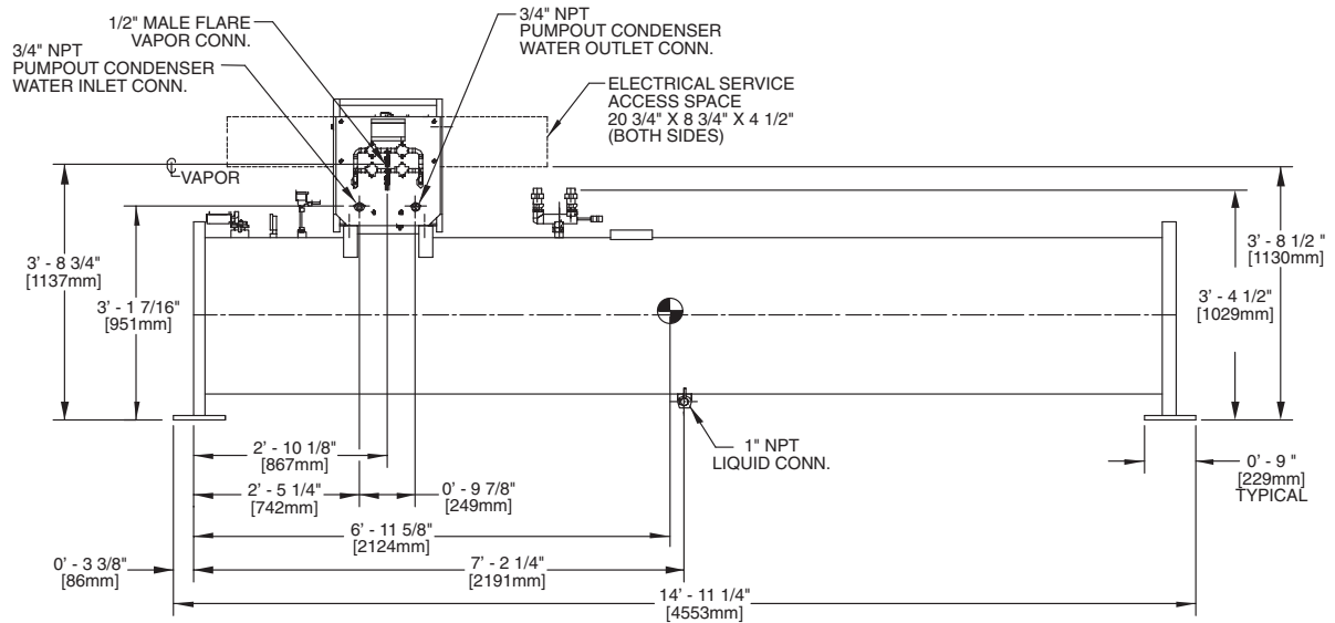
FRONT VIEW
