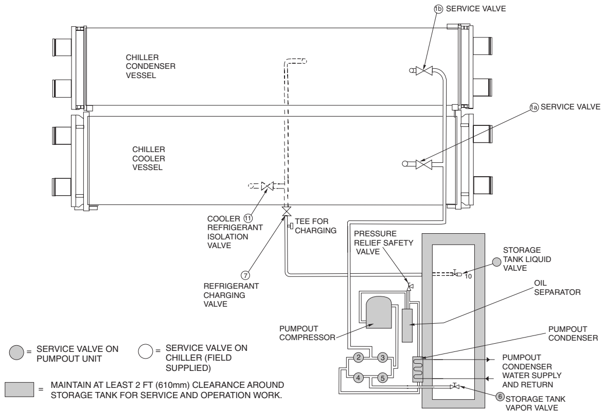
Fig. 10 — Valve Locations for 19XR Pumpout Unit With 19XB Storage Tank
