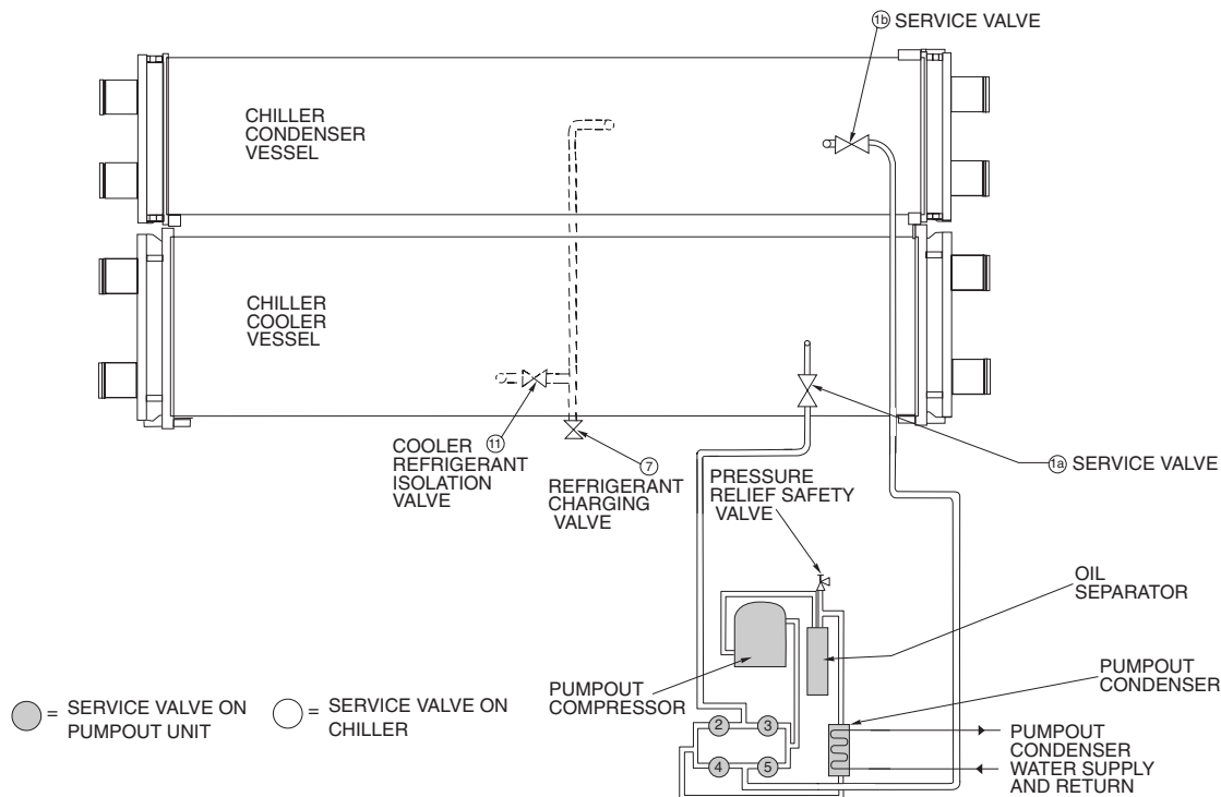
Fig. 11 — Valve Locations for 19XR Pumpout Unit Without Storage Tank
