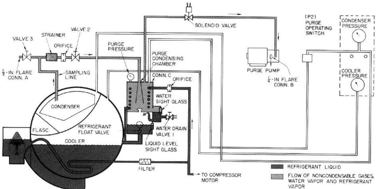
Fig. 12 — Purge Cycle
