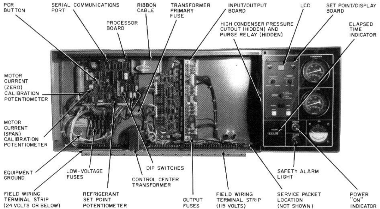
Fig. 2 — Control Center
