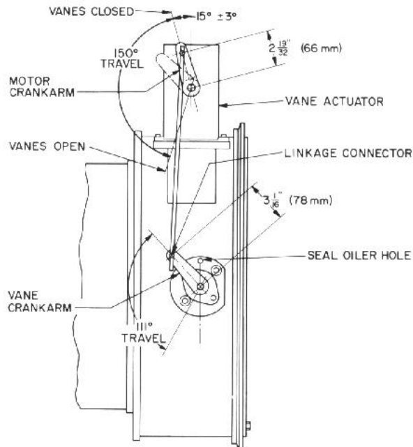
Fig. 9 — Guide Vane Linkage (Closed Position)
