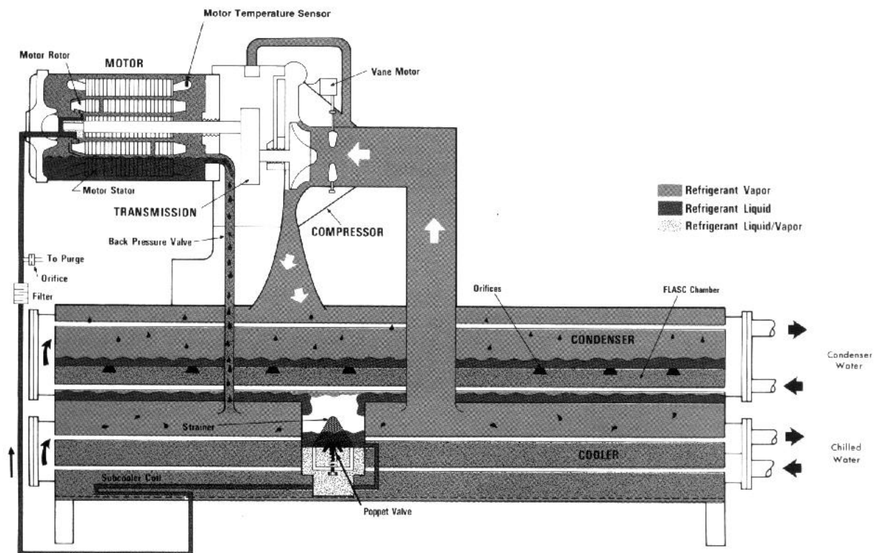
Fig. 10 — Refrigeration and Motor Cooling Cycles
