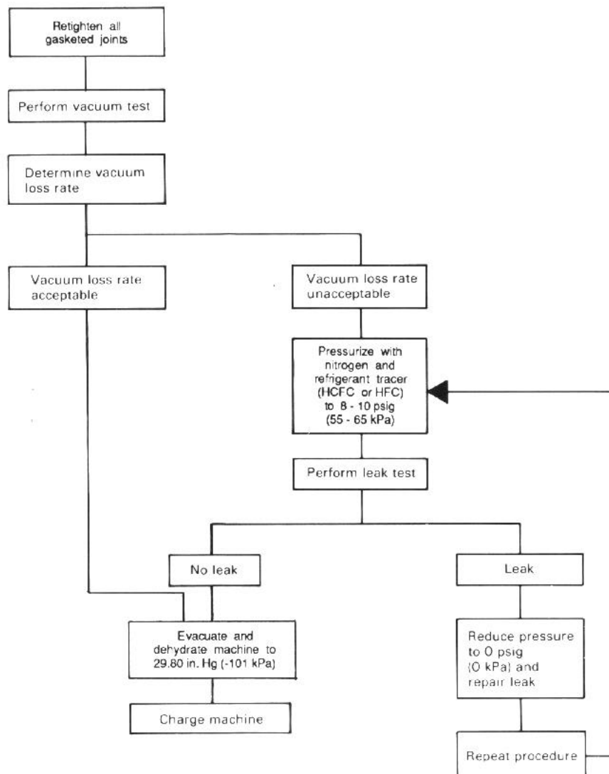
→ Fig. 5 — 19DK Leak Test Sequence and Procedures
