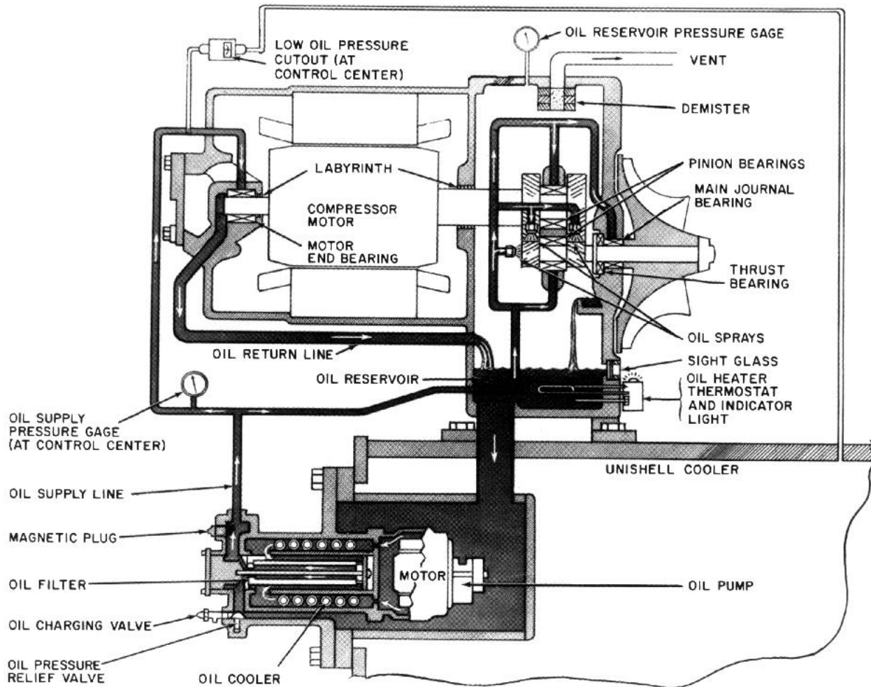
Fig. 11 — Lubrication Cycle
