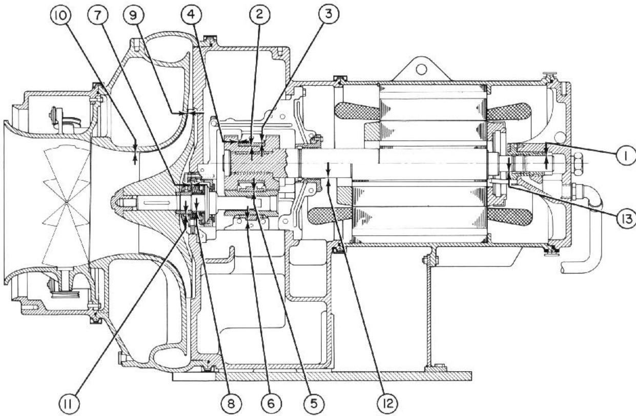
Fig. 13 — Compressor Fits and Clearances
