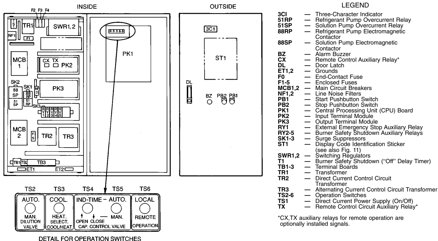
Fig. 10 — Control Panel
