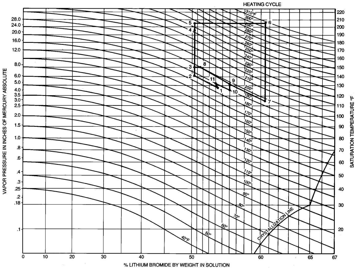
Fig. 8 — Equilibrium Diagram, Heating Cycle
