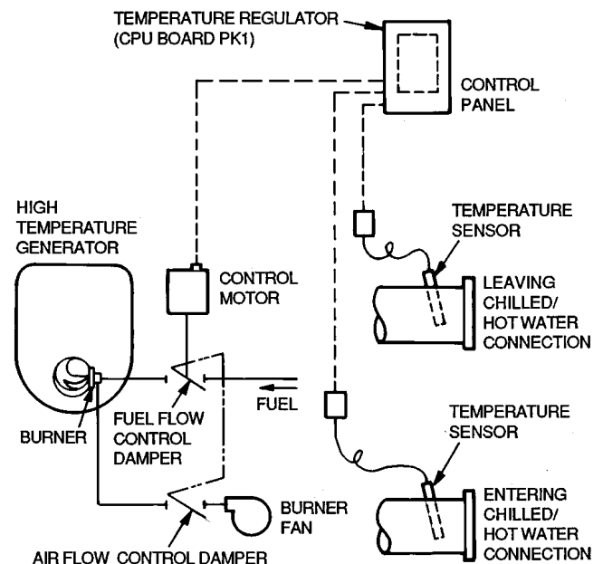
Fig. 27 — Automatic Capacity Controller
