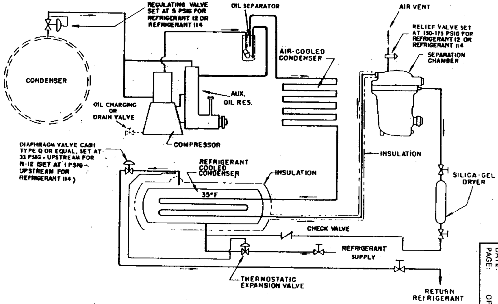
PURGE SYSTEM - DIAGRAM
