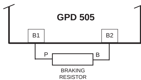
Figure A7-2. Lead Connections For Braking Resistor (Heat Sink Mounted)
