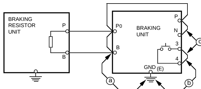
Figure A7-6. Megger Testing Set-up
