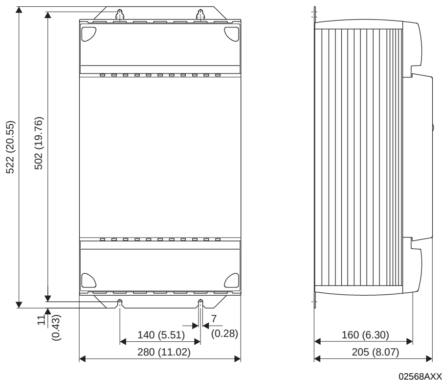
Fig. 29: Dimensions, MDR60A size 4, in mm (in)
