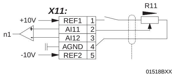
Fig. 99: Switching the potentiometer setpoint
