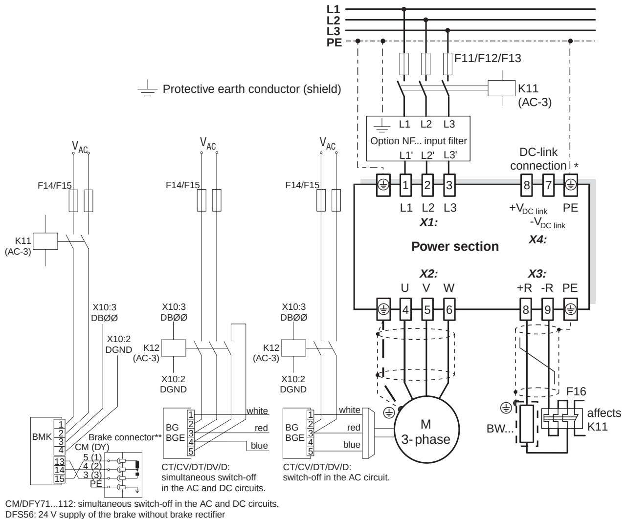
Fig. 118: Wiring diagram, power section and brake
