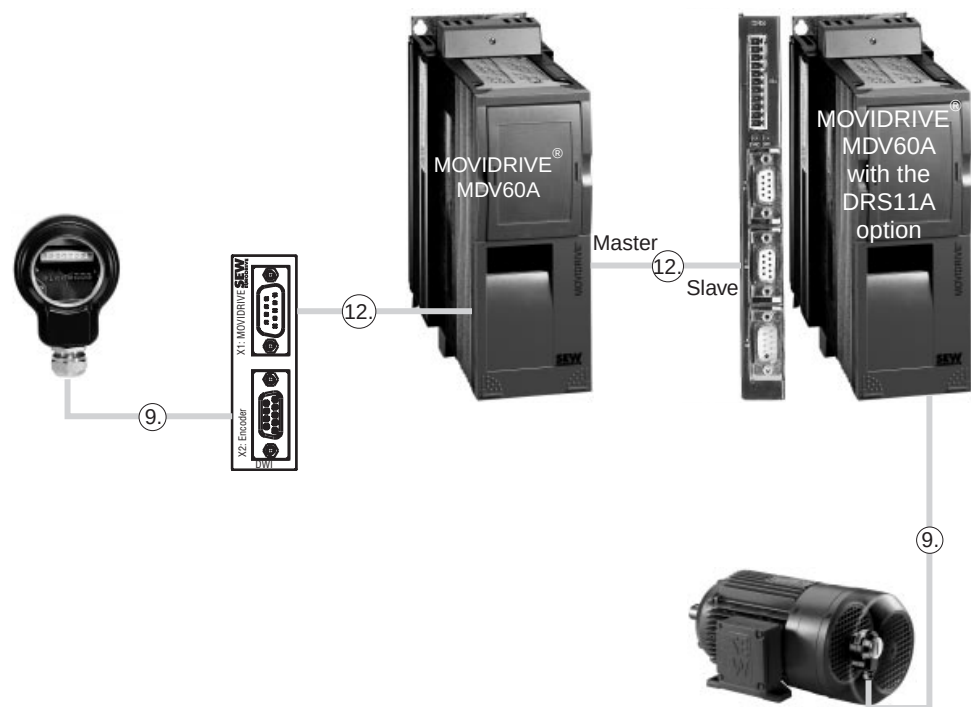
Fig. 48: Connection of motor encoder and master/slave connection
