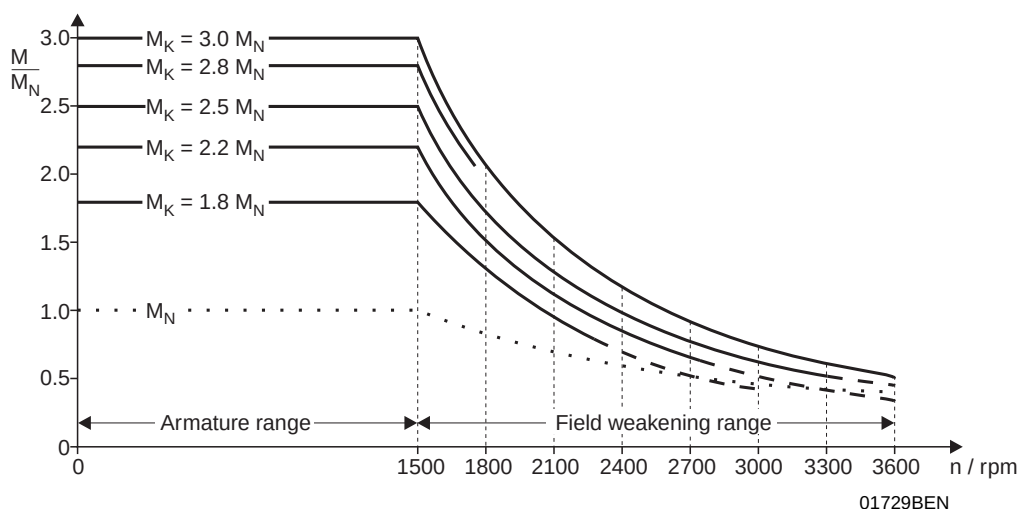
Fig. 82: Quadratically falling breakdown torque
