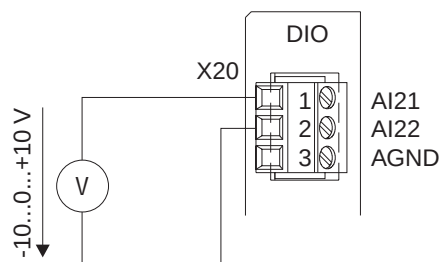
Fig. 127: Setpoint input n2
