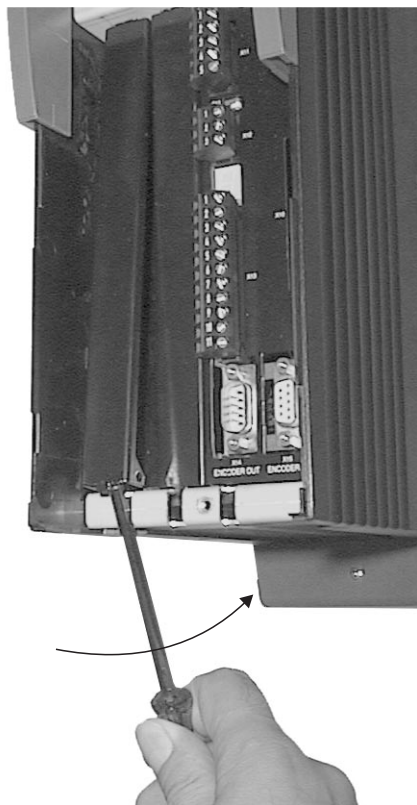
Fig. 125: Lever out the cover plate
