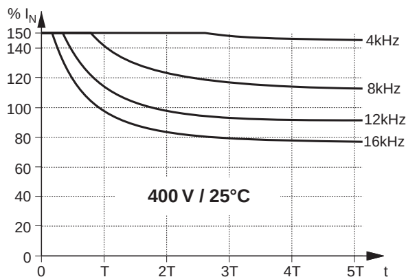
Fig. 86: Overload capacity at \vartheta_{amb} = 25^\circ\text{C}
