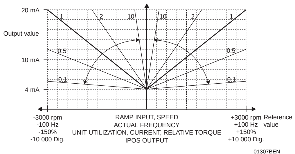
Fig. 69: Characteristic of 4 – 20 mA operating mode
