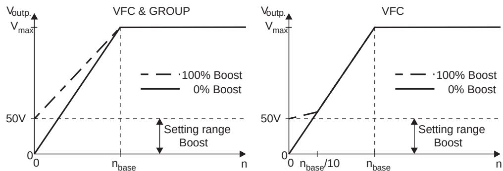
Fig. 63: Working principle of boost (drawing not to scale)
