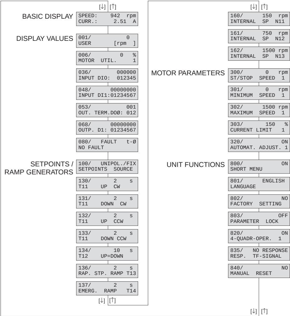
Fig. 152: DBG11A quick menu
