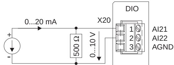
Fig. 128: Current input with external load
