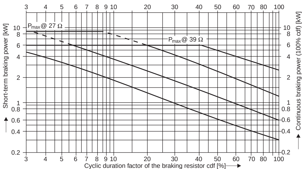
Fig. 91: Power diagram for wire resistors 230 V units
