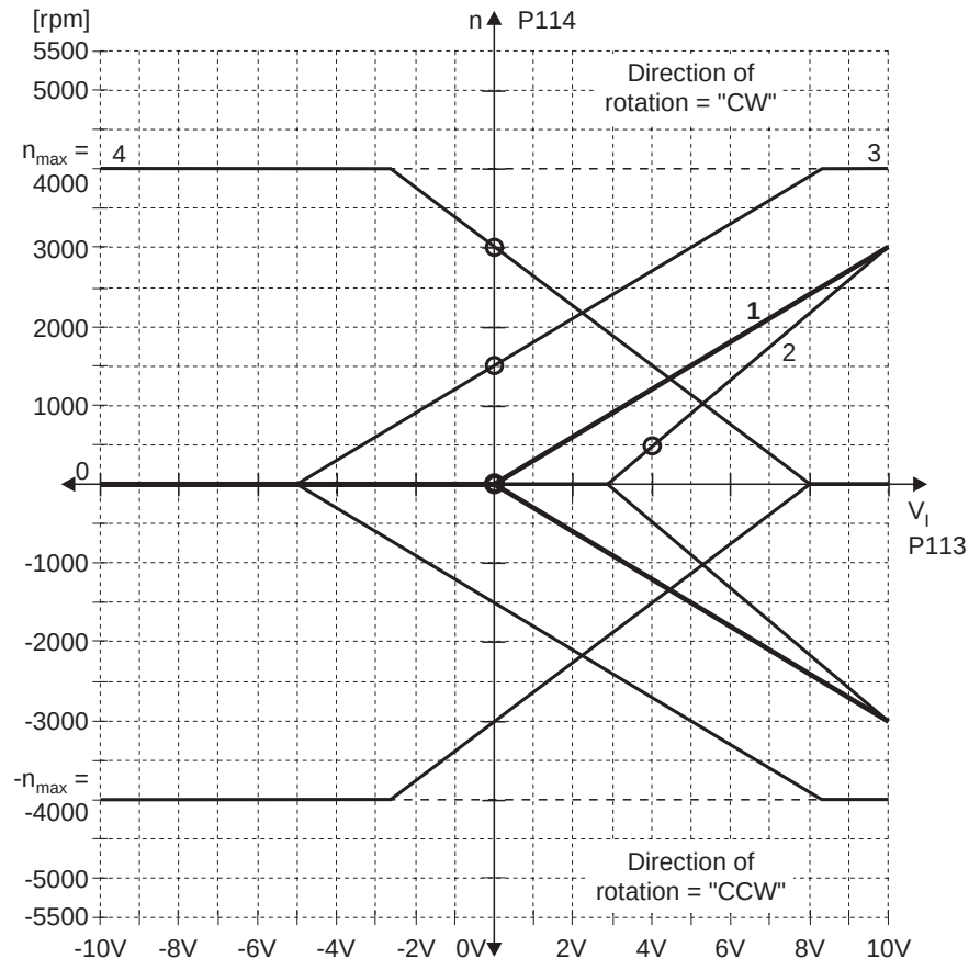
Fig. 57: Samples of expert characteristics with P100 "Setpoint source" = "UNIPOL./FIX.SETPT"
