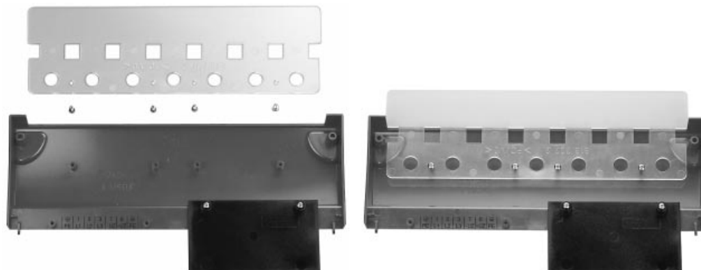
Fig. 117: Touch guard for MOVIDRIVE® sizes 4 and 5
