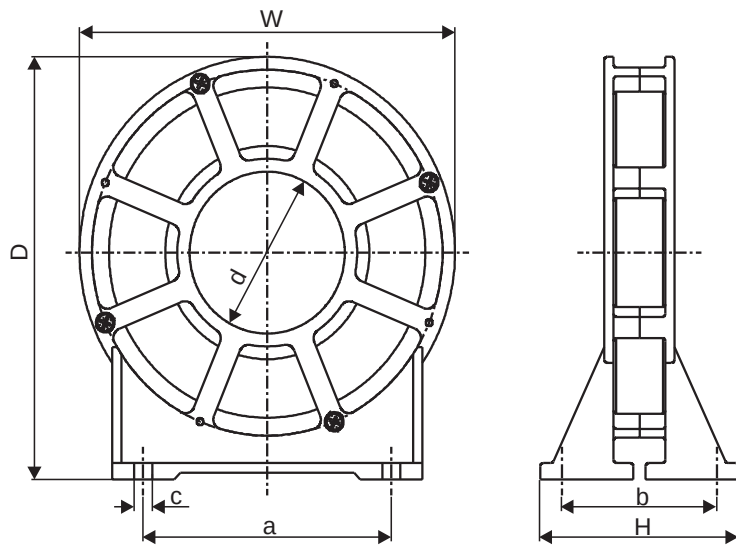
Fig. 42: Dimensions, HD... output chokes
