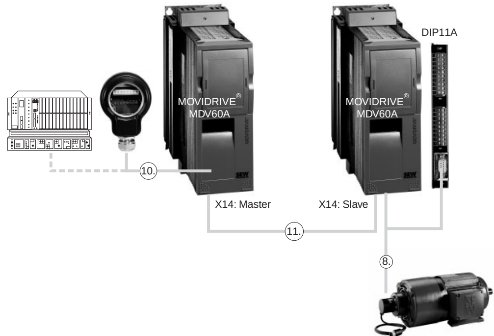
Fig. 47: Connection of external encoder, combination encoder and master/slave connection
