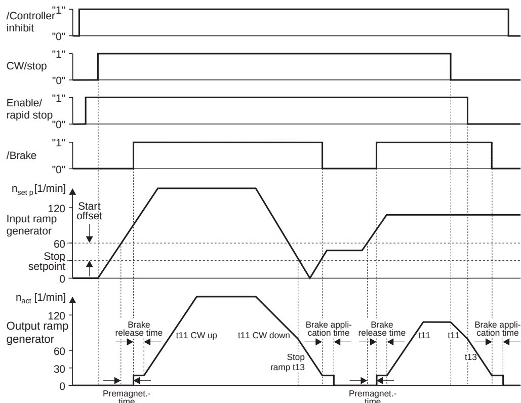
Fig. 73: Setpoint stop function
