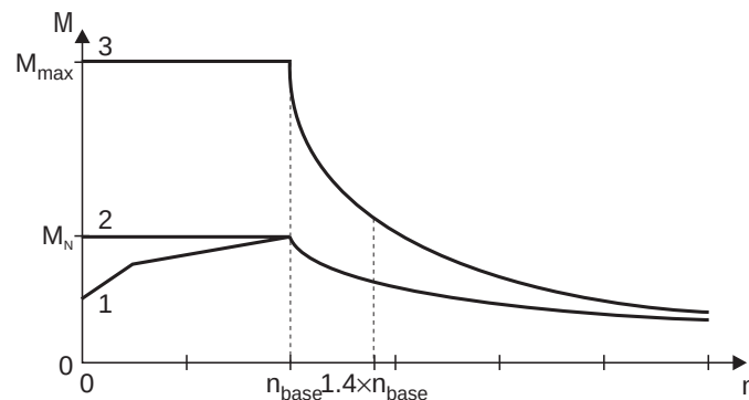
Fig. 83: Speed/torque characteristic curve in CFC operating mode
