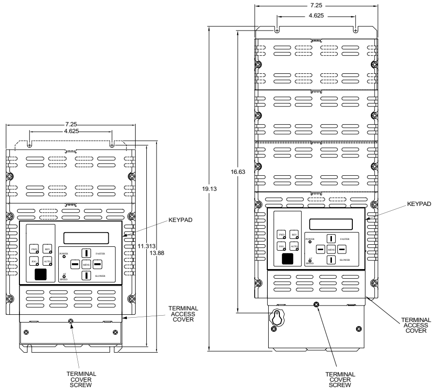
FIGURE 4-2. 6500 CONTROLLER MOUNTING DIMENSIONS, 7.5 - 20HP, 230/460V
