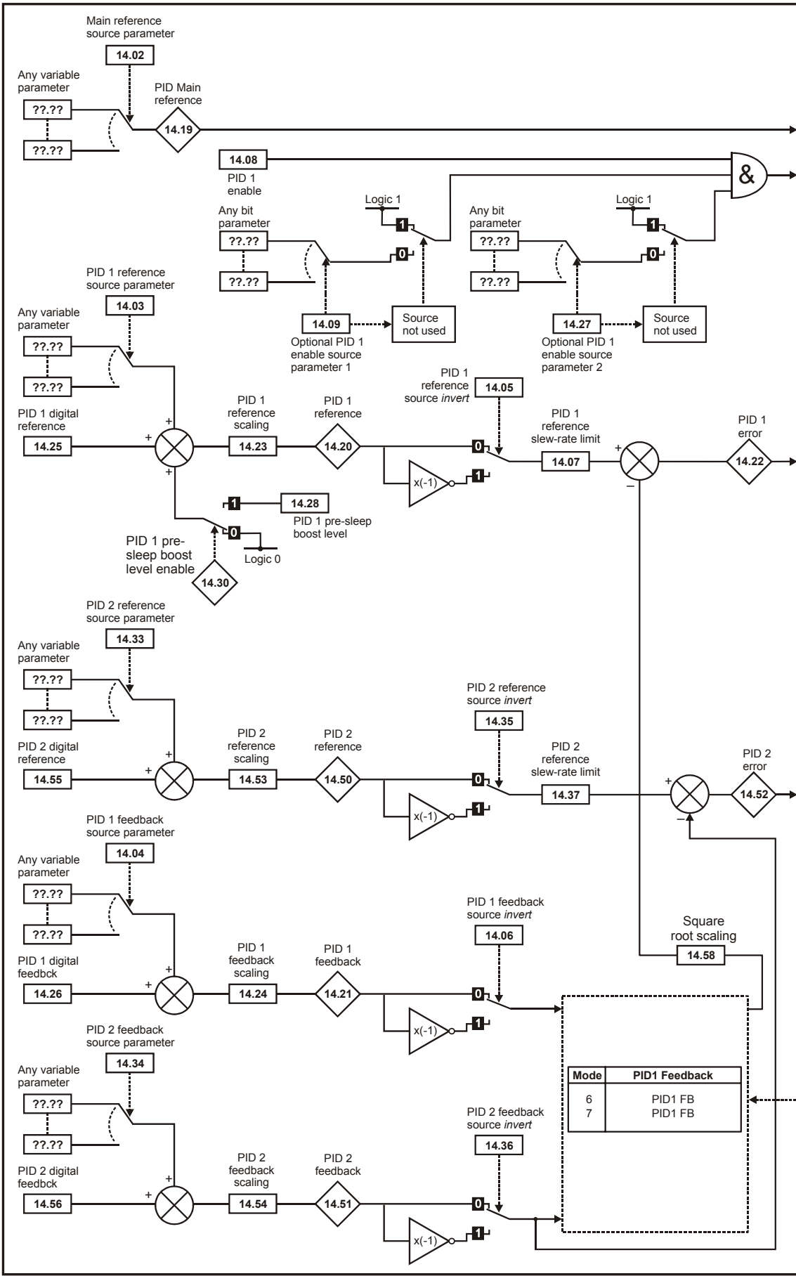
Figure 5-21 Menu 14 Logic diagram - Combined control
