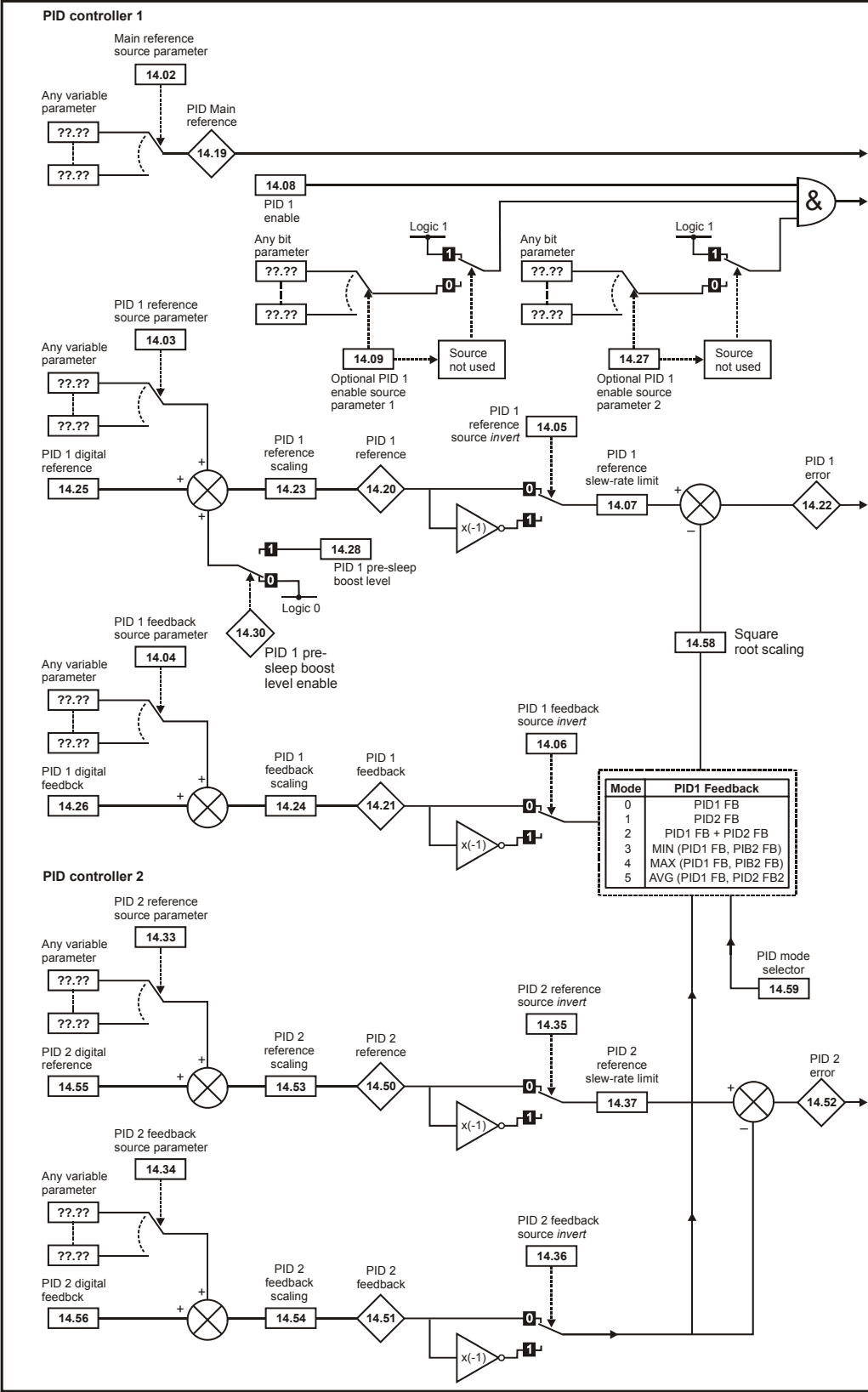
Figure 5-20 Menu 14 logic diagram
