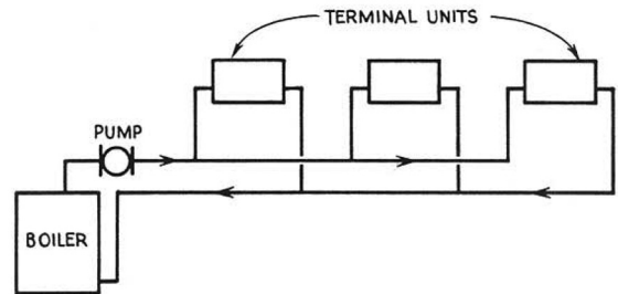
Figure 2 Typical Direct-Return Piping System
