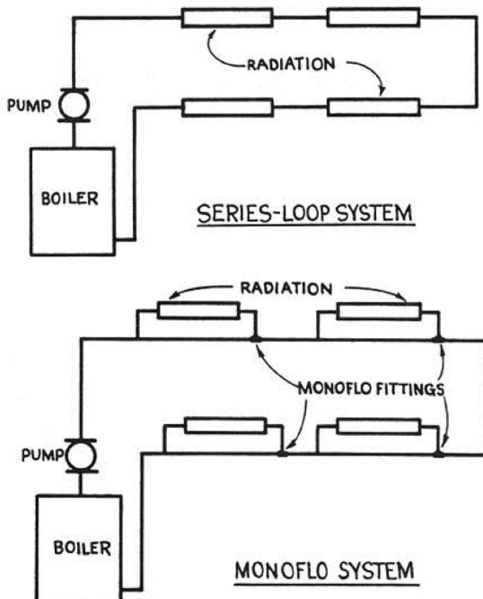
Figure 5 Typical One-Pipe Systems
