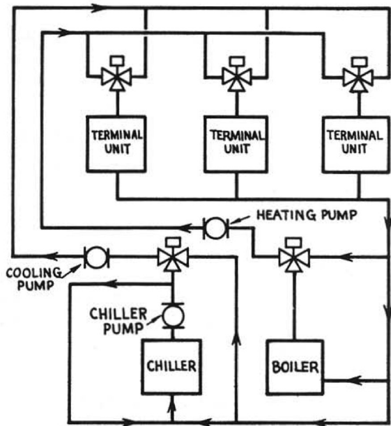
Figure 6 Typical Three-Pipe System
