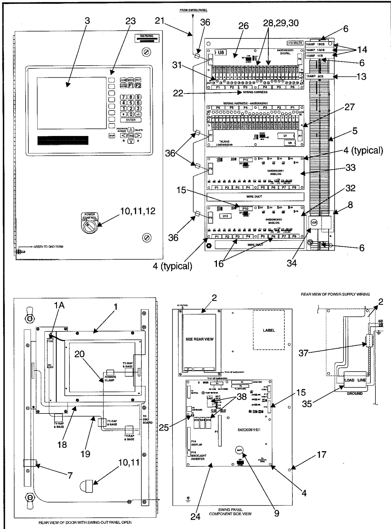
Figure 28. Quantum Control Panel, Typical.
