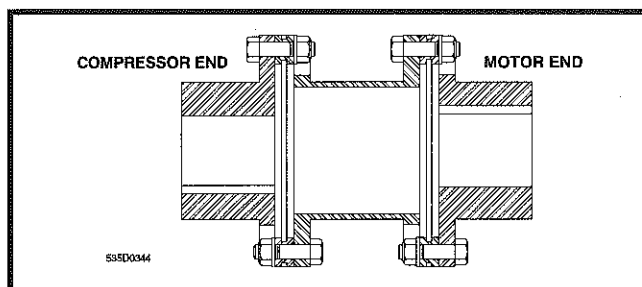
FIGURE 23. Drive Coupling, Models 316—676. COUPLING ASSEMBLIES-FIGURE 23.
