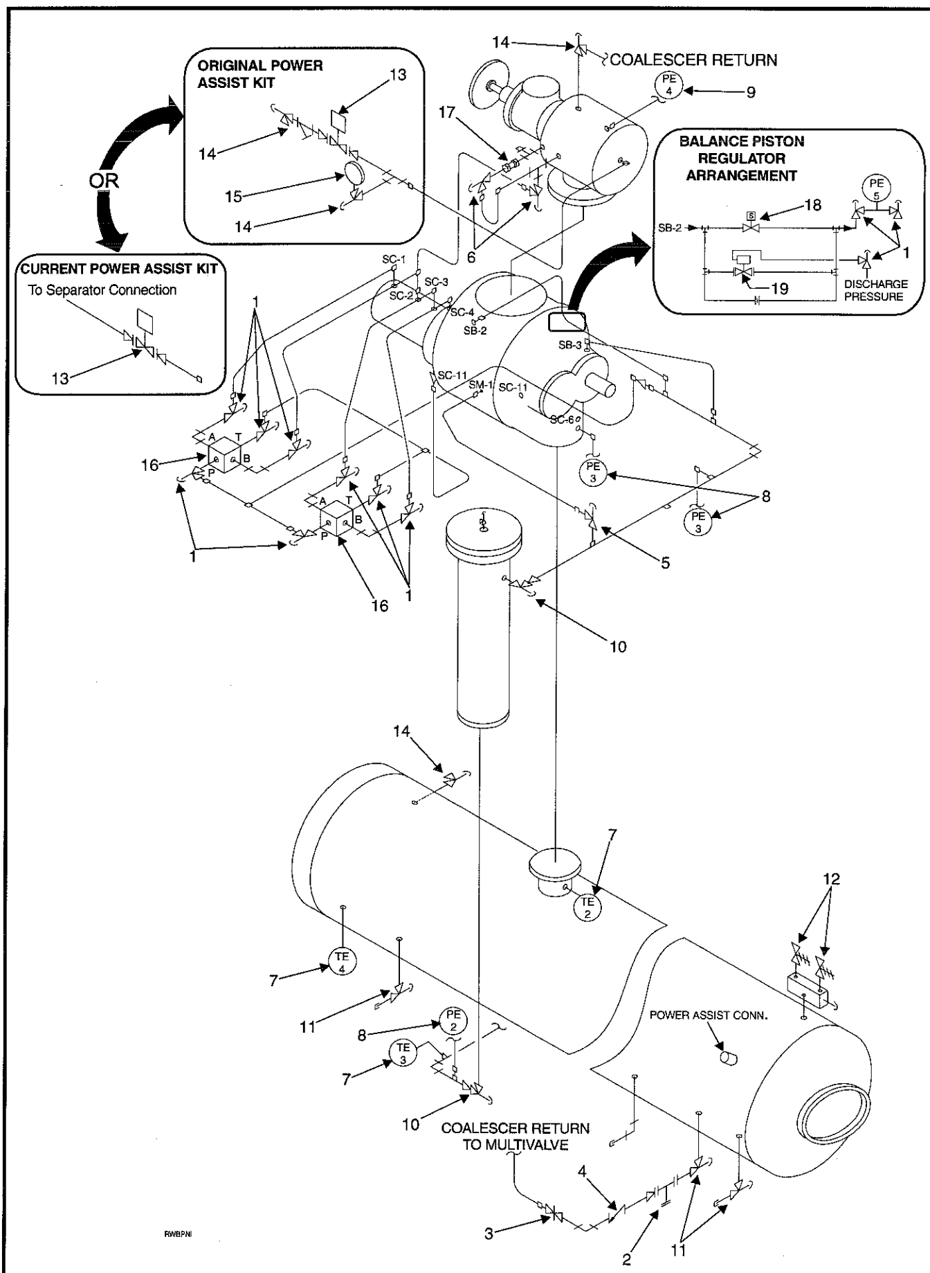
Figure 6. Piping and Instrumentation, Typical.
