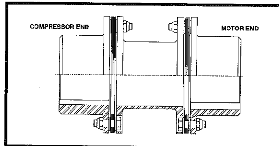
Figure 22. Drive Coupling, Models 496 and 676.
