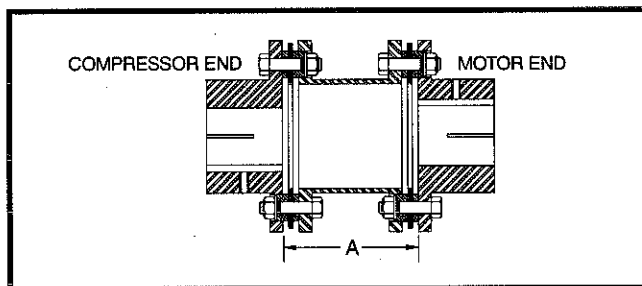
FIGURE 24. Drive Coupling, Model 856. COUPLING ASSEMBLIES-FIGURE 24.
