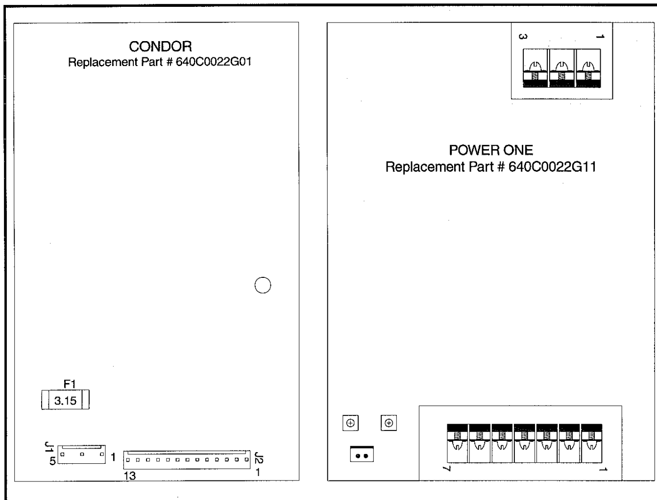
Figure 29. Quantum power supply identification.
