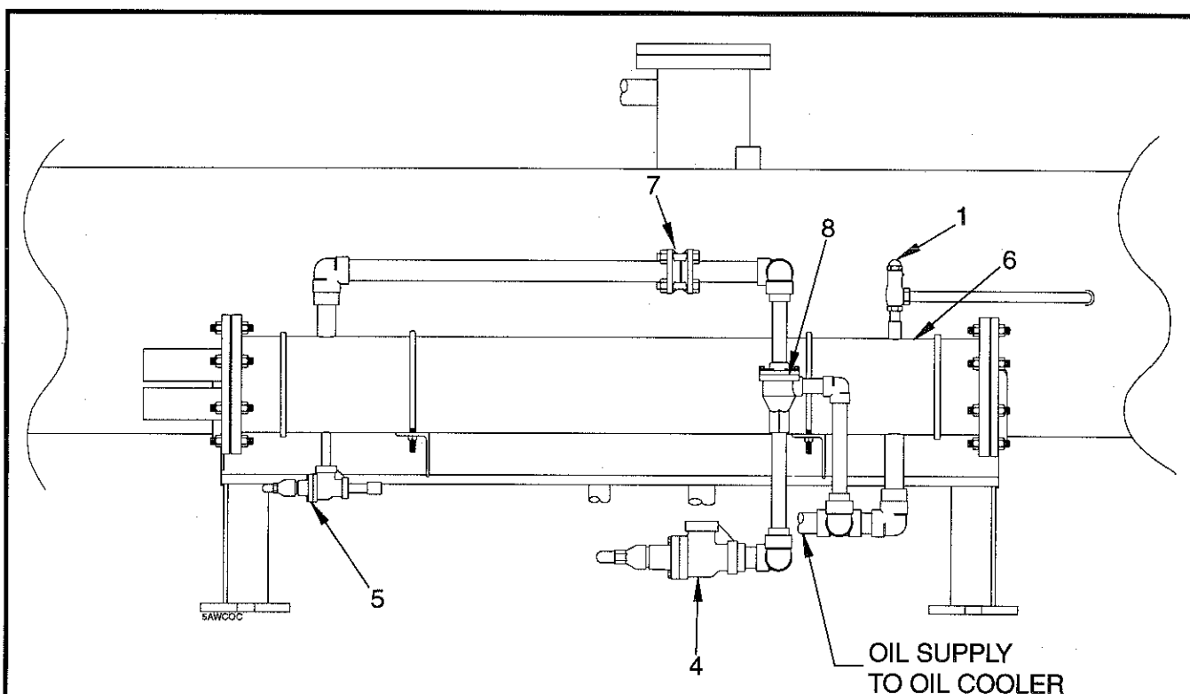
Figure 8a. Oil Cooler Piping With Oil Temperature Regulating Valve.
