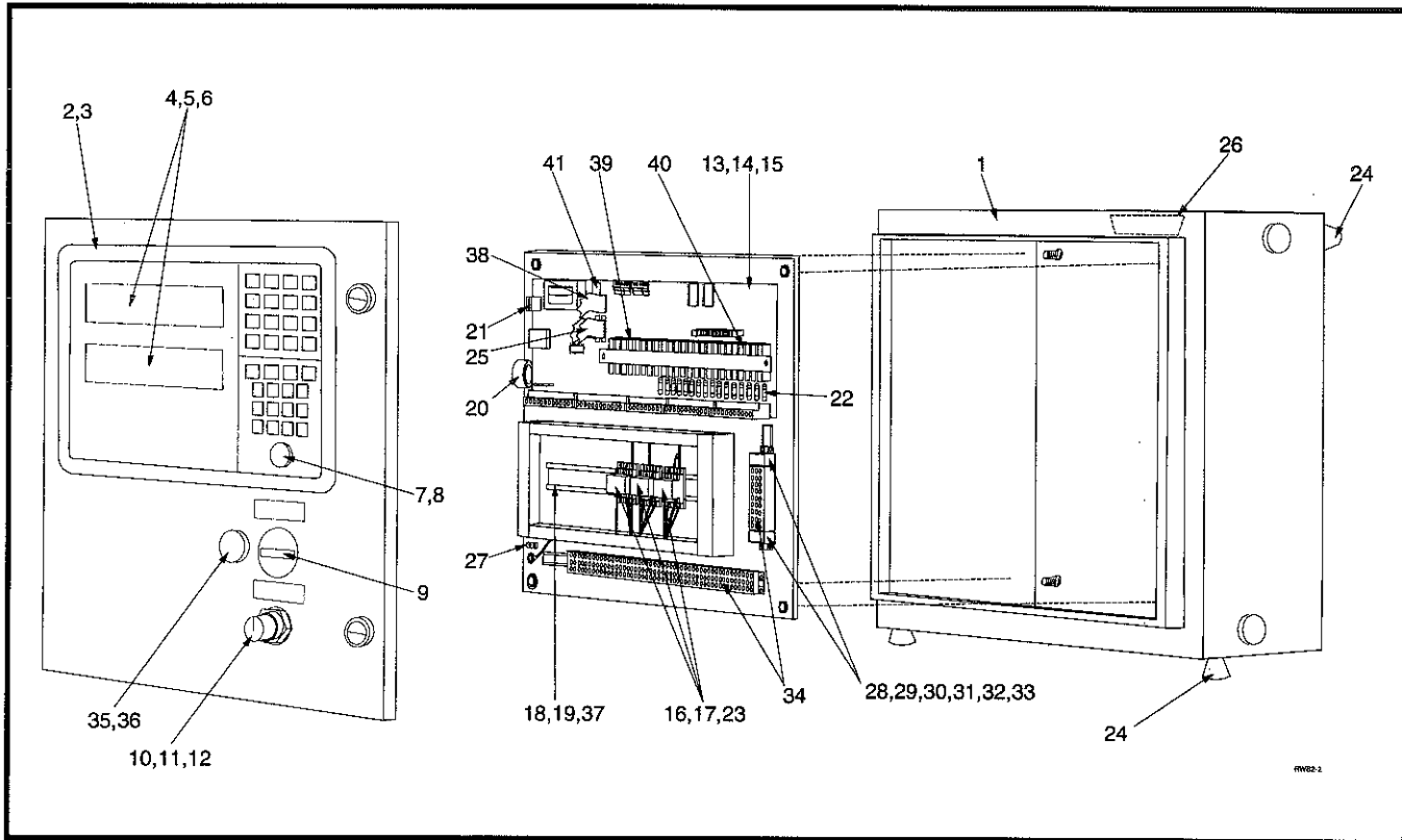
Figure 25. Microprocessor Control Center (Single Box).
