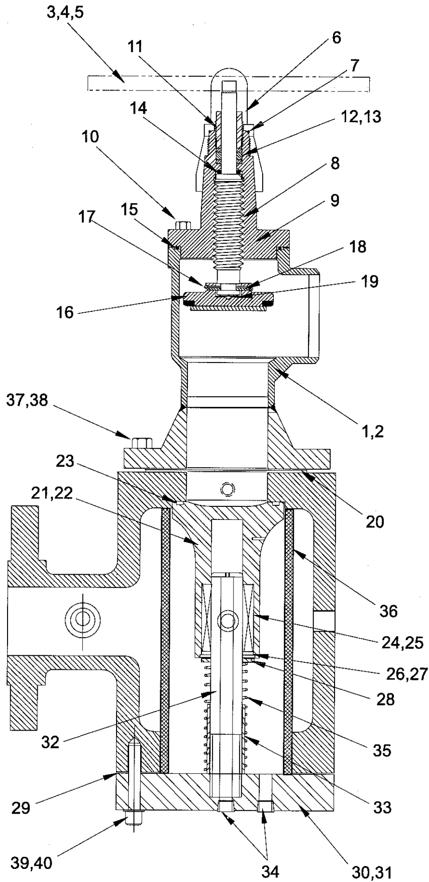
Figure 11. 4" Multivalve
