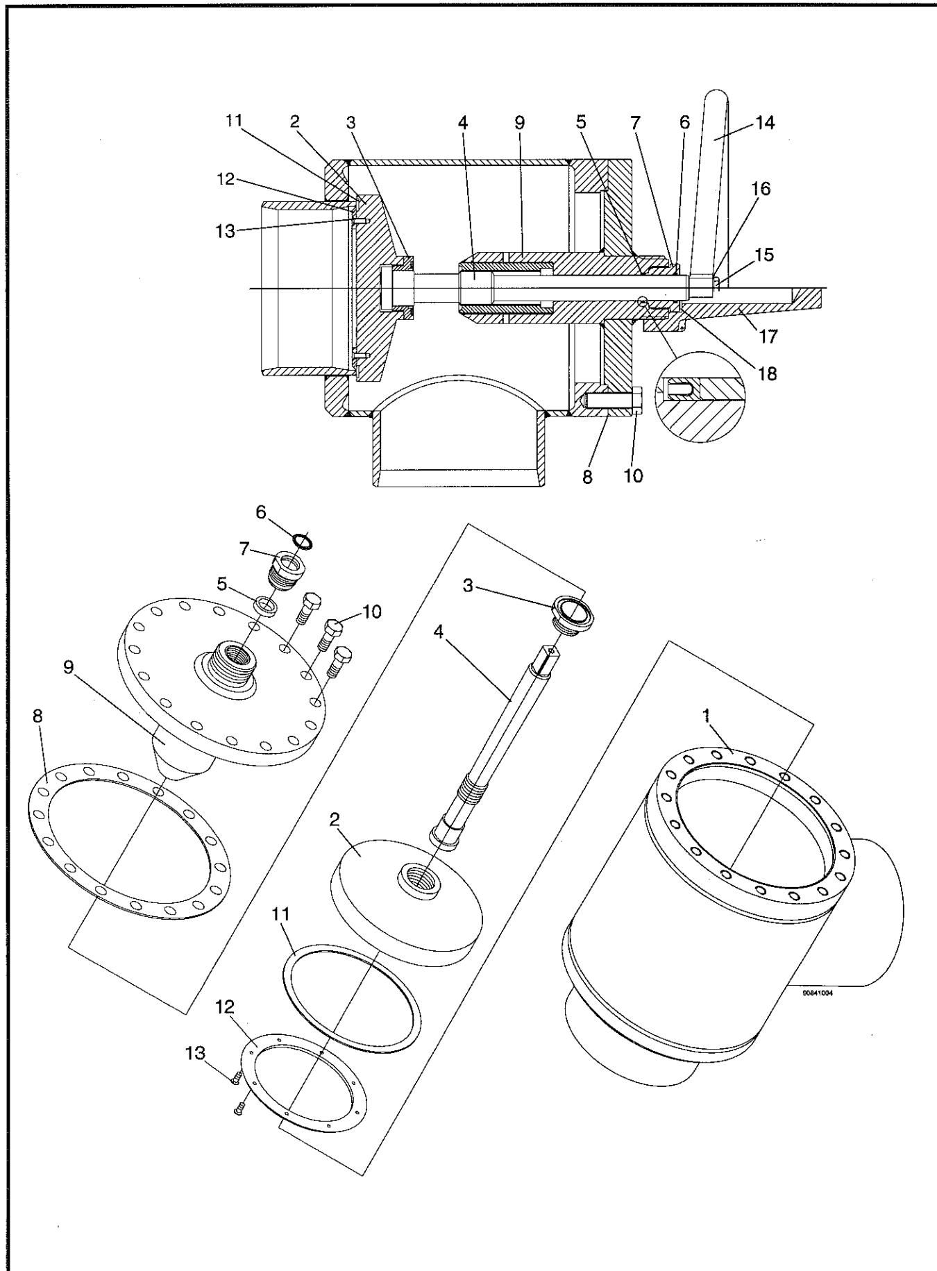
Figure 17. 8" Discharge Stop Valve Assembly (Gram).
