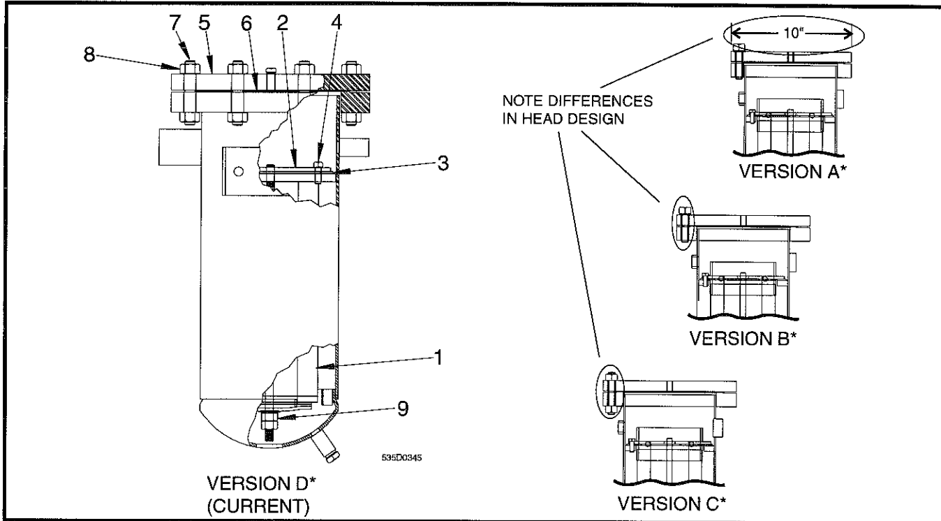
Figure 4. Oil Filter, Standard, Typical (Single Element Shown).
