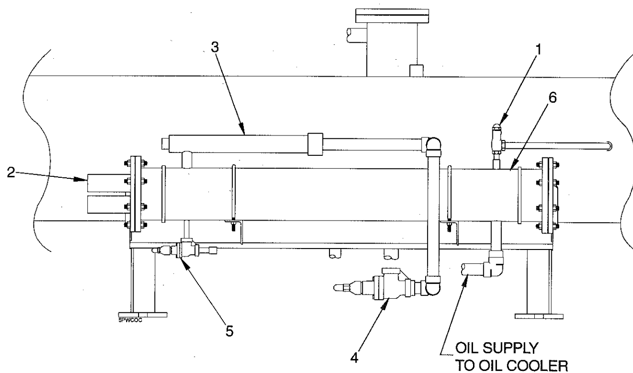
Figure 8b. Oil Cooler Piping With Water Flow Regulating Valve.
