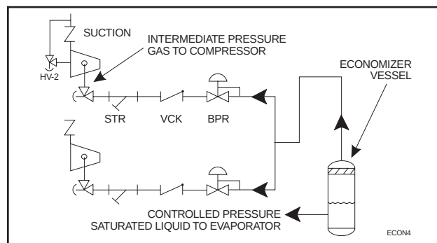
FIG. 4 - MULTIPLE COMPRESSOR ECONOMIZER SYSTEM
