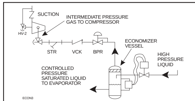
FIG. 3 - FLASH ECONOMIZER SYSTEM
