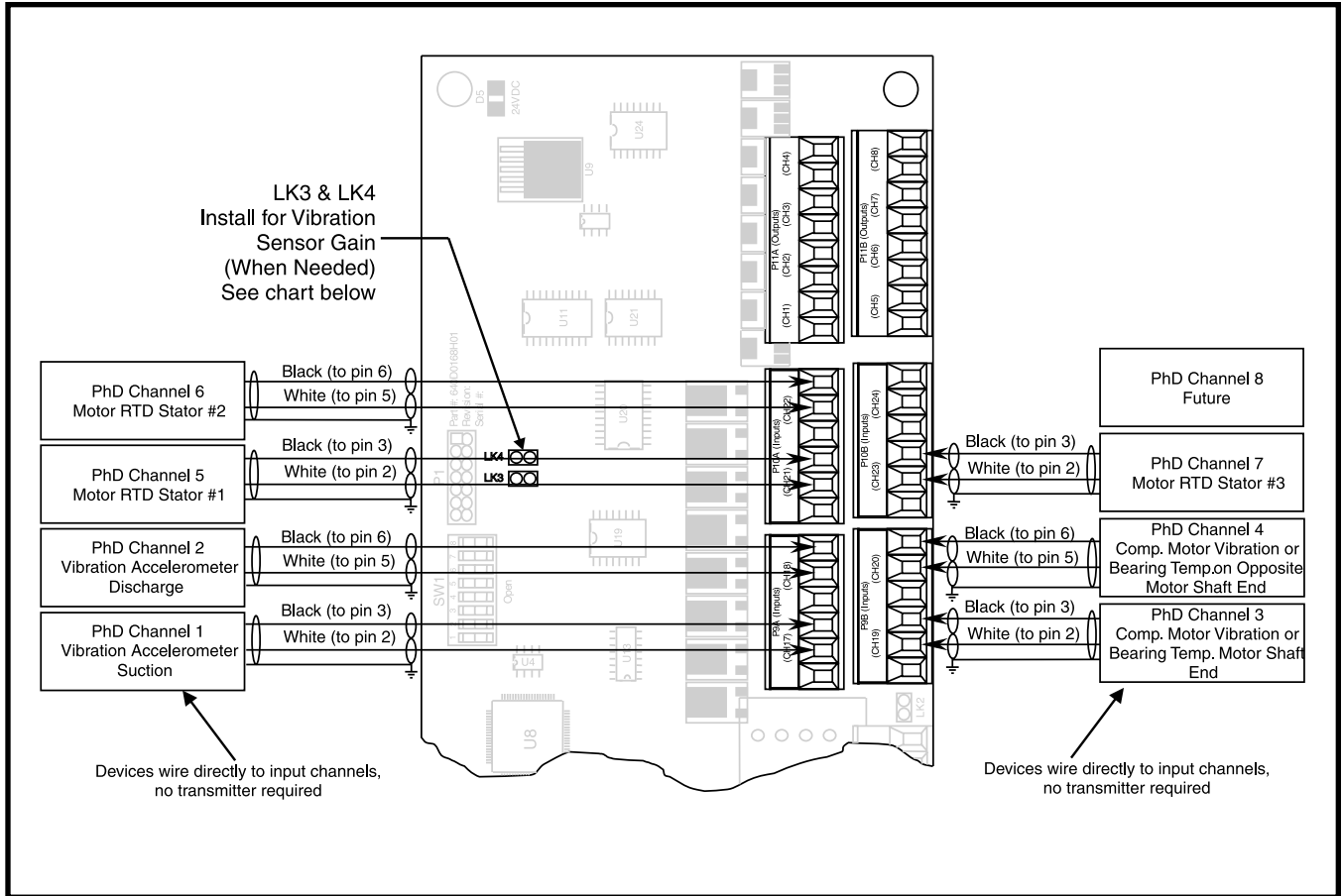
Figure 10 - PhD Wiring Connections
