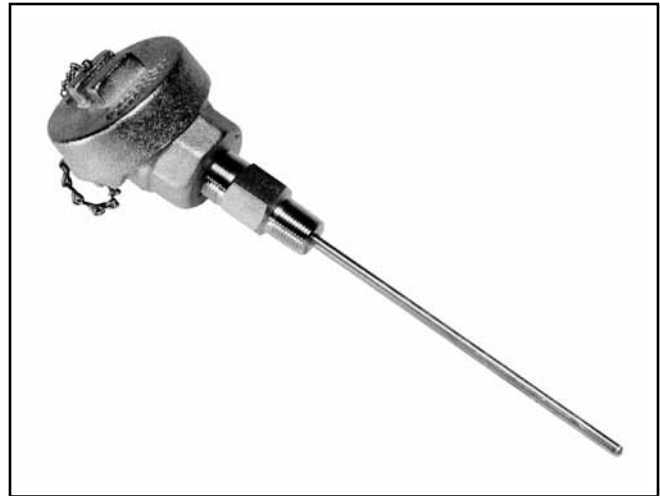
Figure 9 - Motor Bearing RTD Temperature Sensor
