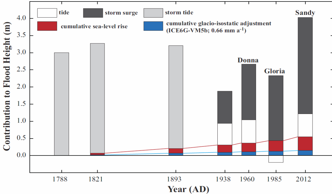
Estimated Contribution to Flood Heights in New York City for Notable Historical Hurricanes 186
