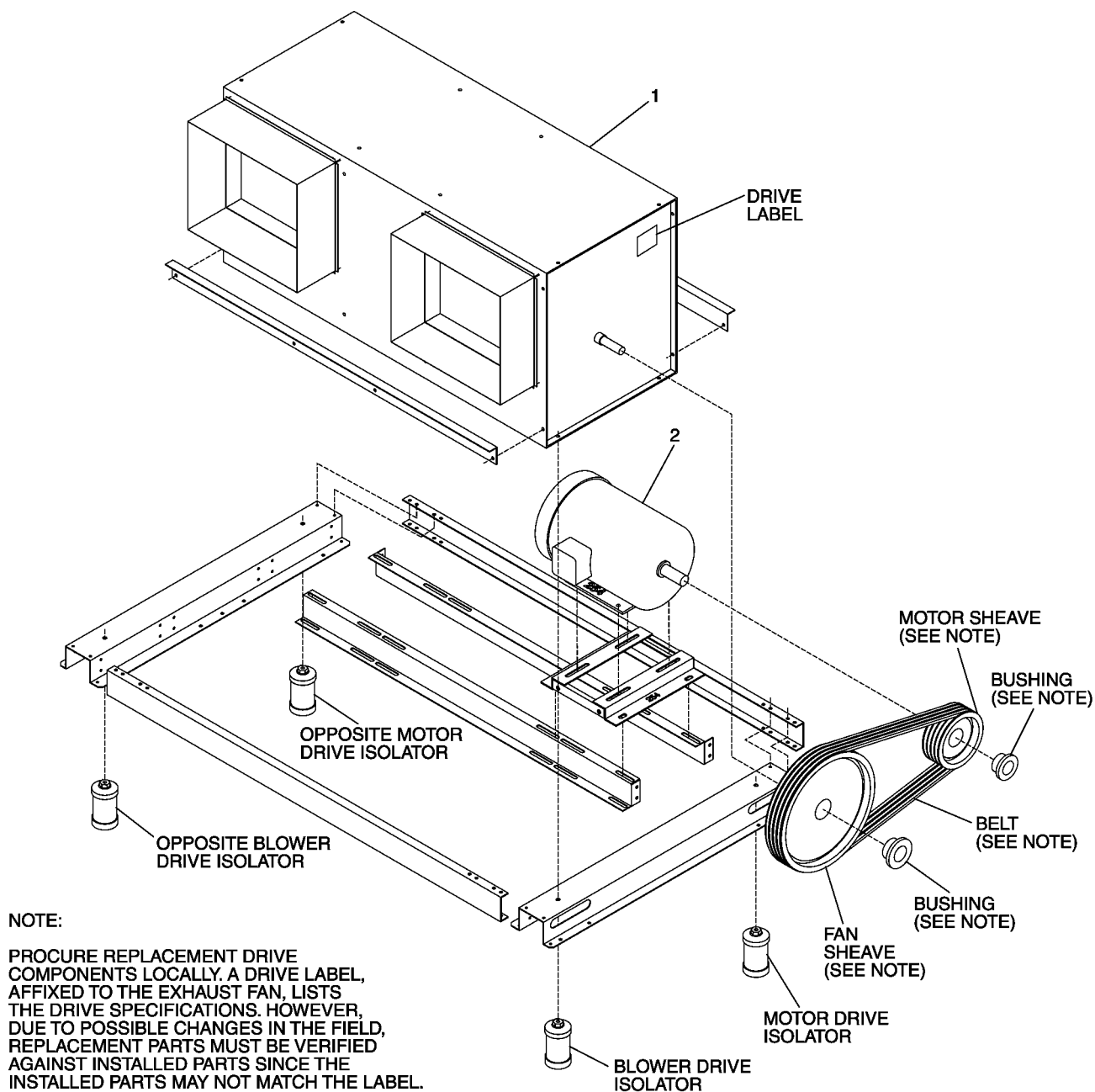
FIGURE 13 - EXHAUST FANS, MOTORS, ISOLATORS, AND DRIVE COMPONENTS
