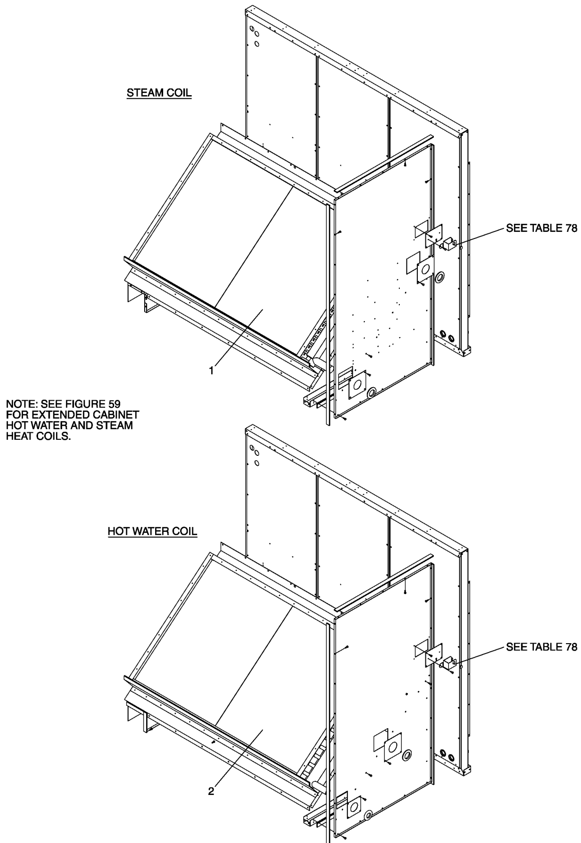
FIGURE 44 - HOT WATER AND STEAM HEAT COILS (STANDARD CABINET)
