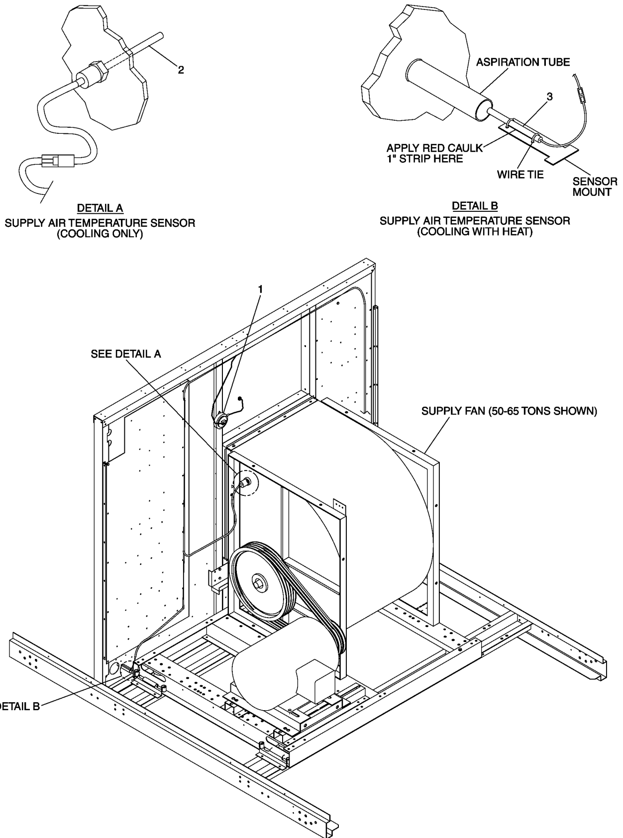
FIGURE 82 - AIR PROVING SWITCH AND SUPPLY AIR TEMPERATURE SENSOR
