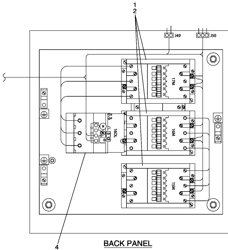
FIGURE 35 - VFD BYPASS BOX REPLACEMENT PARTS (60-110 MOTOR FLA)
