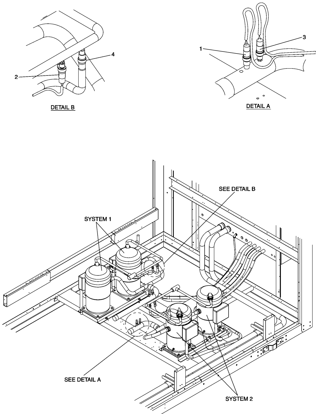
FIGURE 78 - SUCTION AND DISCHARGE PRESSURE TRANSDUCERS AND SAFETY SWITCHES (50-65 TONS)
