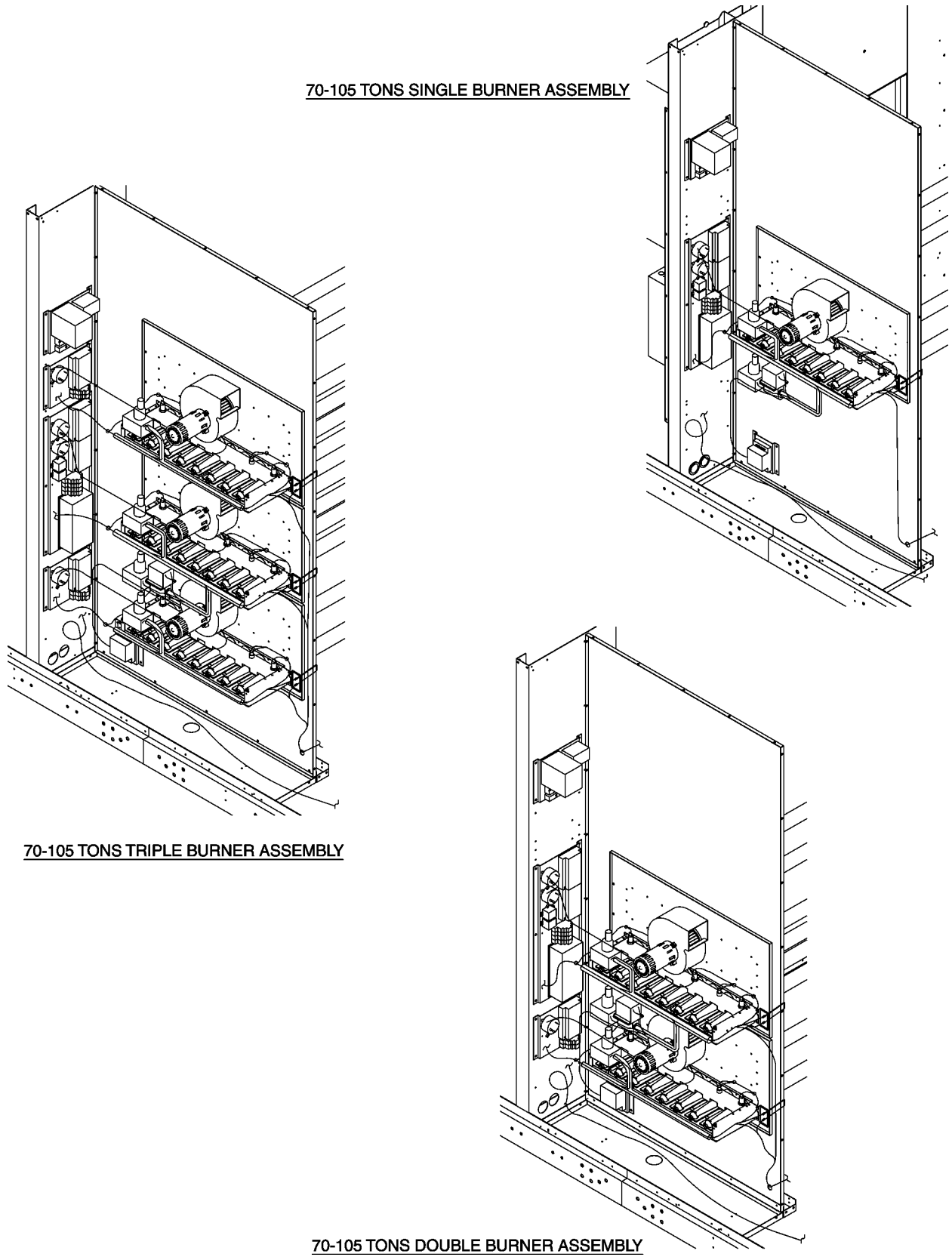
FIGURE 42 - MODULATING GAS HEAT ARRANGEMENTS (70-105 TONS)
