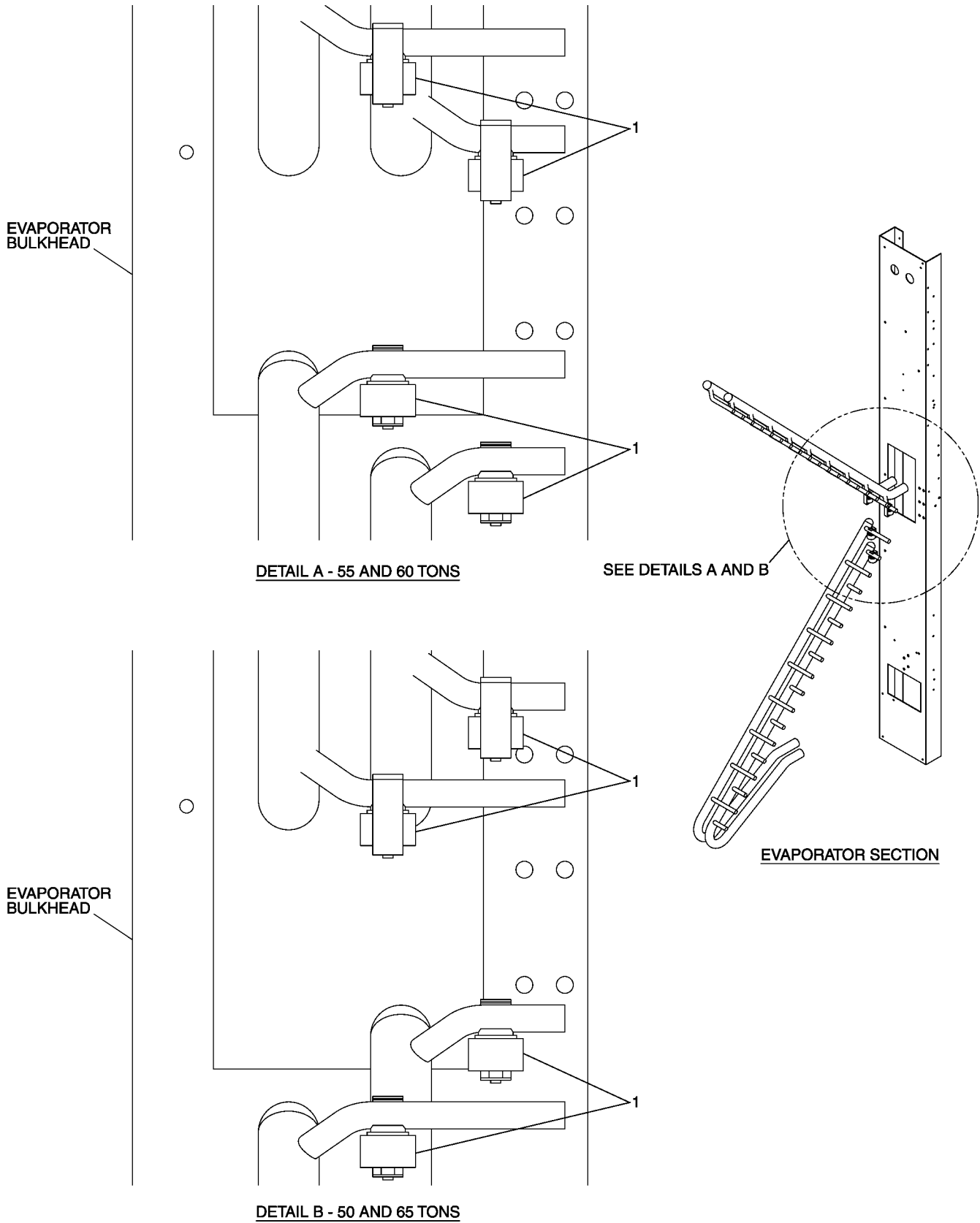
FIGURE 83 - EVAPORATOR TEMPERATURE SENSOR (50-65 TONS)
