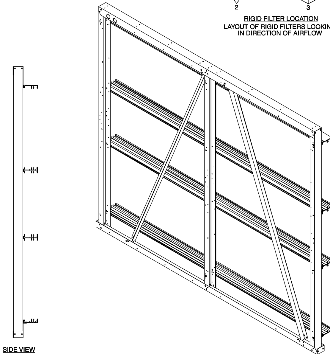
FIGURE 21 - RIGID UNIT FILTERS (50-65 TONS)
