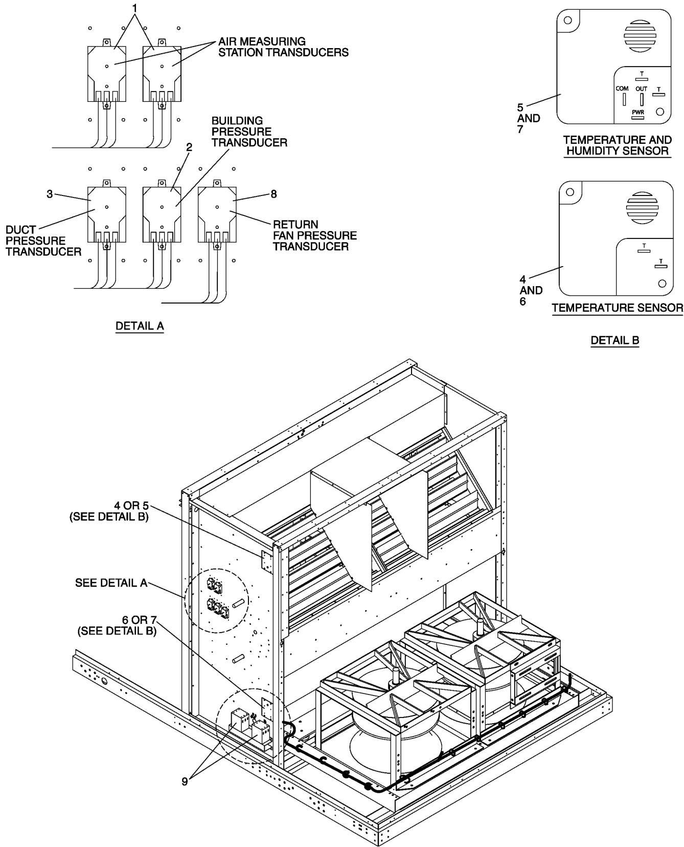
FIGURE 87 - ECONOMIZER SECTION TRANSDUCERS AND SENSORS
