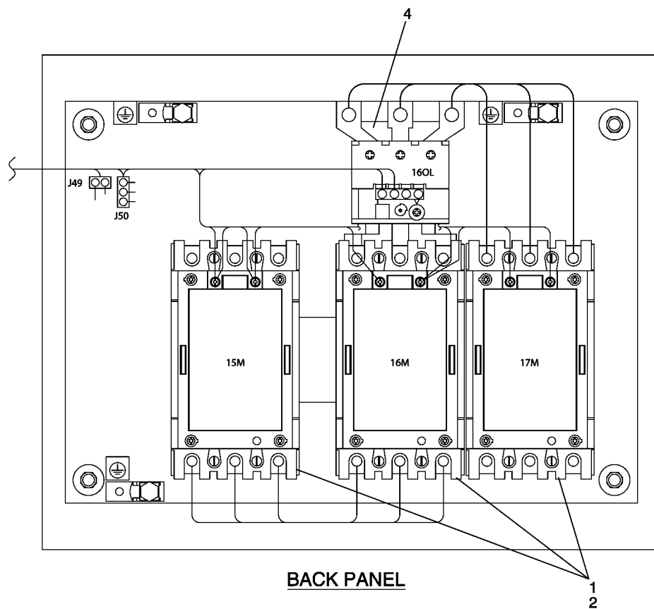
FIGURE 36 - VFD BYPASS BOX REPLACEMENT PARTS (110-200 MOTOR FLA)
