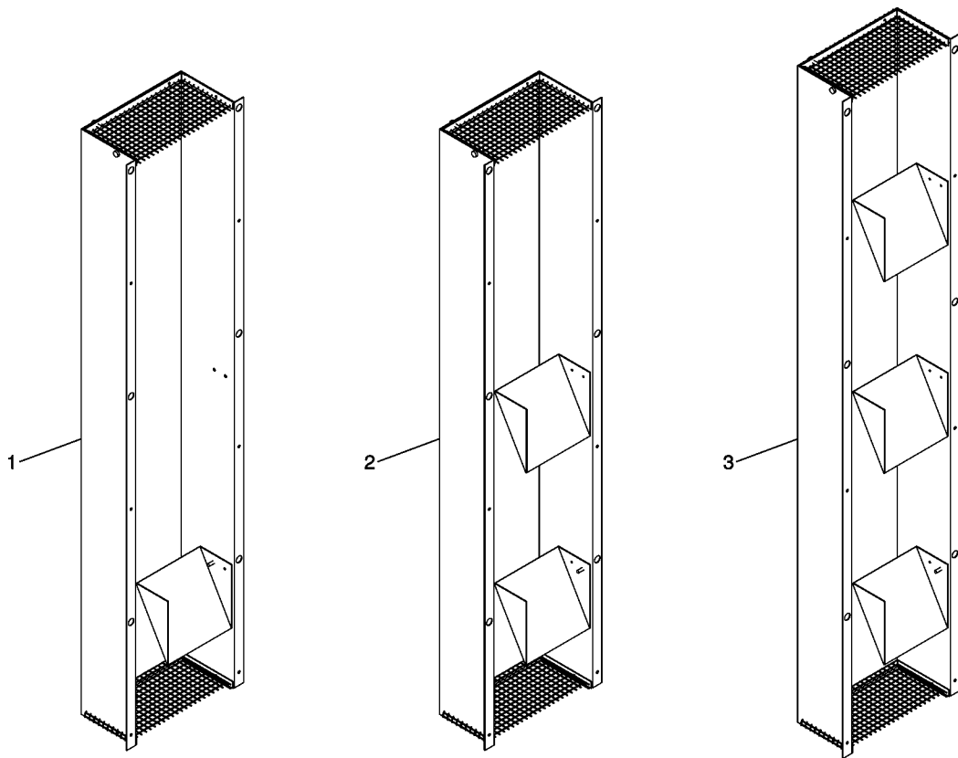
FIGURE 11 - CHIMNEY ASSEMBLIES
