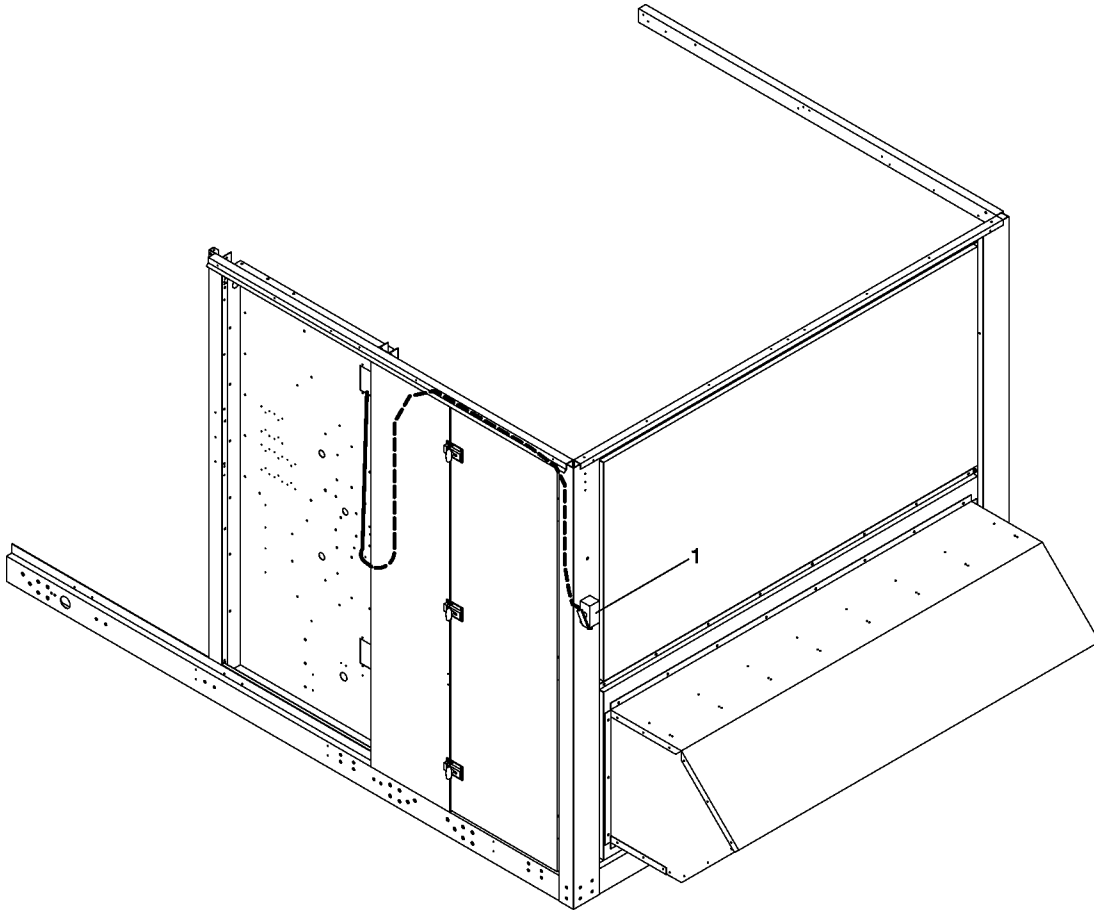
FIGURE 88 - OUTSIDE AIR TEMPERATURE SENSOR (EXTERNAL)
