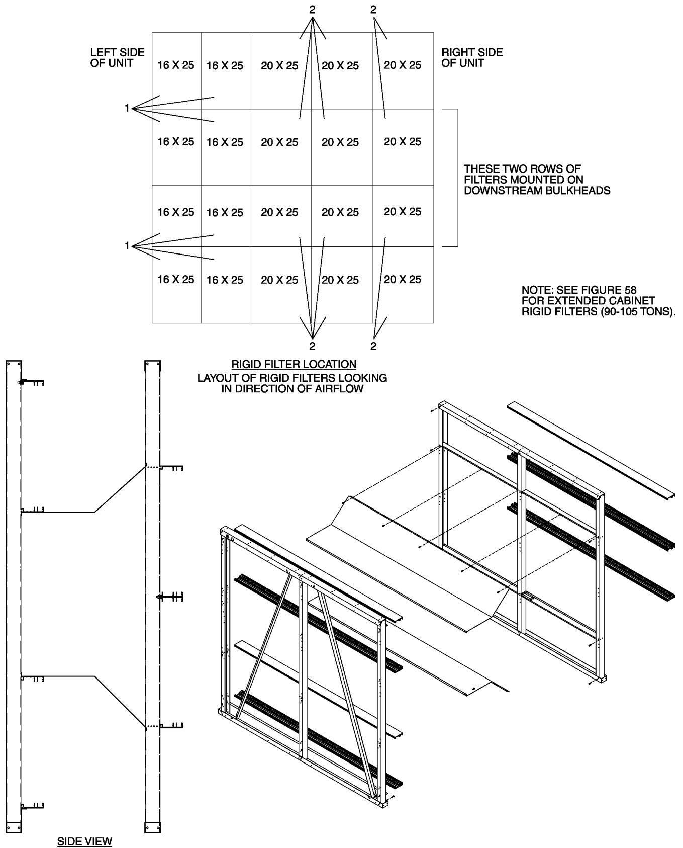
FIGURE 23 - RIGID UNIT FILTERS (90-105 TONS)
