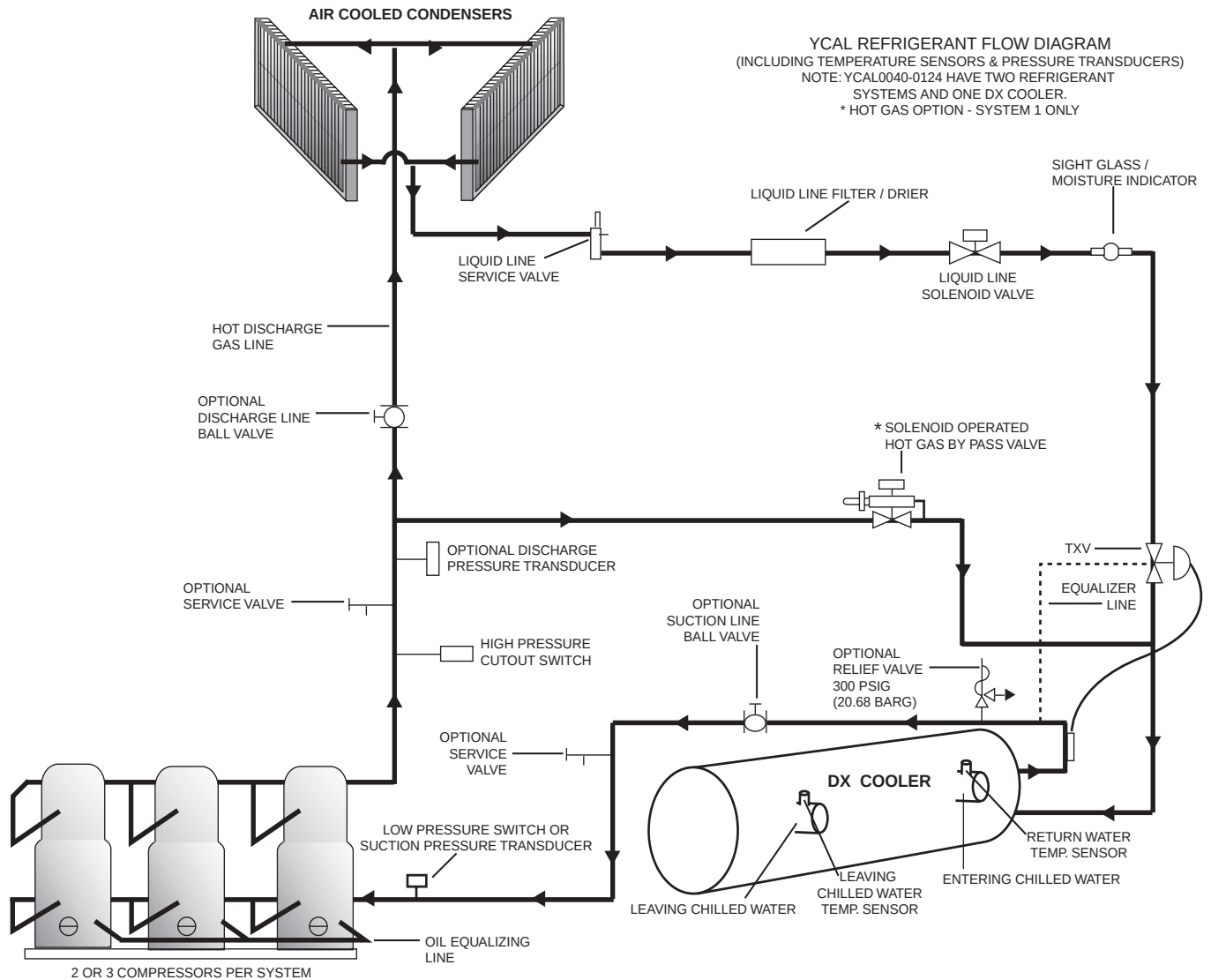
FIG. 1 – REFRIGERANT FLOW DIAGRAM
