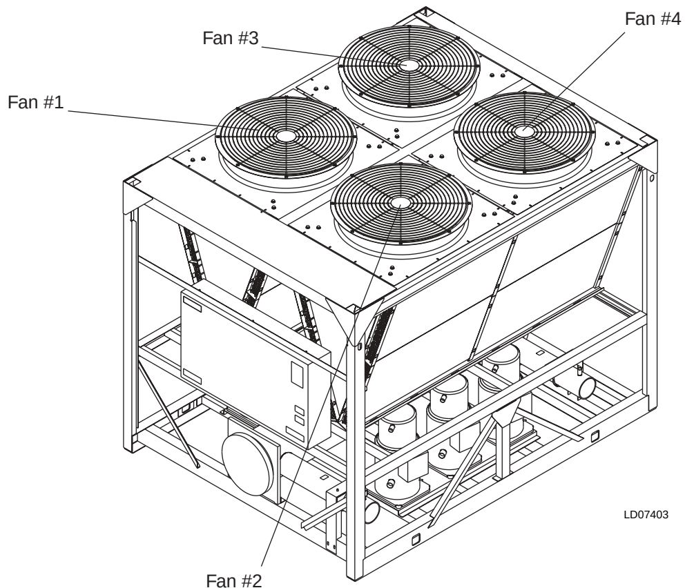
FIG. 9 – DYCAL0010 – 0040 FAN LOCATION (TYPICAL)
