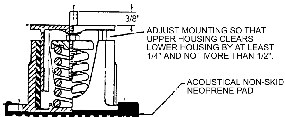
FIG. 37 – TYPE CP MOUNTING
