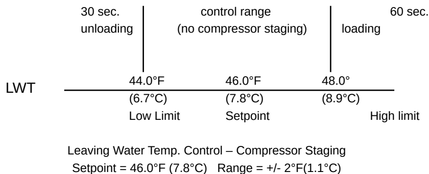
FIG. 8 – LEAVING WATER TEMPERATURE CONTROL EXAMPLE
