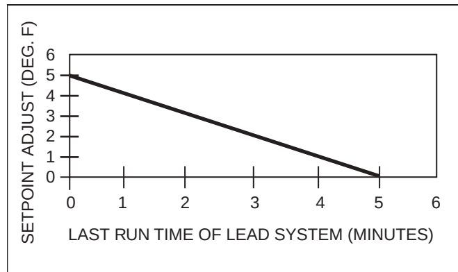
FIG. 7 – SETPOINT ADJUST
