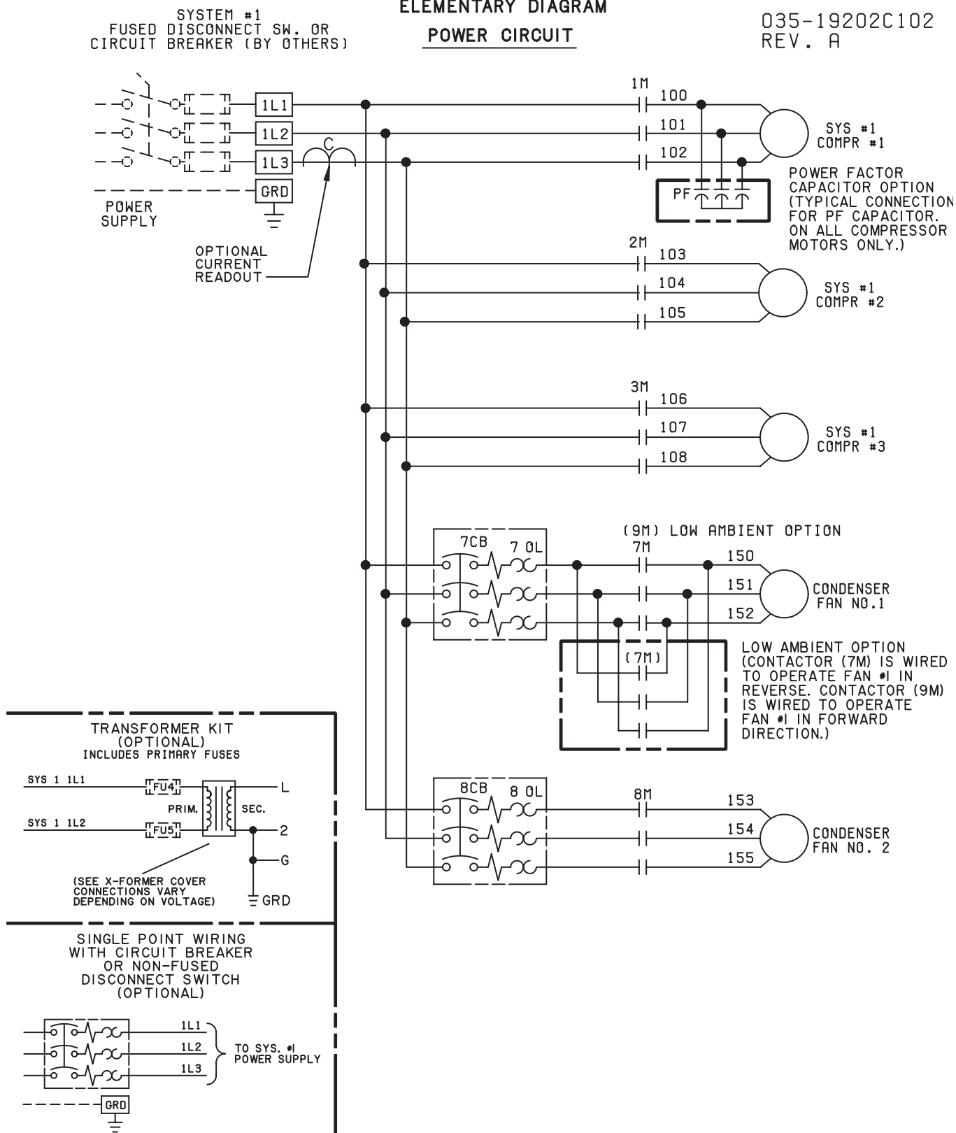
FIG. 21 – ELEMENTARY DIAGRAM, POWER CIRCUIT – DYCAL0035, 40, &amp; 50
