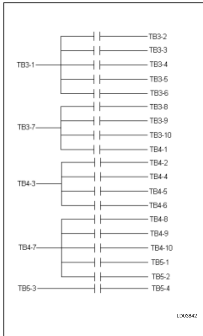
FIG. 14 – MICROBOARD RELAY CONTACT ARCHITECTURE
