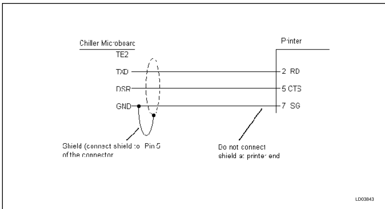
FIG. 15 – PRINTER TO MICROBOARD ELECTRICAL CONNECTIONS
