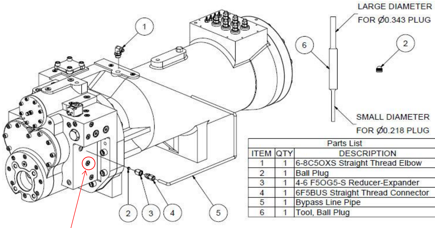
FIGURE 2 - BYPASS LINE ASSEMBLY
