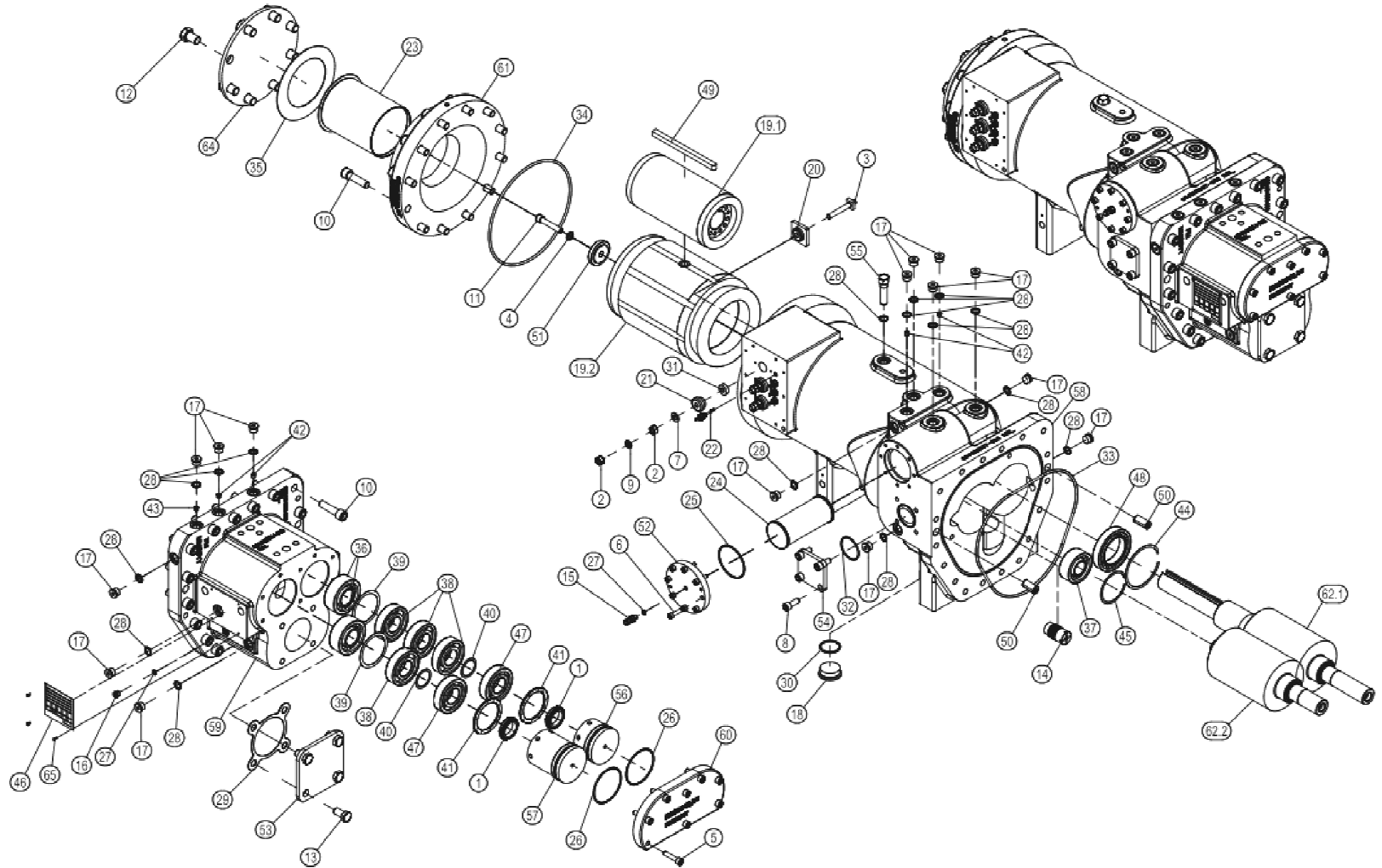
图 2 CTS136 Standard/HP 螺杆压缩机总图 Figure 2 CTS136 Standard/HP Screw Compressor General Arrangement
