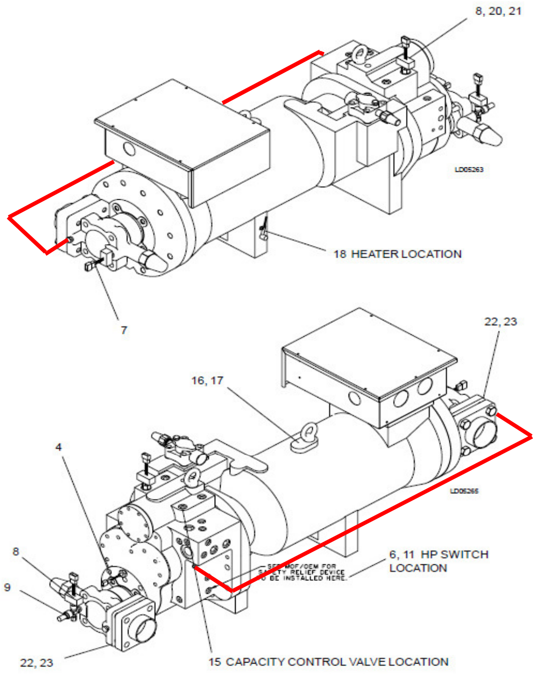
FIG. 12 – DXS COMPRESSOR OUTLINE (REF. TABLES 8 AND 9, PAGE 25)
