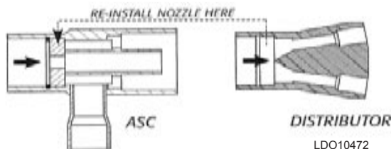
FIG. 24 – ASC/NOZZLE LOCATION
