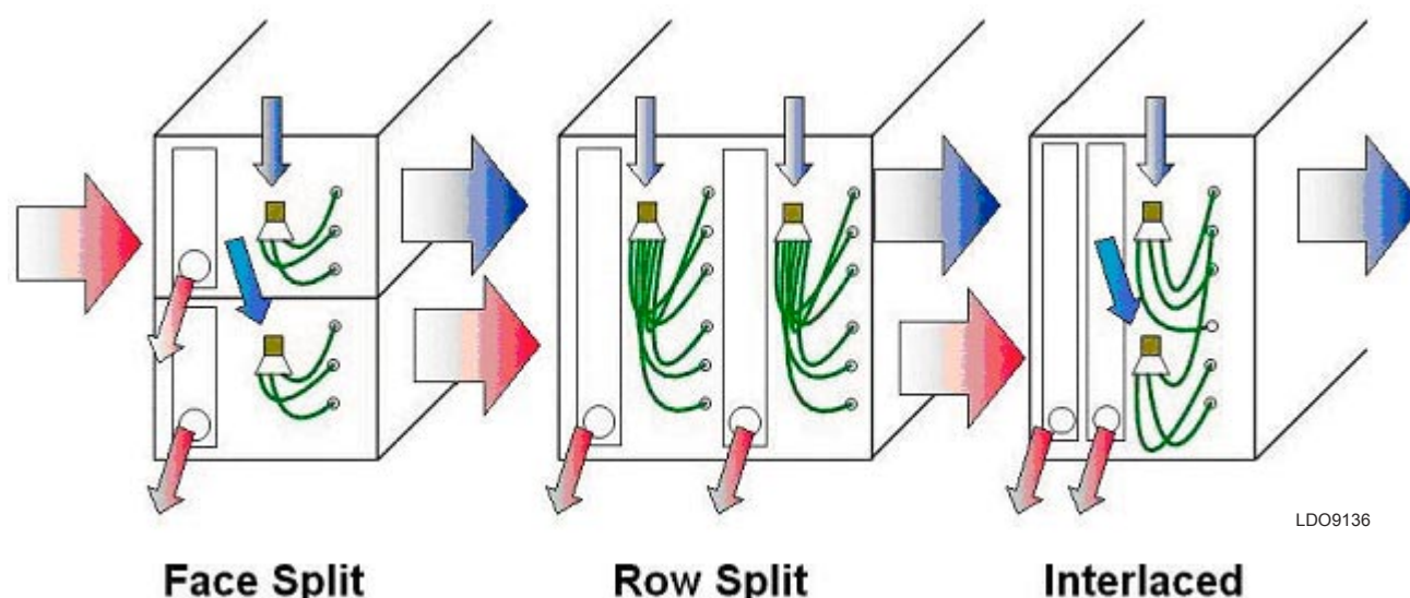
FIG. 18 – EVAPORATOR COIL TYPES
