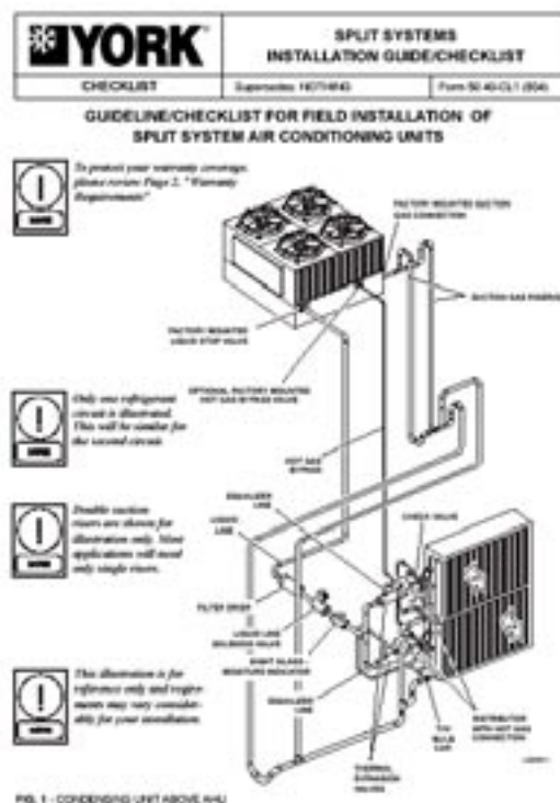
FIG. 1 - CONDENSING UNIT ABOVE A/CU
