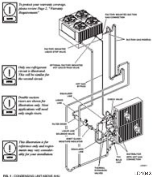
FIG. 1 - CONDENSING UNIT ABOVE A/CU
