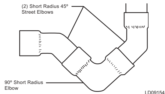
FIG. 7 –OIL TRAP PIPING
