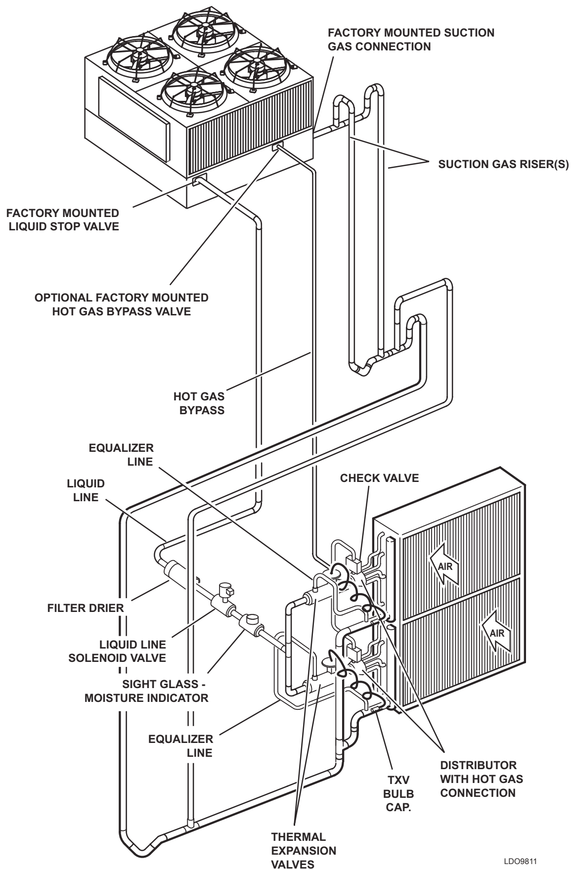
FIG. 30 – REFERENCE DRAWING - FIELD-PIPING LAYOUT (ACCU ABOVE EVAPORATOR)
