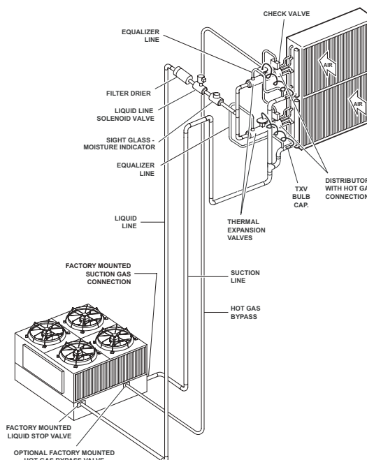
FIG. 4 - YCUL BELOW EVAPORATOR COIL
