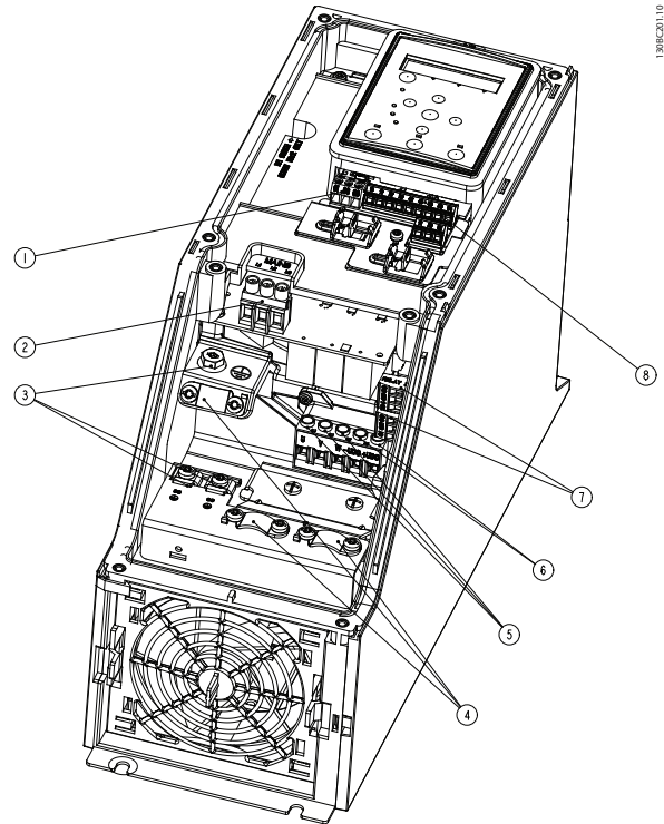
Figure 1.14 I3 Frame IP54 380-480 V 75-100 hp [5.5-7.5 kW]
