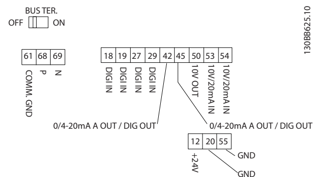
Figure 1.25 Control Terminals
