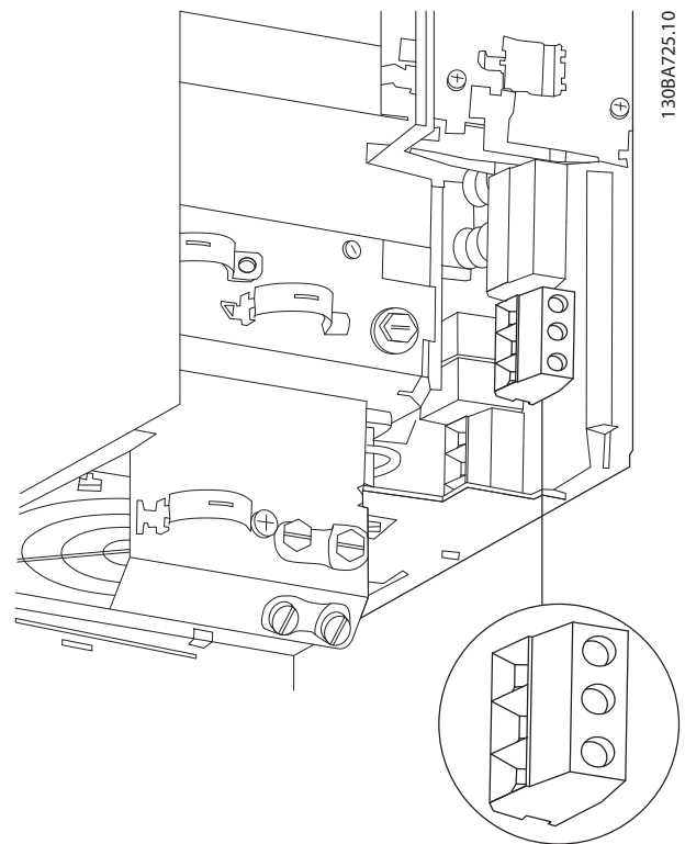
Figure 1.12 H10 Frame IP20 600 V 15-20 hp [11-15 kW]
