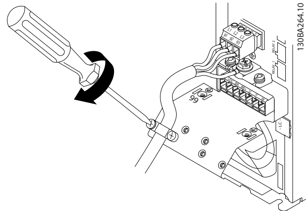
Figure 1.11 Tighten support bracket on the line power wires
