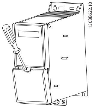
Figure 1.22 Location of Control Terminals
