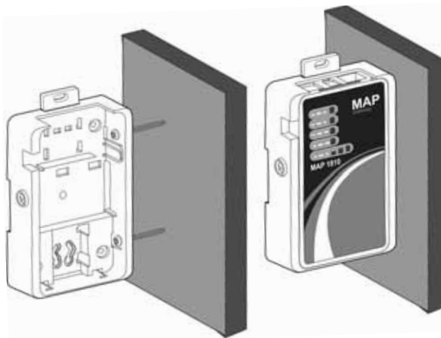
Figure 7: Sample Permanent Mounting, Side Screws
