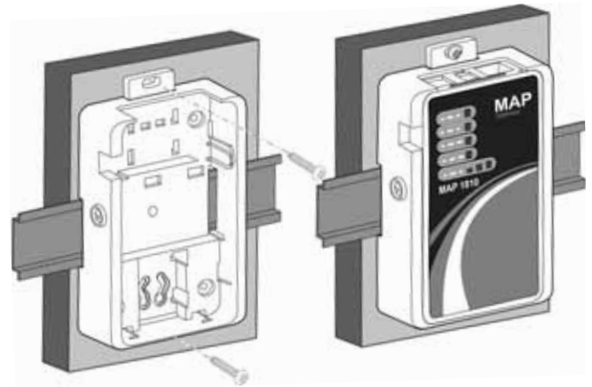
Figure 8: Sample Permanent Mounting, DIN Rail Screw Holes
