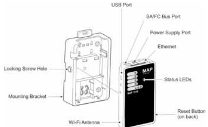
Figure 1: MAP Gateway Features (Portable Unit)
