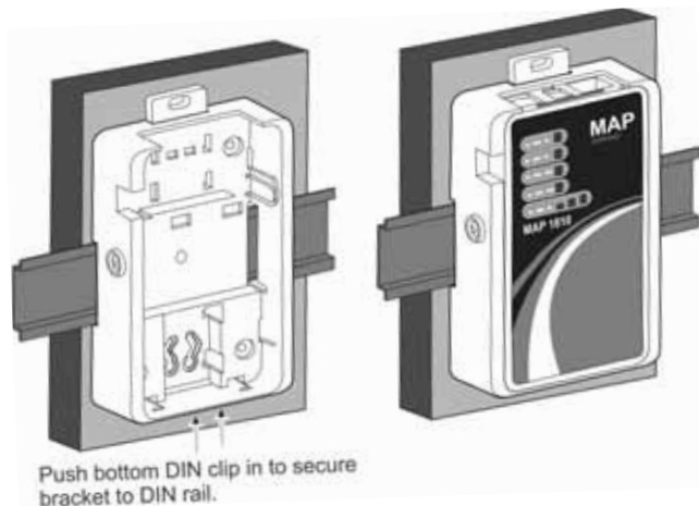
Figure 5: Positioning the Bracket on a DIN Rail
