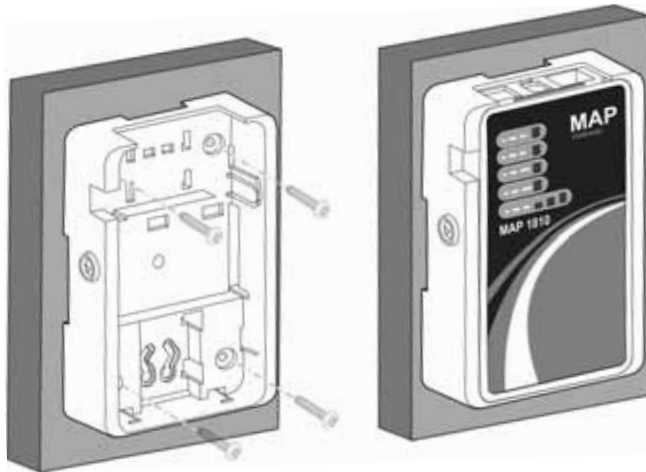
Figure 6: Sample Permanent Mounting, Back-side Screws
