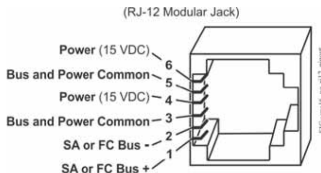
Figure 12: SA/FC Port Pin
