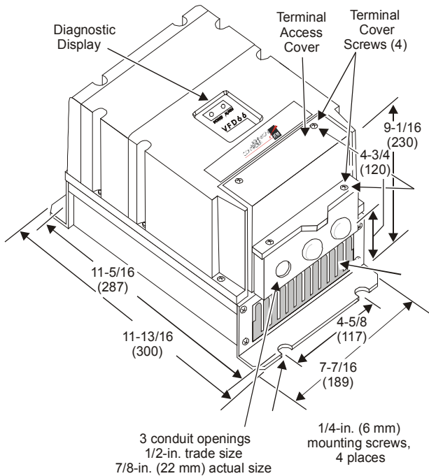
Figure 4: Large VFD66 NEMA 4 Enclosure Dimensions
