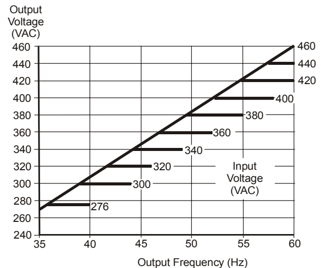
Figure 18: Output Voltage and Frequency vs. Input Power, 400/460 VAC
