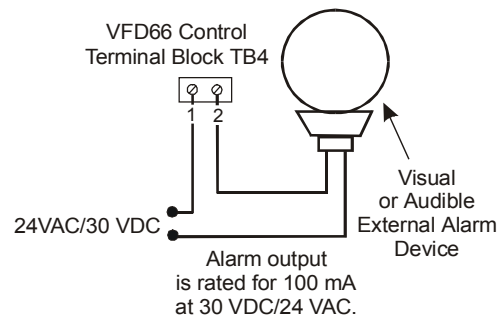
Figure 9: Wiring the Alarm Output
