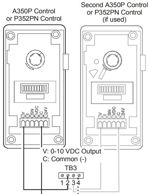
Figure 8: Wiring A350P Controls or P352PN Controls to VFD66 Terminal Block 3
