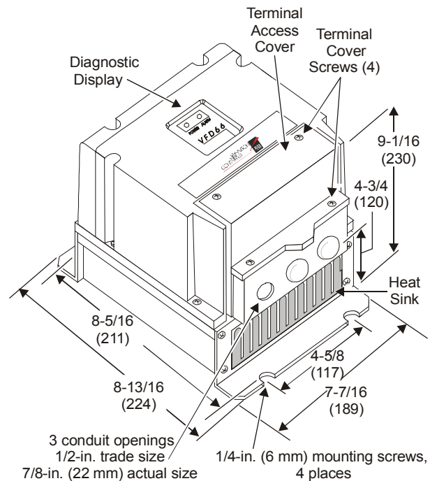
Figure 3: Small VFD66 NEMA 4 Enclosure Dimensions
