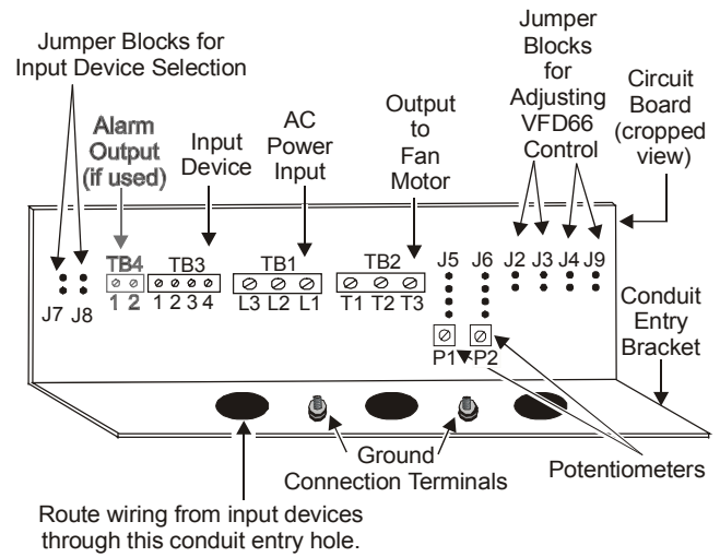
Figure 5: Jumper Block, Terminal Block, and Potentiometer Locations
