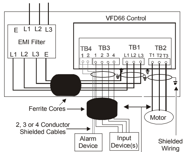
Figure 10: CE/FCC/DOC Compliance Wiring
