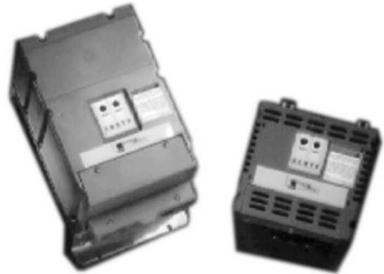
Figure 1: VFD66 Condenser Fan Speed Control, NEMA 4 and NEMA 1 Enclosures
