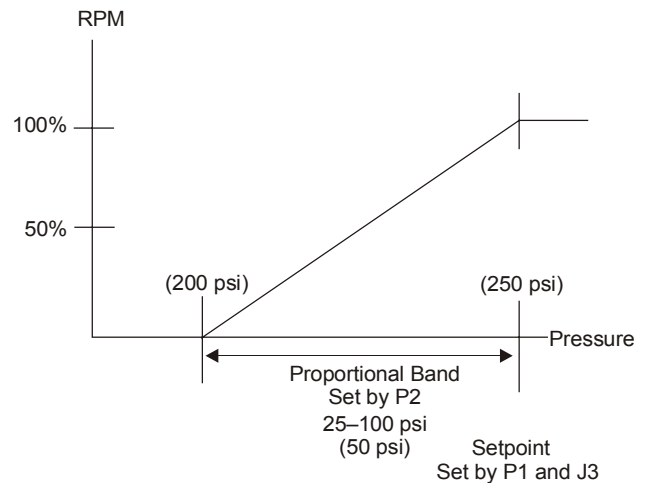
Figure 15: Electronic Pressure Transducer Input Mode, 0-500 psi P399 Transducer
