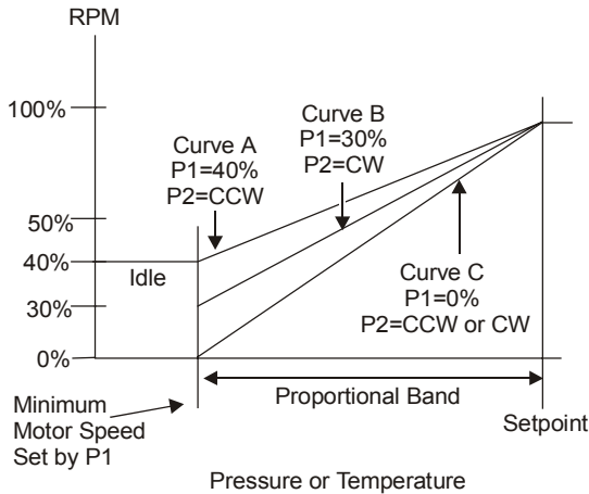
Figure 14: Standard Input Mode
