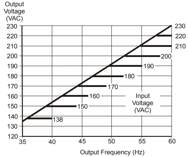
Figure 17: Output Voltage and Frequency vs. Input Power, 208/230 VAC
