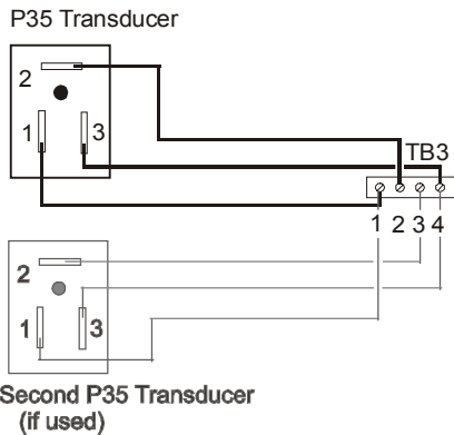
Figure 6: Wiring P35 Transducers to VFD66 Terminal Block 3
