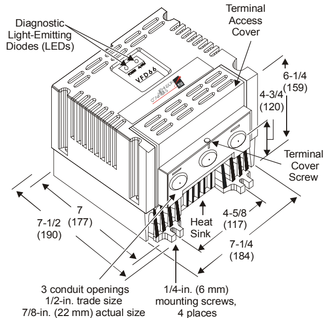
Figure 2: VFD66 NEMA 1 Enclosure Dimensions
