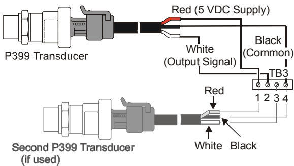
Figure 7: Wiring P399 Transducers to VFD66 Terminal Block 3
