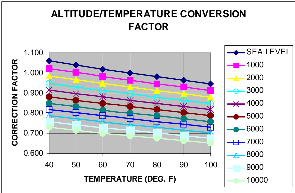
FIGURE 21 - ALTITUDE/TEMPERATURE CONVERSION FACTOR
