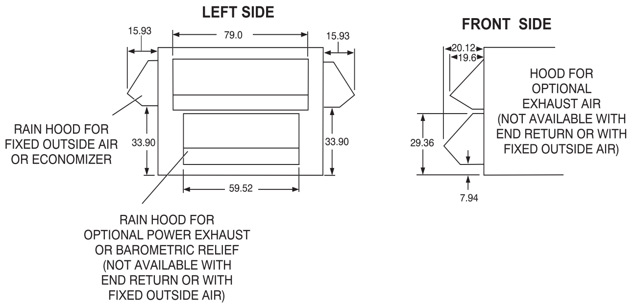
FIGURE 36 - CLEARANCES - HOOD/ECONOMIZER & MOTOR DRIVE - FRONT & END
