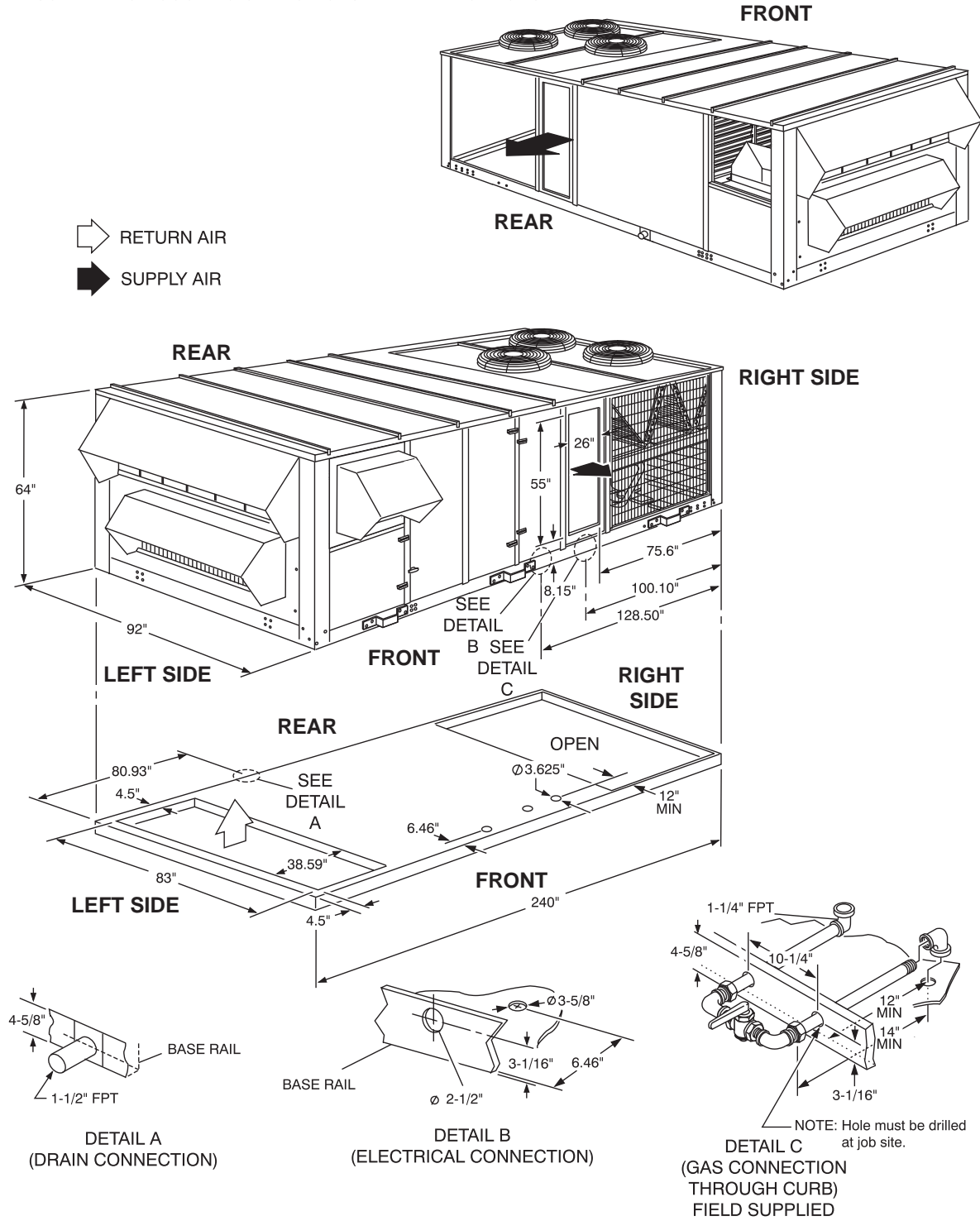
FIGURE 31 - BOTTOM RETURN, FRONT & REAR SUPPLY
