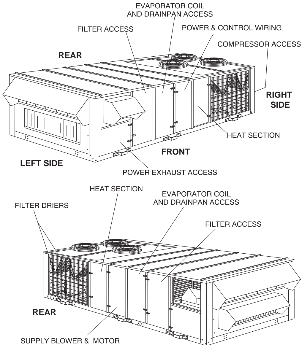
FIGURE 28 - COMPONENT LOCATION
