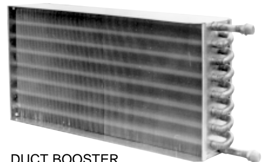
DUCT BOOSTER
