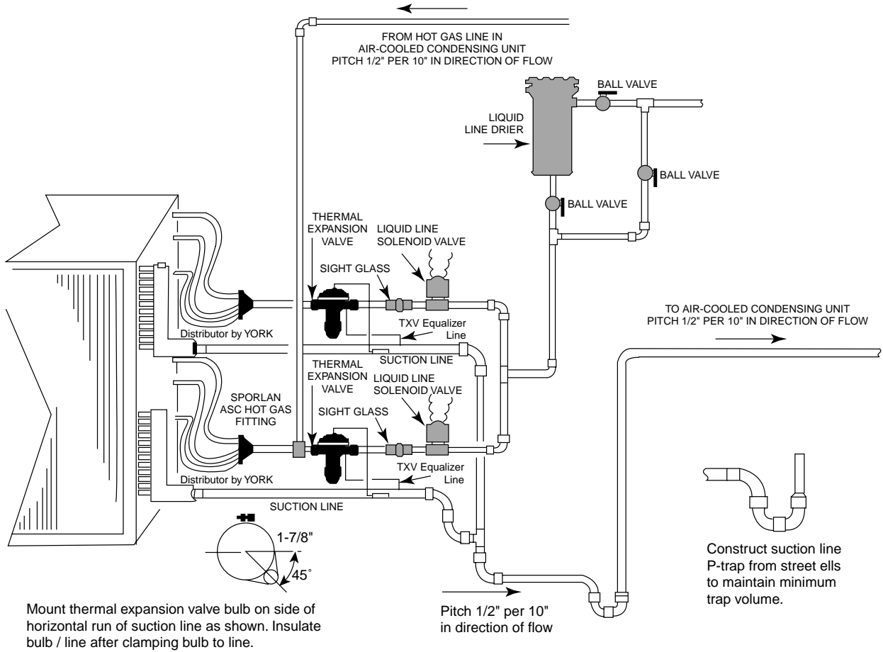
FIG. 3 – PIPING ARRANGEMENTS
